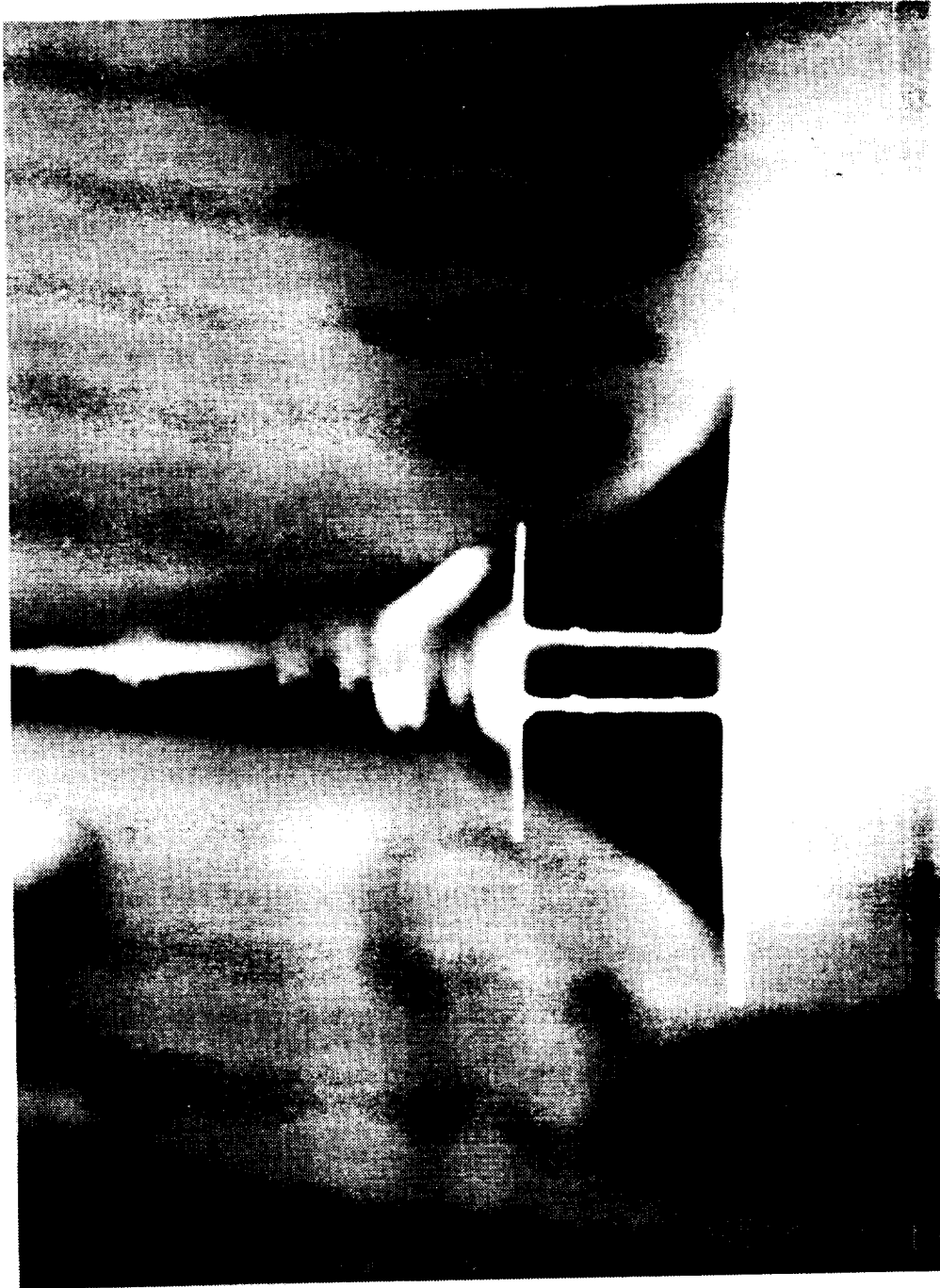
Figure 27. Second free-free out-of-plane mode of the I-specimen: The cross-sectional motion shown in the photograph is purely lateral. Thus, the I-section decouples in-plane and out-of-plane response.
