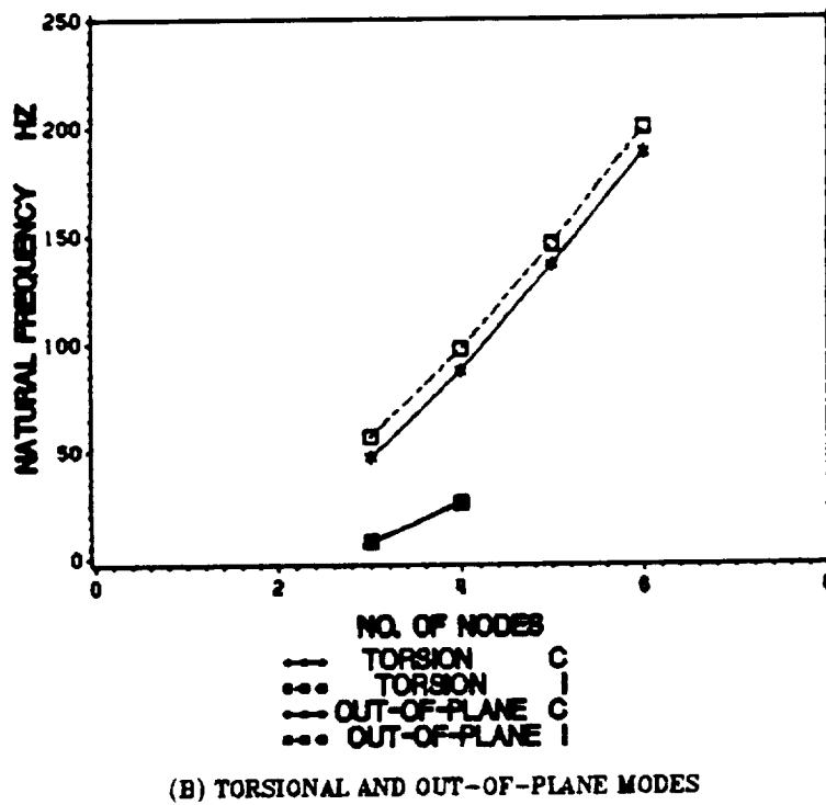
Figure 29. Comparison of free-free natural frequencies: The in-plane and out-of-plane natural frequencies for both test specimens are shown in the two plots. The number of nodes in a mode is plotted on the horizontal axis and natural frequency in hertz on the vertical axis.
