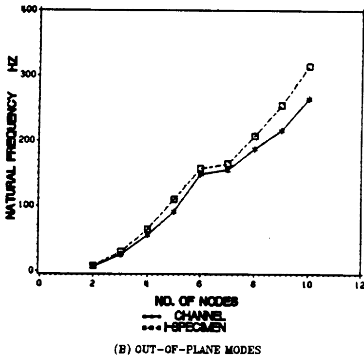
Figure 30. Comparison of clamped-clamped natural frequencies: The in-plane and out-of-plane natural frequencies for both specimens are compared in the two plots. The number of nodes in a mode is plotted on the horizontal axis and natural frequency in hertz on the vertical axis.
