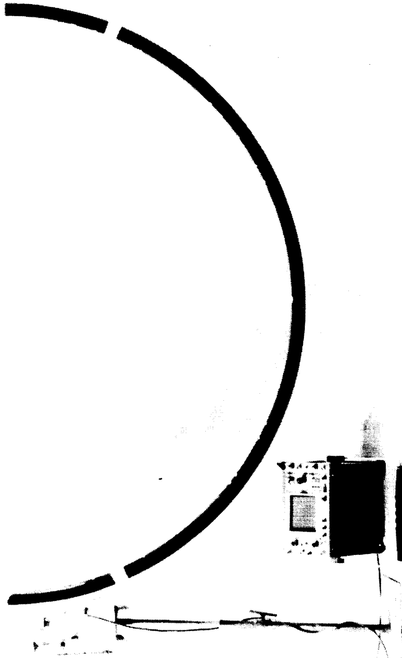
Figure 13. Free-free frame vibrational test setup: The specimens were hung by elastic bands at two points and excited at one end by an air shaker. The response of the frames was monitored using a velocity probe and an oscilloscope.
