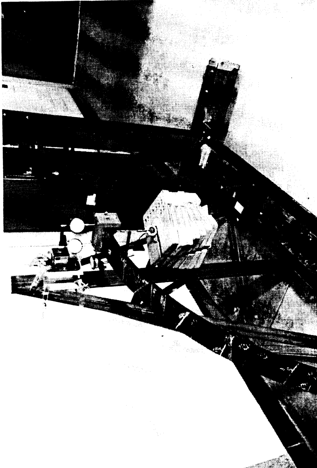
Figure 21. In-plane test apparatus: Twenty pound calibration weights were hung from the load fixture to generate the radial load. The torque was changed by moving the line of action of the radial load relative to the cross section.
