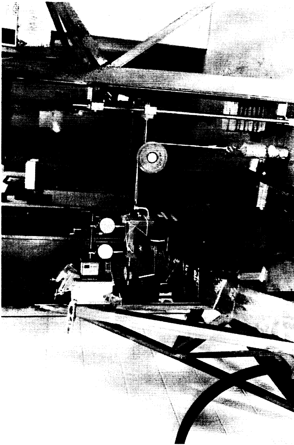
Figure 24. Out of plane test apparatus: Load path for the out-of-plane tests. The load was applied perpendicular to the frame by hanging weights from a line looped over a pulley.
