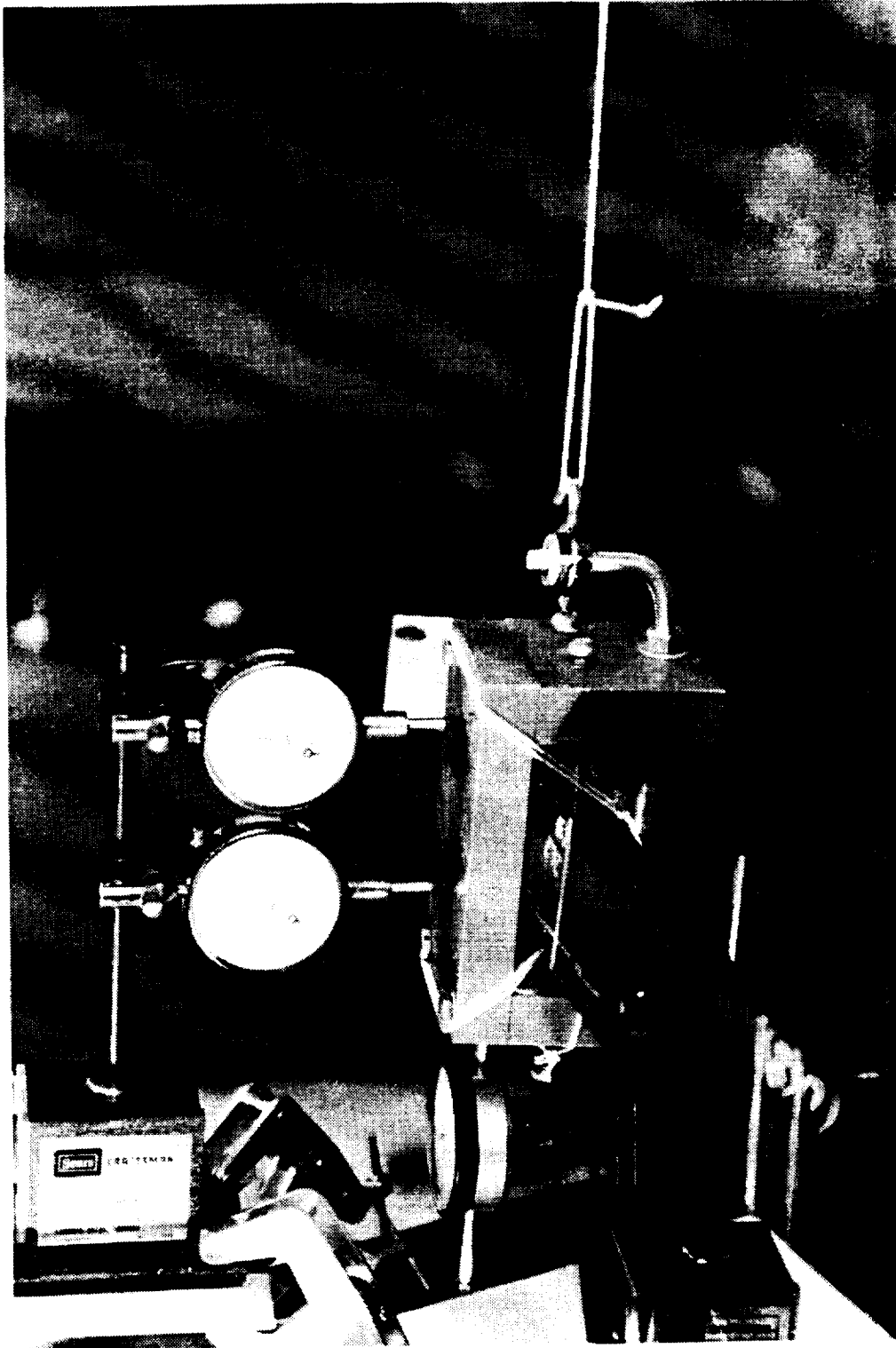
Figure 23. Photograph of modified load fixture and dial indicators: Dial indicators were used to measure the displacement of the load fixture at the midspan. The load fixture was tied to the specimen to force them to deform as a rigid body.
