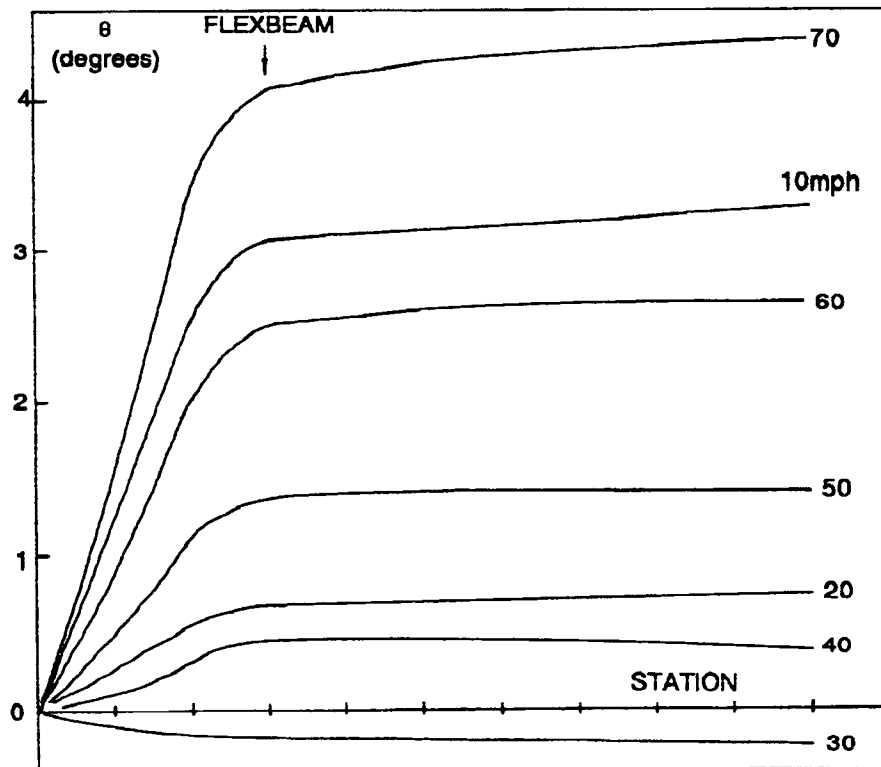
FIG. 6.5 UTRC ELASTIC TWIST (10-70 mph)
