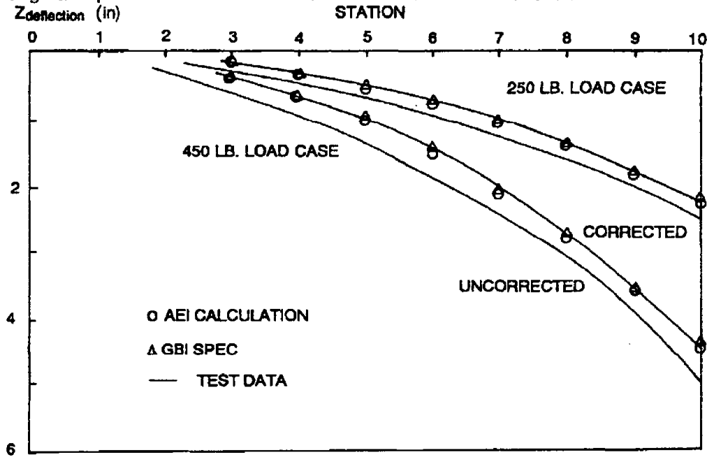
FIG. 5.12 ESI BLADE DEFLECTION: PREDICTIONS VS. TEST
