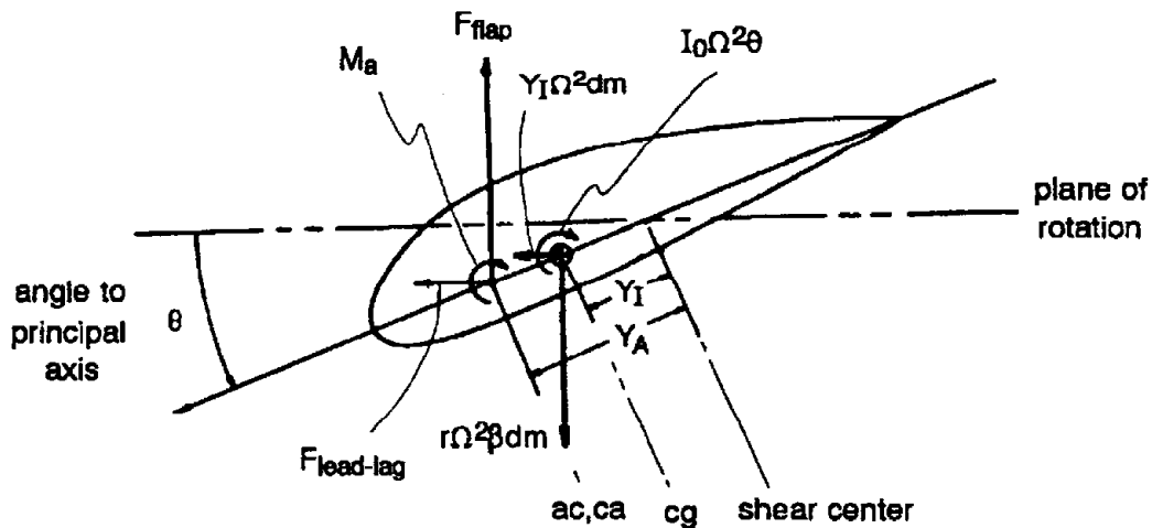
FIG. 6.2 BLADE SECTION FREE BODY DIAGRAM
