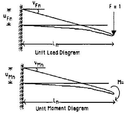
FIG. 4.7 UNIT LOAD AND MOMENT DIAGRAMS
