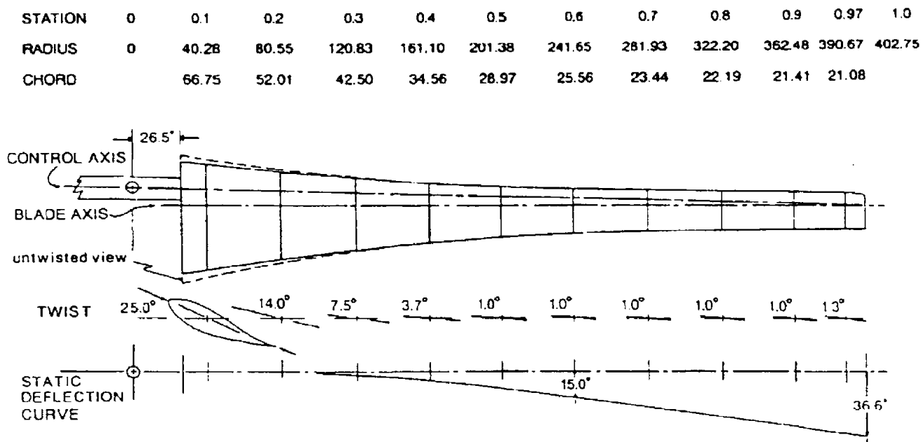
FIG 1.1 CARTER 300 BLADE
