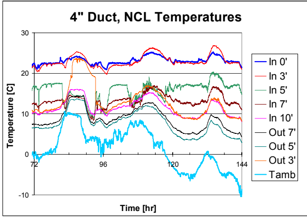
Fig. 6. Variation with temperature along the NCL. The bounding T_{\text{room}} , T_{\text{amb}} are shown as heavy lines. The temperatures decrease around the loop at night, until the pattern is broken with T_{\text{OUT@3'}} , which increases due to interaction with the room.
