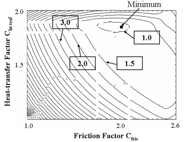
Fig. 7. Contours of \chi^2 as a function of (C_{\text{fric}}, C_{\text{ht-trsf}}) for all the data on the 4" diameter room-air NCL. Contour values are shown in the boxes, and the minimum is \chi^2_{\text{min}} \sim 1 , located at (C_{\text{fric}}, C_{\text{ht-trsf}}) = (2.05, 1.8) .
