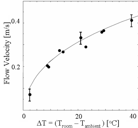
Fig. 8. Average duct flow velocity vs. \Delta T = T_{\text{room}} - T_{\text{ambient}} . Measured flow rates are shown as the solid dots. The model results with (C_{\text{fric}}, C_{\text{ht-trsf}}) = (2.05, 1.80) are the solid curve.
