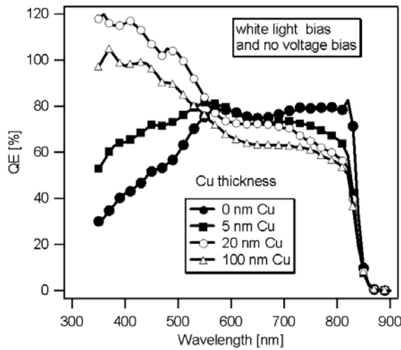
Fig. 7. QE curves under white light bias.
