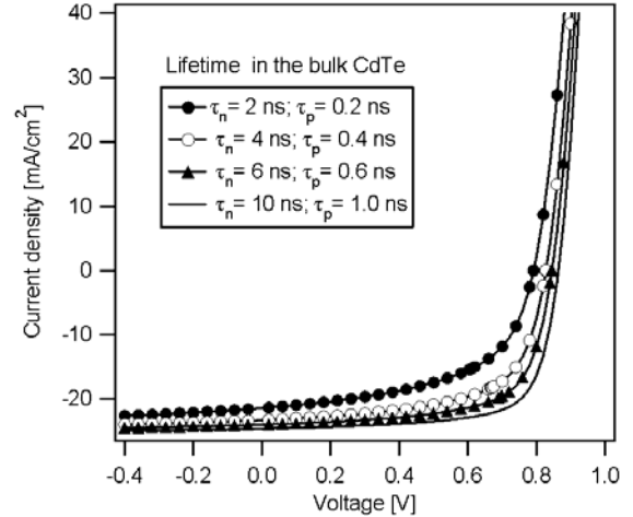
Fig. 6. Effect of lifetime on JV characteristics (simulated).
