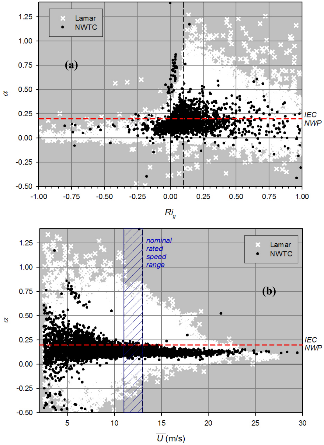
Figure 15. Comparison of the observed rotor disk shear exponent, \alpha , with: (a) turbine layer R_{i_g} , and (b) hub-height mean wind speed for the NWTC ART and over an equivalent rotor disk and hub-height of a GE 1.5 MW turbine installed at the Lamar Site. The IEC Normal Wind Profile (NWP) value of 0.2 is shown as - - - - -
