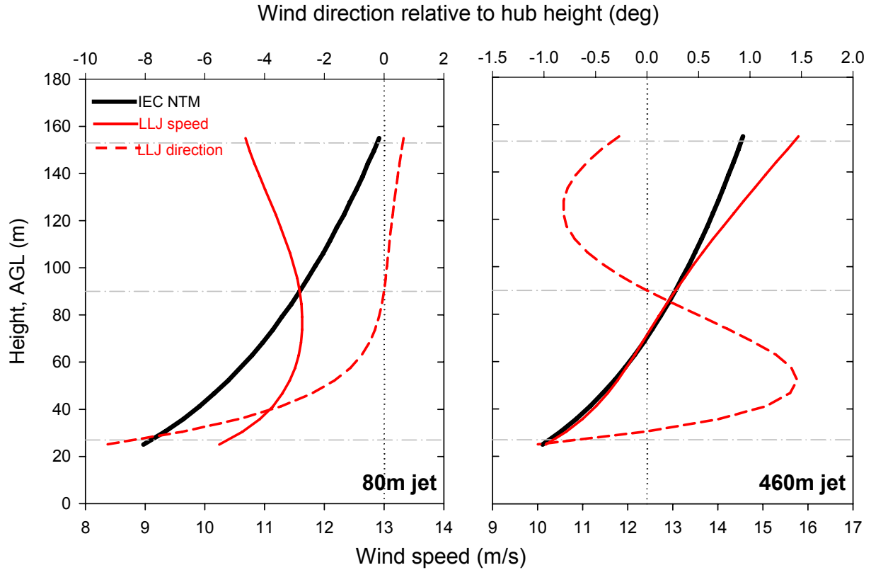
Figure 6. Vertical wind speed and direction profiles over 5-MW turbine rotor disk for simulated 80- and 460-m LLJs.
