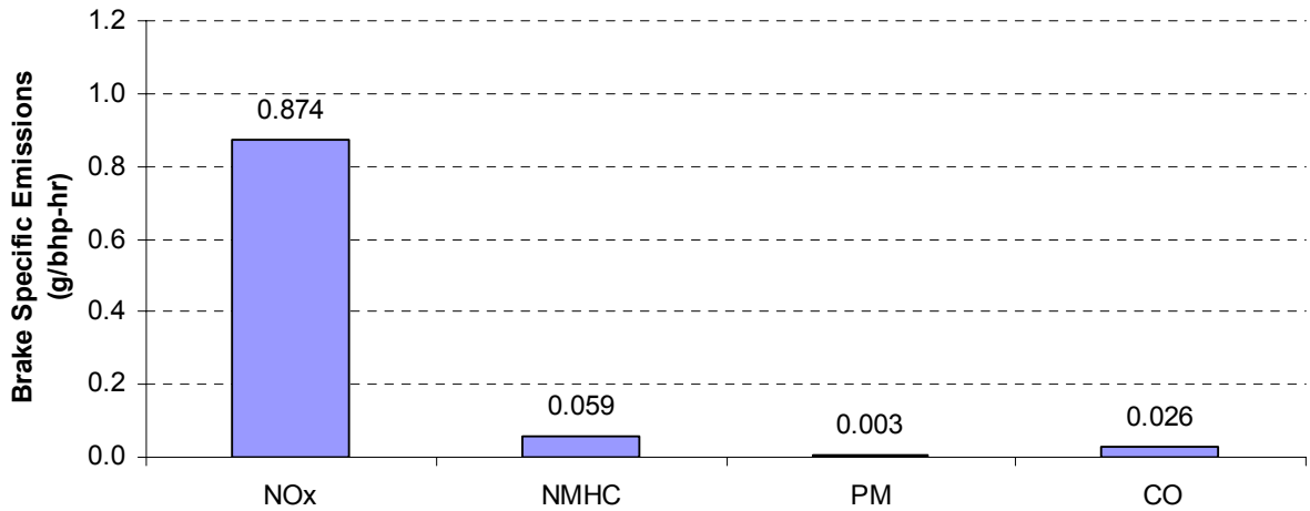
Figure 3-5. Summary of emission results for 250 hp rating
