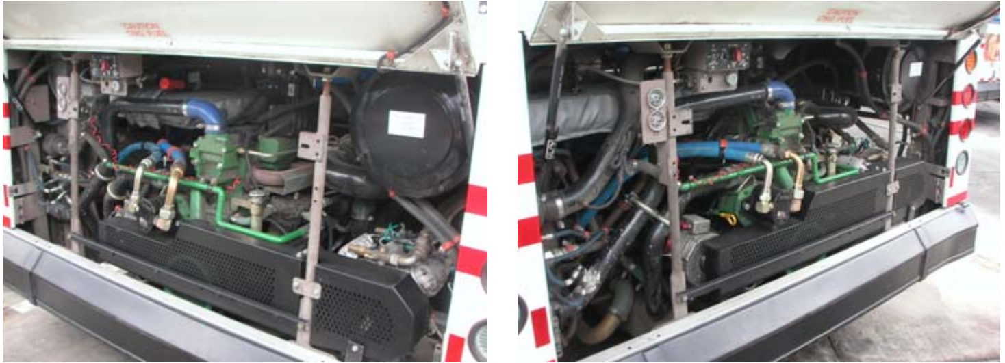
Photos 3-3 and 3-4. Views of John Deere 8.1 L engine installed in New Flyer Bus
