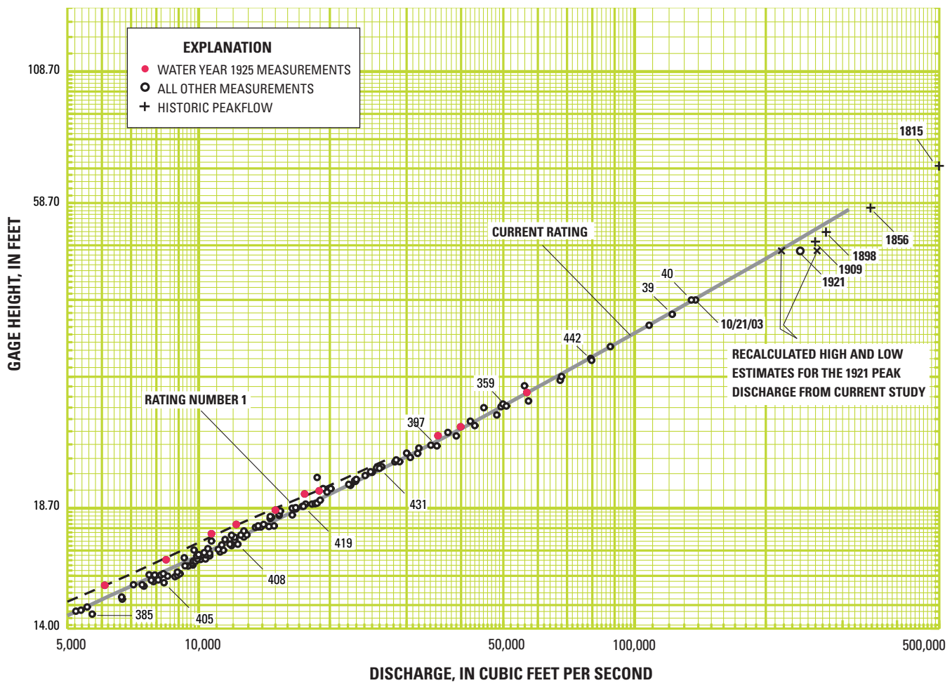
Figure 10. Current rating and rating No. 1 stage-discharge ratings for Skagit River near Concrete, Washington, with historical peak-flow discharges and recalculated high and low estimates of the peak discharge of the 1921 flood.
