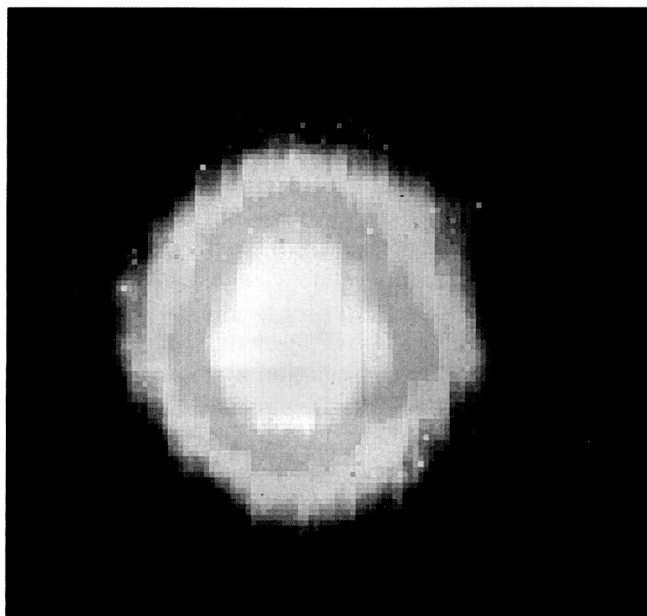
Ultraviolet image of Halley's Comet obtained by Pioneer Venus when the comet was close to perihelion
