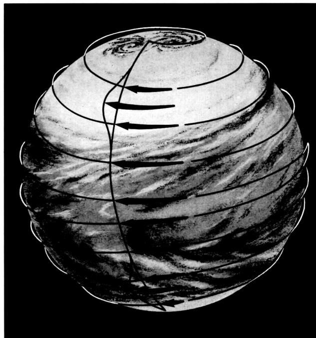
Diagram of global winds in the atmosphere of Venus as charted by Pioneer spacecraft
