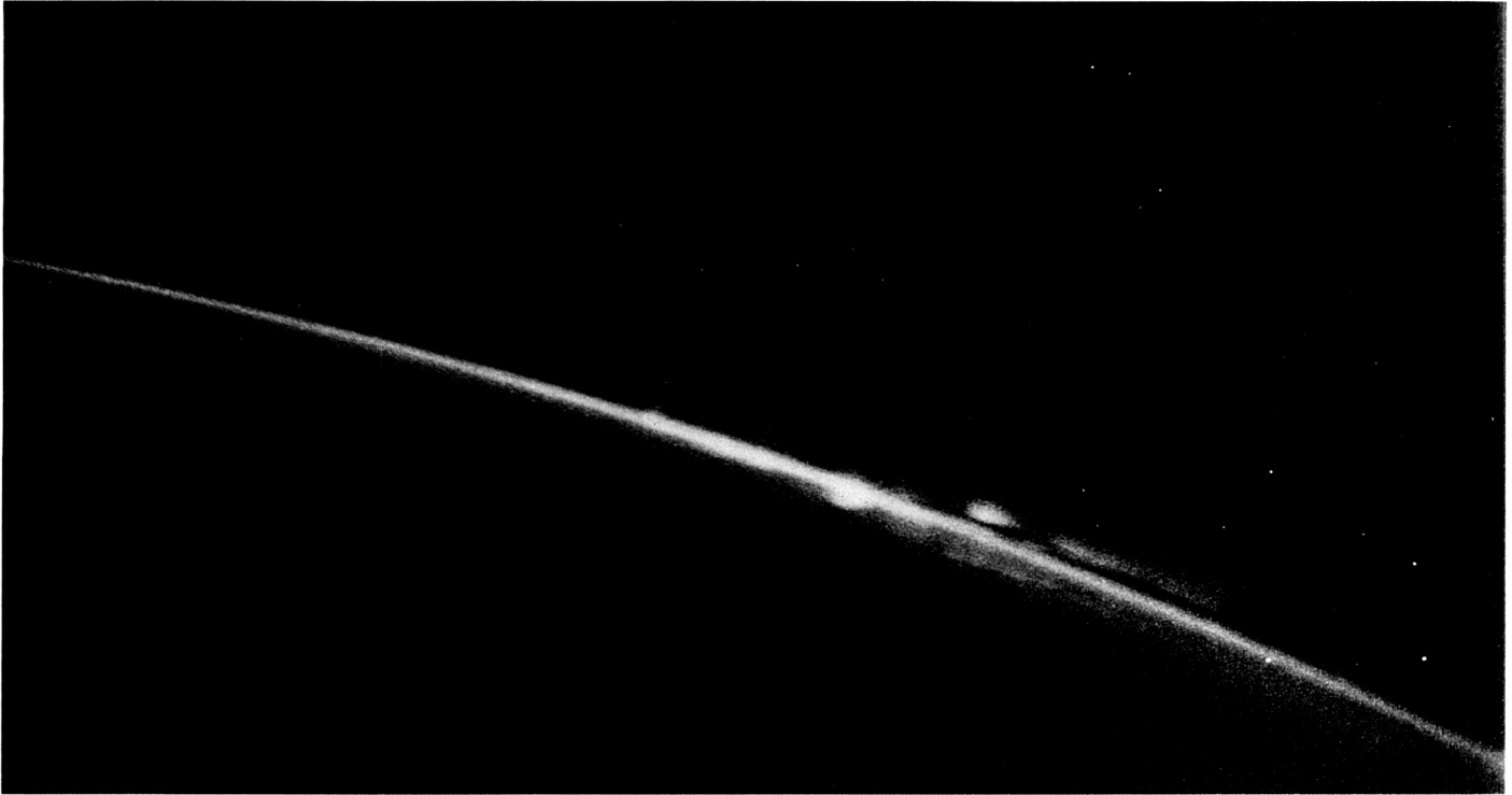
Terrestrial aurora as seen from Skylab
