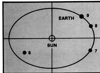
NOV 8, 1968
