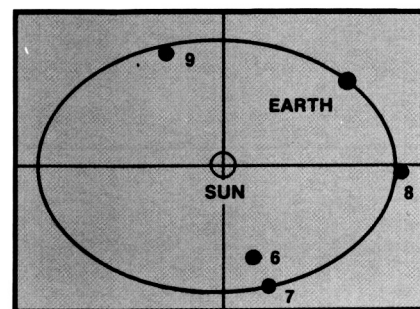
NOV 3, 1969
