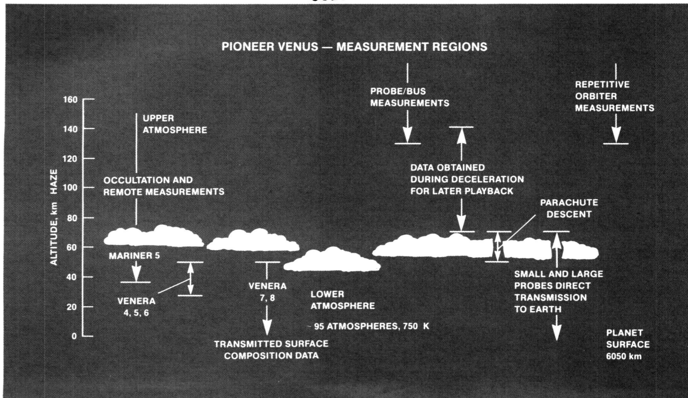
Regions of Venus' atmosphere explored by spacecraft
