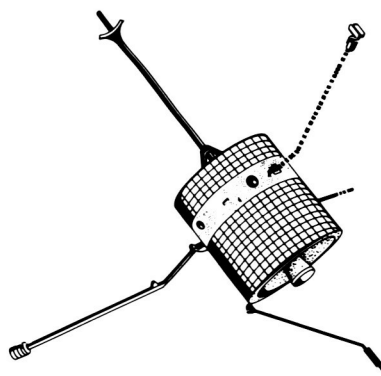
PIONEER 6-9 (1965-1968)
