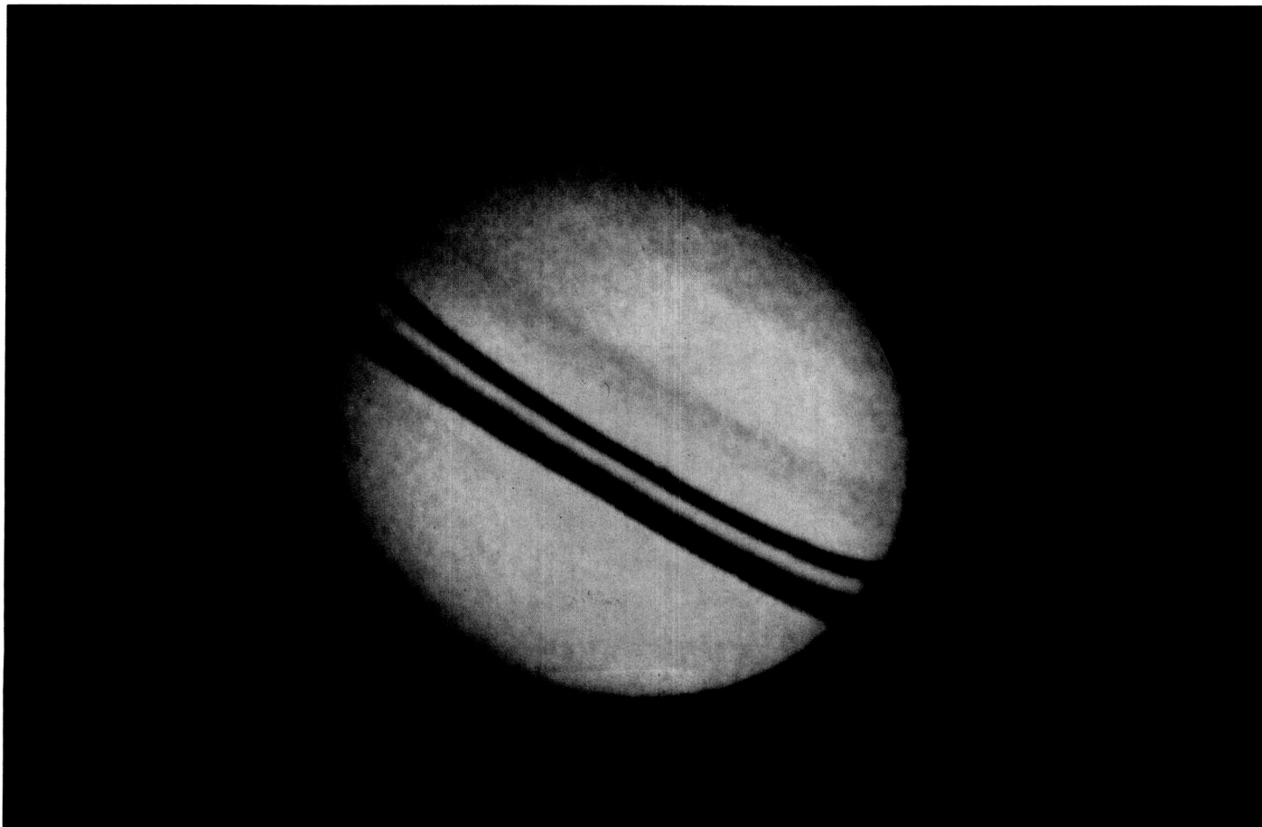
The planet Saturn and its majestic ring system
