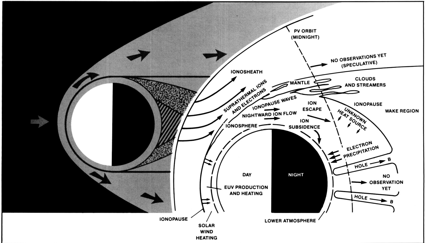
Diagram of the magnetosphere of Venus
