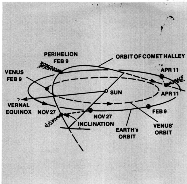
Halley's Comet, its path around the Sun in 1985/86 and its close approach to Pioneer Venus
