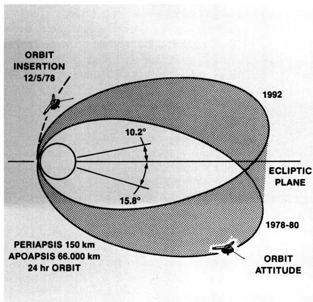
Changing orientation of Pioneer orbiter's path
