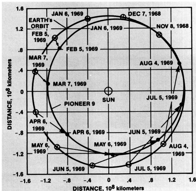
Pioneers mapped the solar wind patterns
