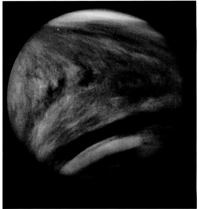
Planet Venus imaged from Pioneer Venus
