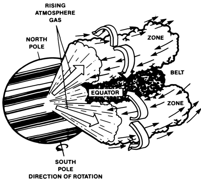
Diagram of the cloud belts and zones of Jupiter
