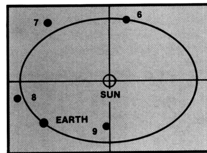
MAY 7, 1969
