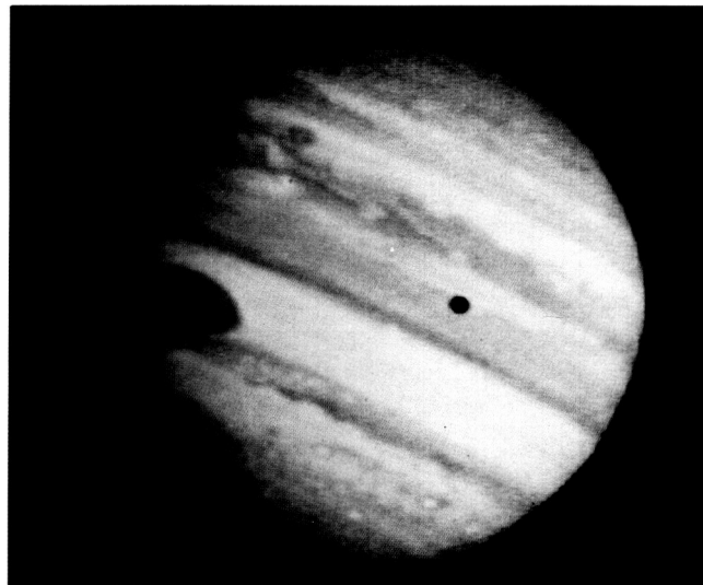
The planet Jupiter and its Great Red Spot
