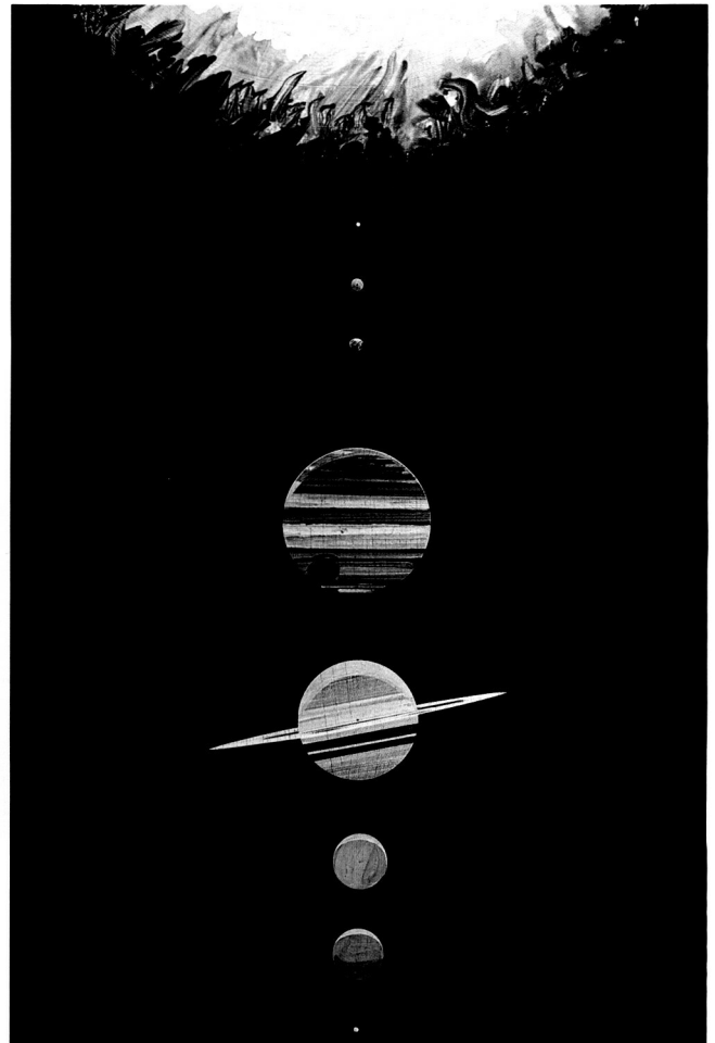
Comparative sizes of the planets and the Sun
