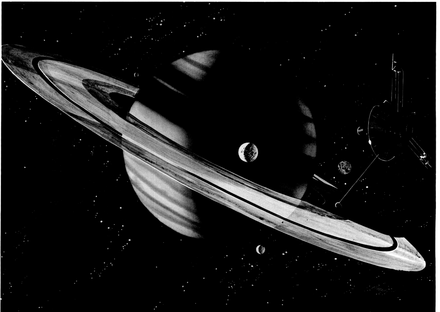
A Pioneer spacecraft flies by Saturn
