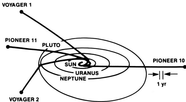
Relative paths of four spacecraft leaving the Solar System for interstellar space
