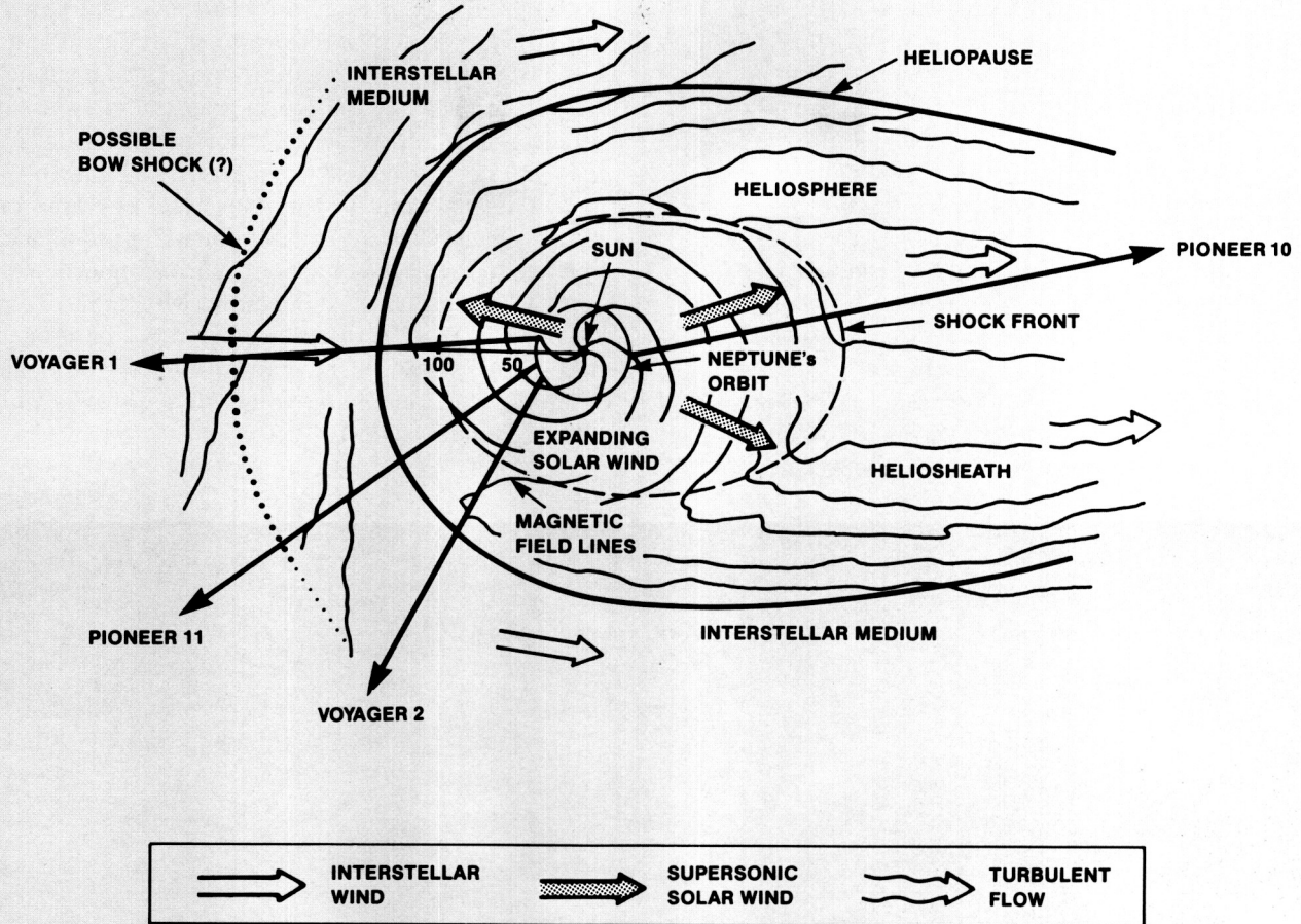
Paths of the Pioneer spacecraft through the heliosphere and out of the Solar System
