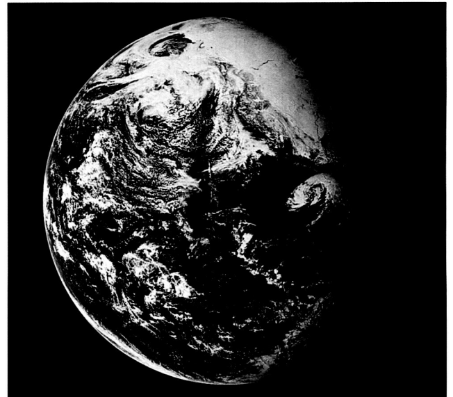
View of Earth from space centered on California
