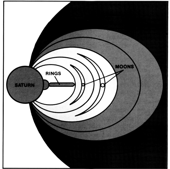
Diagram of the magnetosphere of Saturn discovered by Pioneer 11
