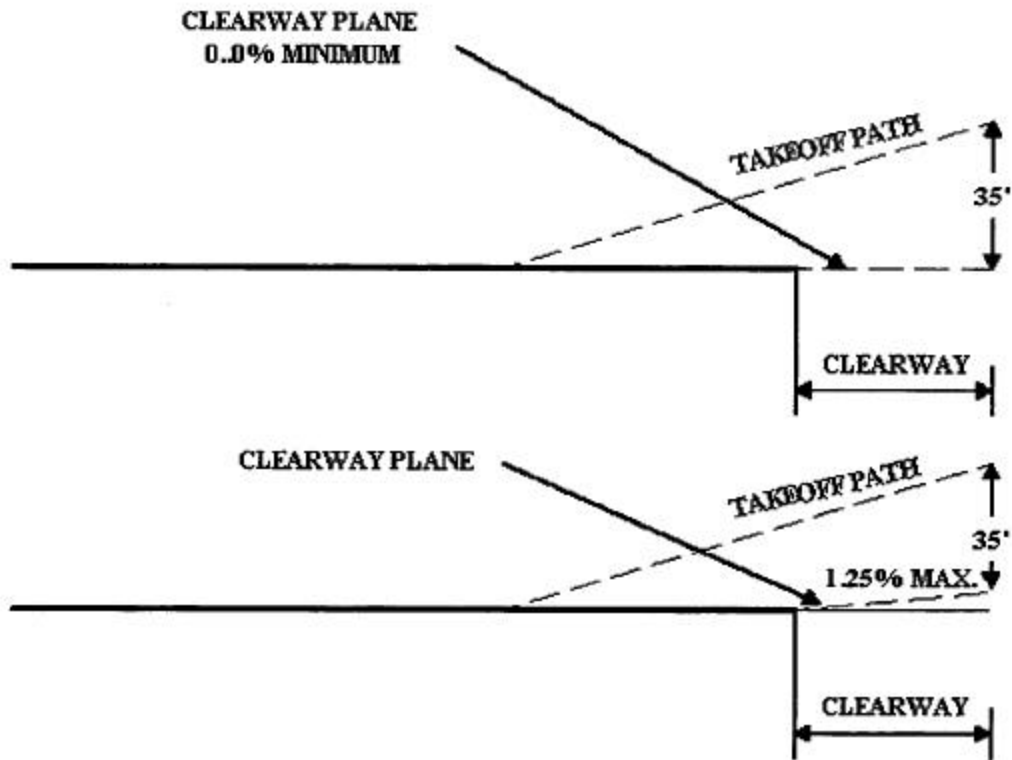
FIGURE 13-6. CLEARWAY PROFILES
