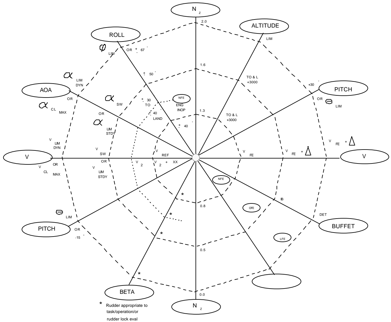
Figure 7: Flaps DOWN Flight Envelopes
