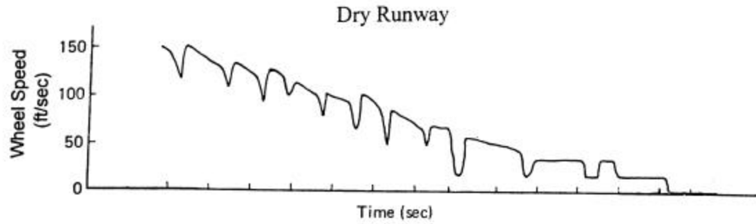
FIGURE 11-4. ANTI-SKID SYSTEM RESPONSE CHARACTERISTICS Quasi-Modulating System
