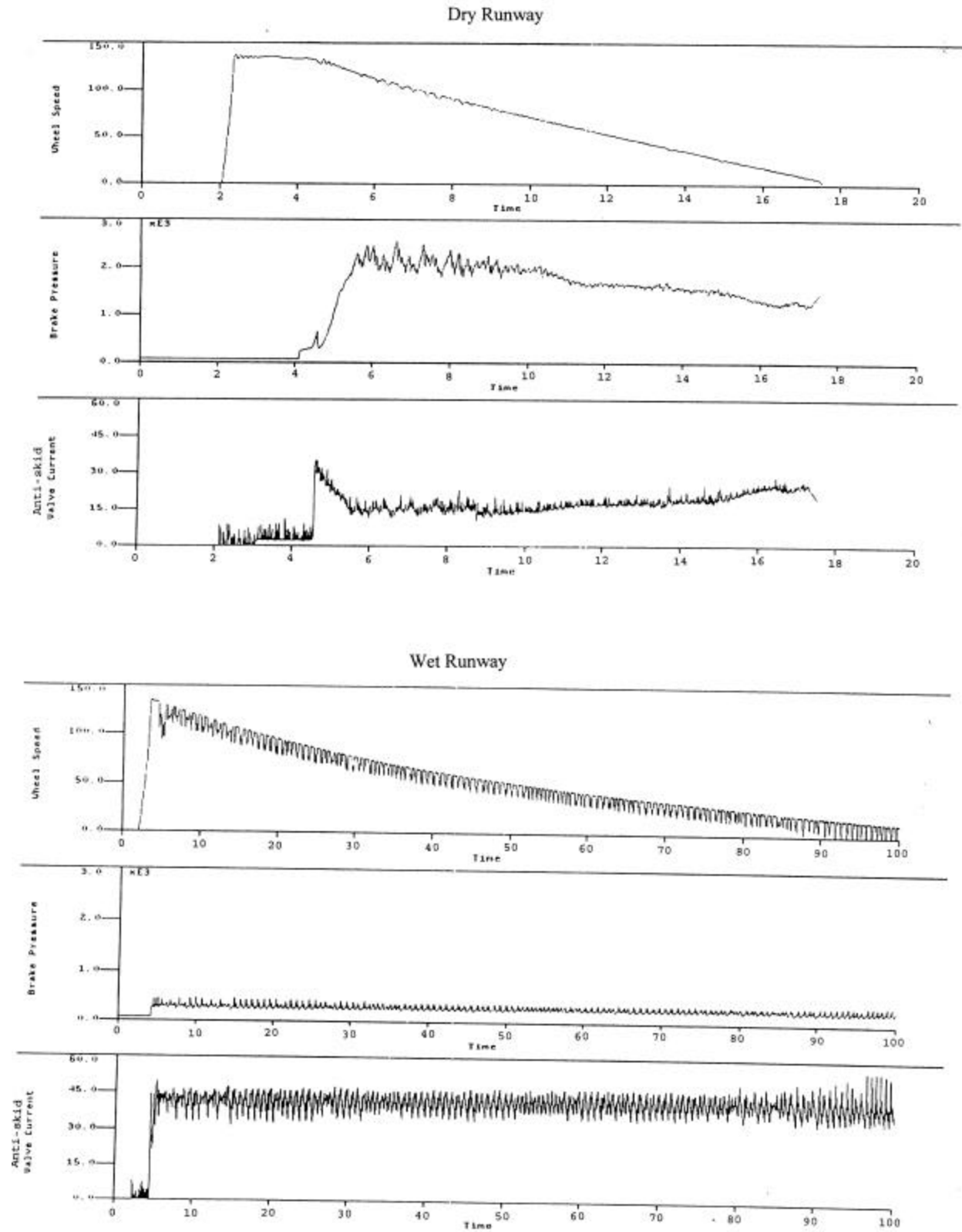
FIGURE 11-5. ANTI-SKID SYSTEM RESPONSE CHARACTERISTICS Fully Modulating System
