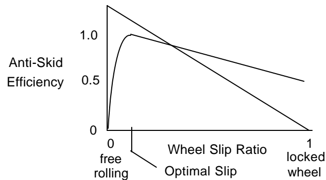
FIGURE 11-7. ANTI-SKID EFFICIENCY - WHEEL SLIP RELATIONSHIP
