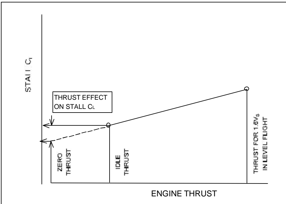
FIGURE 29-5. THRUST EFFECT ON STALL C_L
