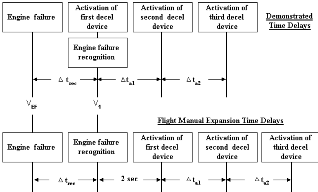
FIGURE 2 ACCELERATE-STOP TIME DELAYS (Amendment 25-42 thru Amendment 25-91)
