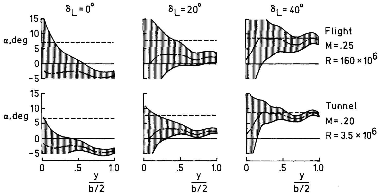
Figure 17.- Program estimate of the range of full thrust for the candidate flap system.
