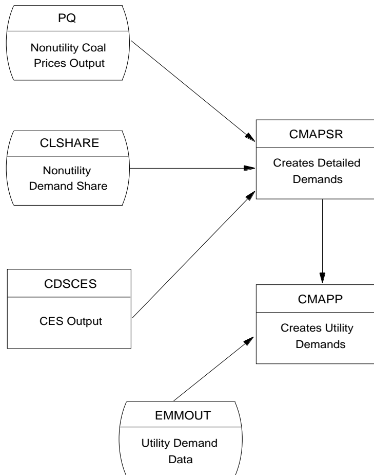
Figure 11. Functions of Subroutine “CMAPSR”
