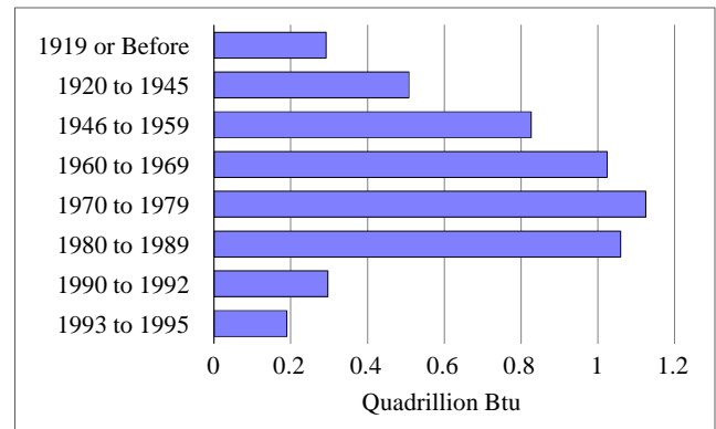
Figure 16. Site Energy Consumption by Year Constructed, 1995
