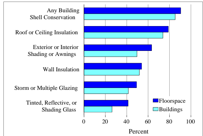
Figure 50. Building Shell Conservation Features in Commercial Buildings, 1995
