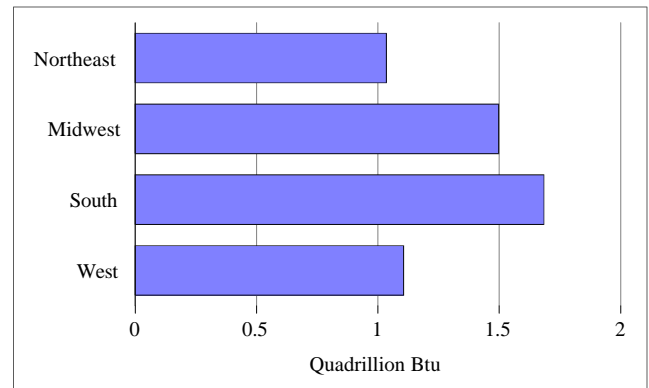
Figure 19. Site Energy Consumption by Census Region, 1995
