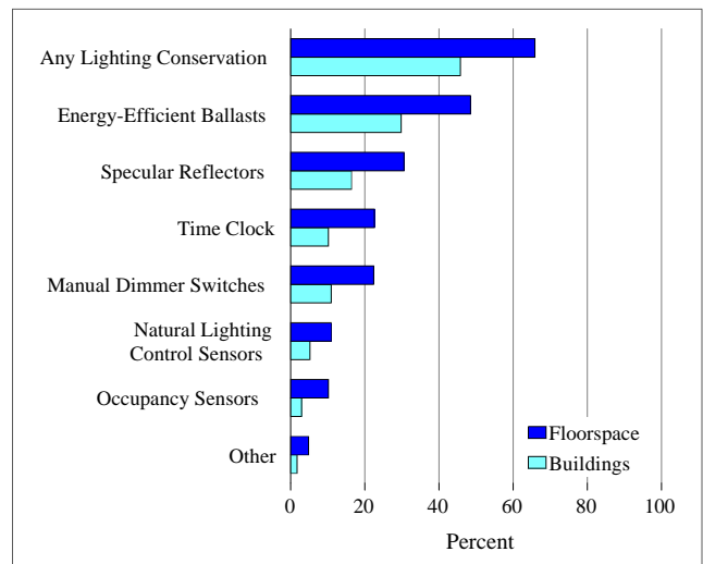
Figure 52. Lighting Conservation Features in Commercial Buildings, 1995
