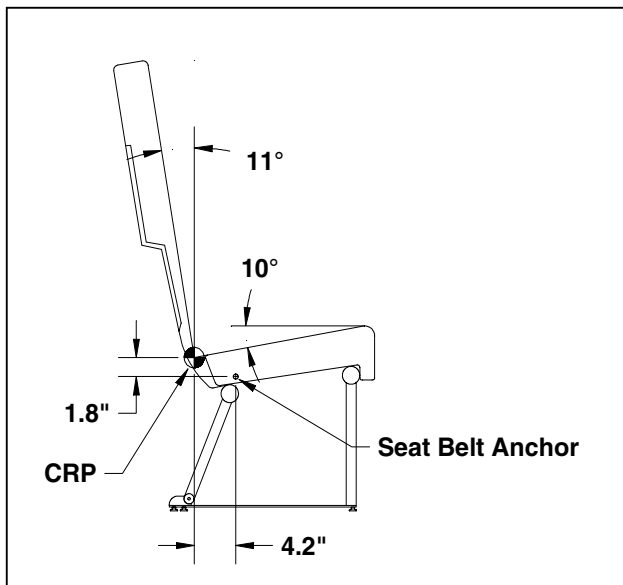
Figure 2. Tension Study Seat Dimensions
