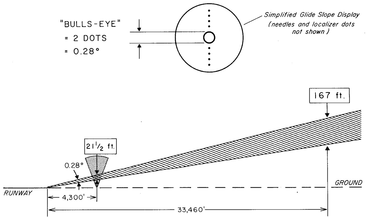
FIGURE 12. A two dot deviation, equal to a vertical displacement of the glide slope needle across the span of the crosspointer bull's eye, is equal to about 0.28 of subtended angle, resulting in a narrowing of the glide slope "beam" as the middle marker is approached.
