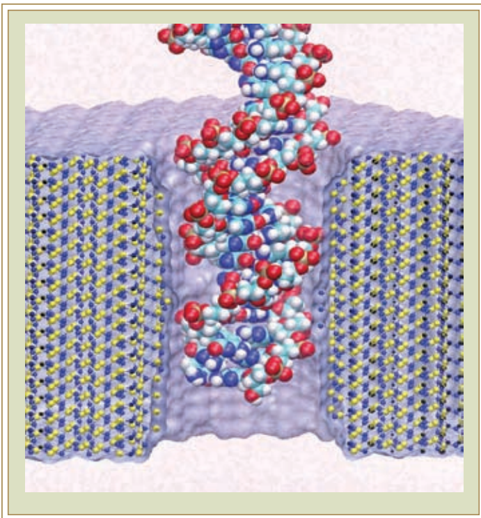
Visualization of a molecular dynamics simulation of a double stranded DNA molecule as it enters a nanopore in a silicon nitride membrane.
