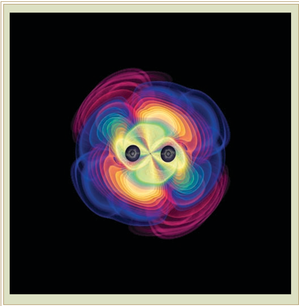
This numerical simulation, created on the NCSA Itanium Linux Cluster by international researchers, shows the merger of two black holes and the ripples in space time that are born of the merger.
