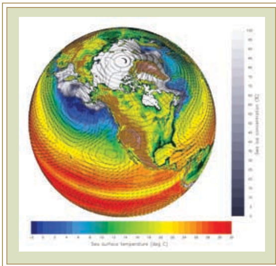
Results from the Parallel Climate Model, prepared from data in the Earth System Grid, depict wind vectors, surface pressure, seas surface temperature and sea ice concentration.
