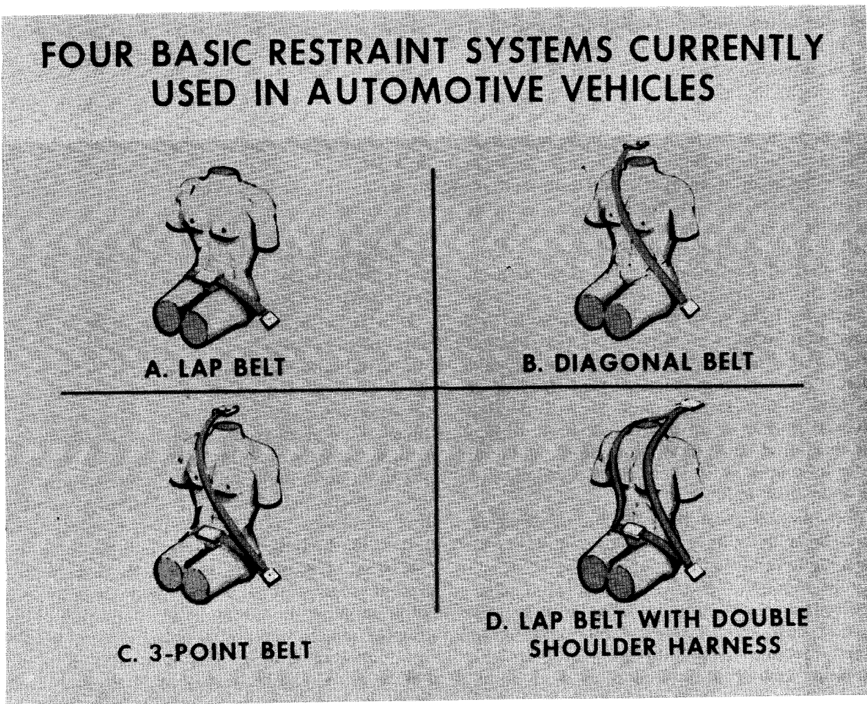
FIGURE 1. Four basic restraint systems currently used in automotive vehicles.
