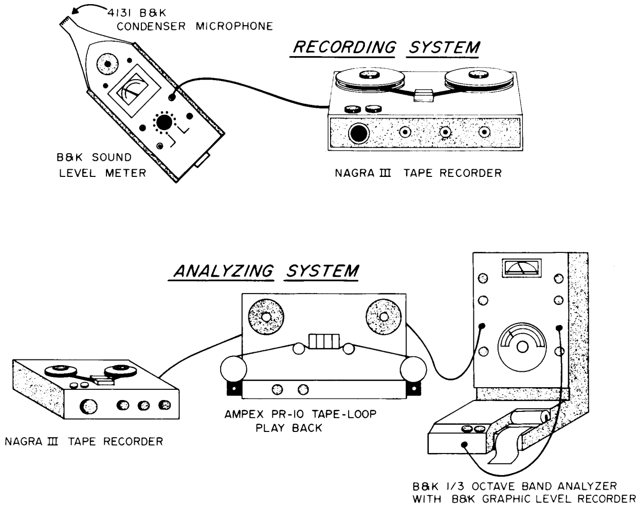
FIGURE 1. Diagrams of the recording and analyzing systems used.
