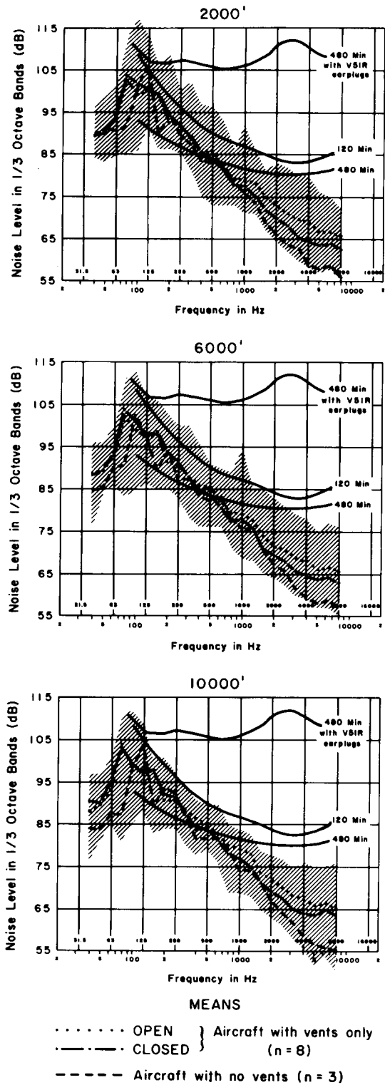
FIGURE 3. Effects of ventilation on cockpit noise. 3a shows the mean values for each condition of ventilation at 2000 feet MSL; 3b shows the same information at 6000 feet; and 3c shows it at 10000 feet. The solid lines represent DRC curves.
