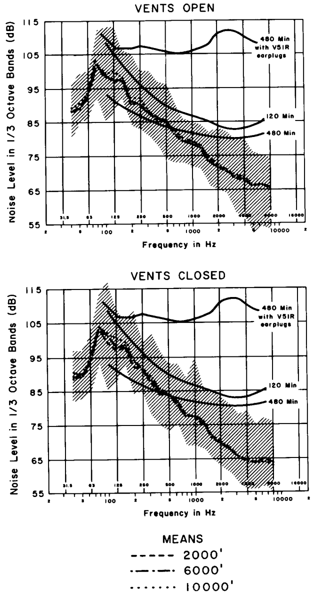
FIGURE 2. Effects of altitude on cockpit noise. 2a shows the mean values for each altitude when the vents were open (in the 8 aircraft so equipped). 2b shows the values when the vents were closed. The solid lines represent DRC curves.
