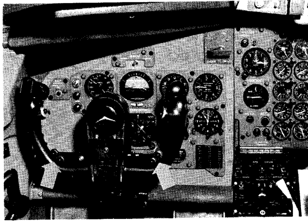
FIGURE 3. Peripheral vision cues relating to aircraft bank angle were provided by two sets of small colored lights attached to pilot's control wheel (arrows). Upper bulbs were red, lower ones green.
