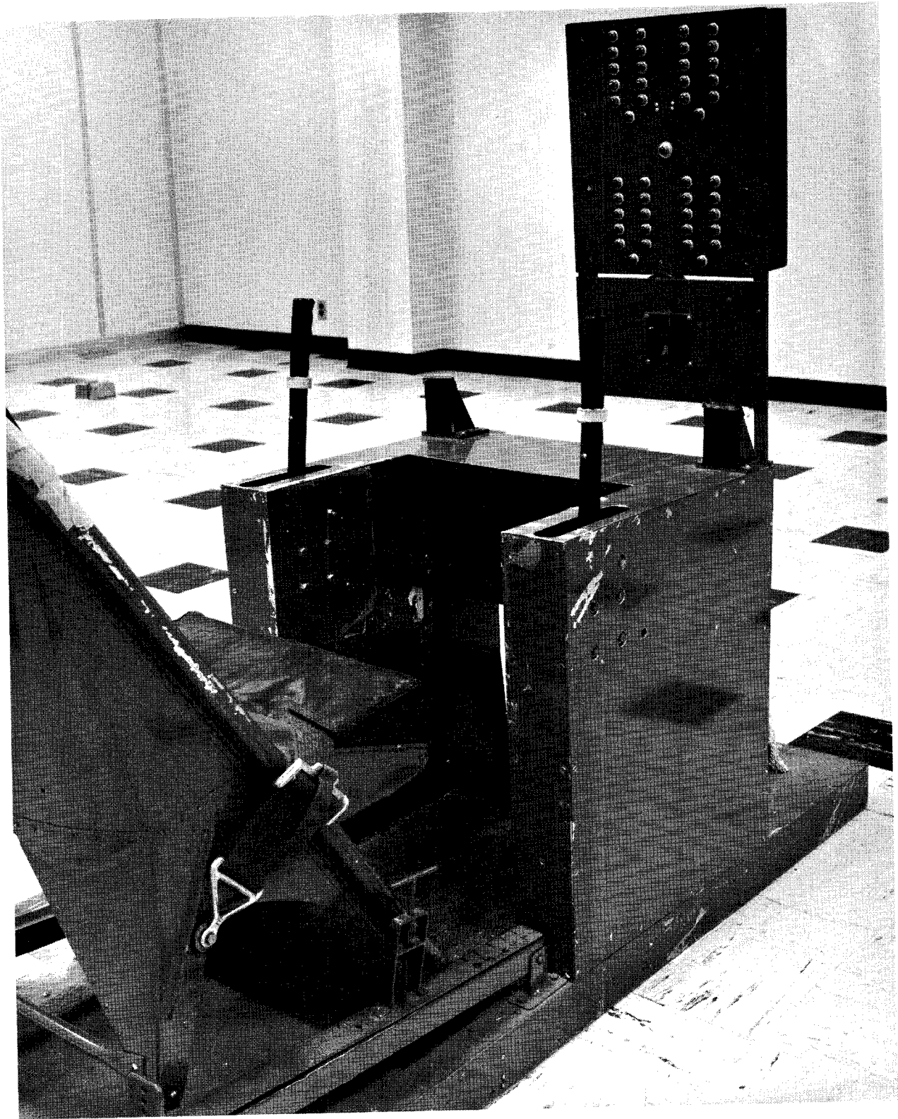
FIGURE 1. Modified Mashburn Coordinator.
