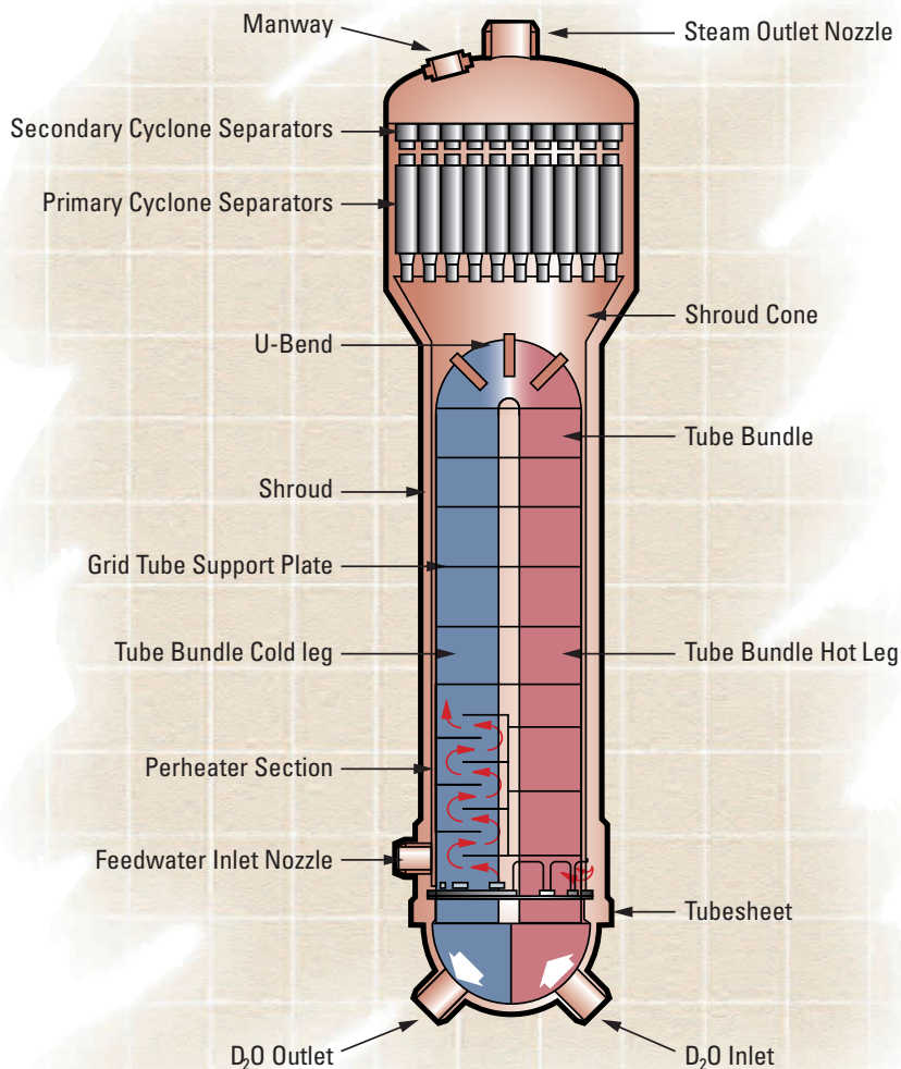
Steam Generator
