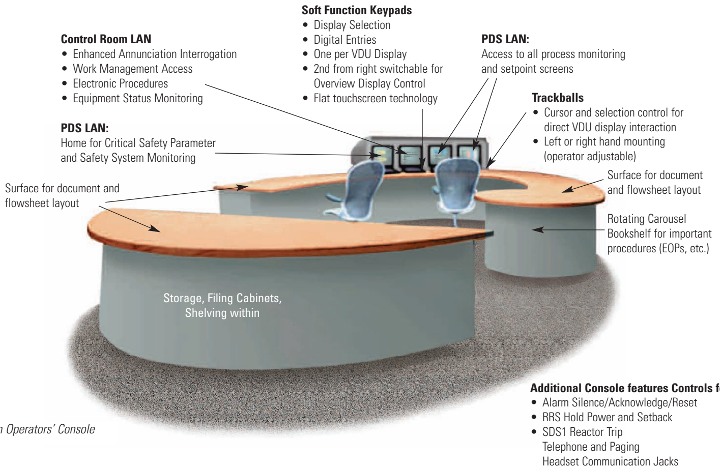
Qinshan Phase III Unit 1, Control Room
