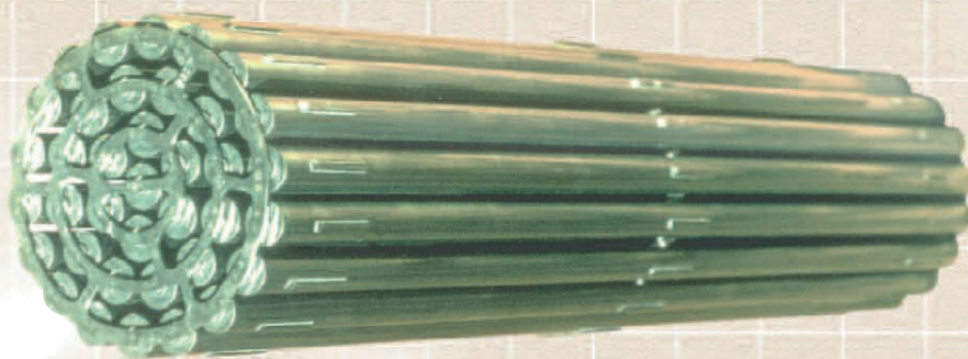
37 Element Fuel Bundle
