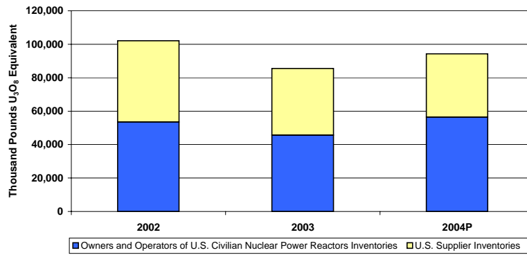
Figure 20. Commercial Inventories of Natural and Enriched Uranium as of End of Year, 2002-2004
