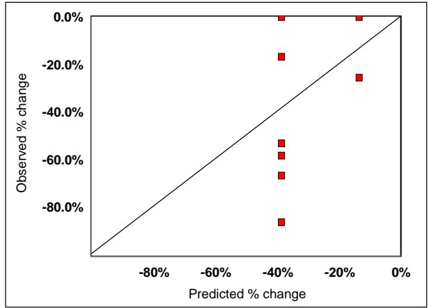
Figure V.B-8 Predicted vs observed HC for nonroad using R49 correlation
