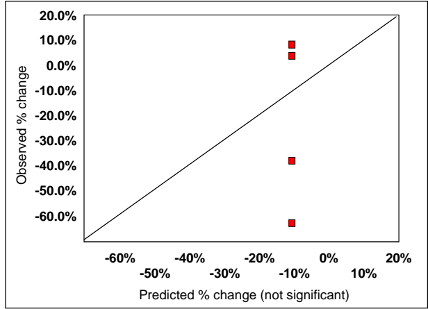
Figure V.B-6 Predicted vs observed PM for nonroad using R49 correlation
