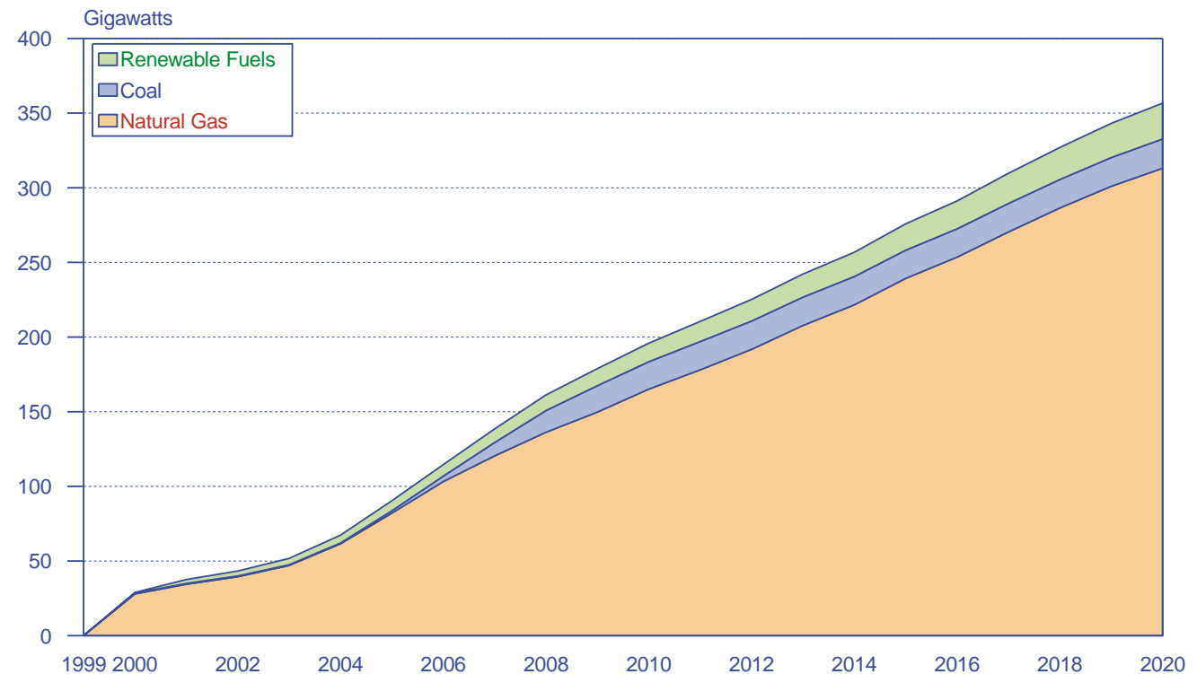
Figure 4. Projected Cumulative Additions to U.S. Electricity Generating Capacity, 1999-2020
