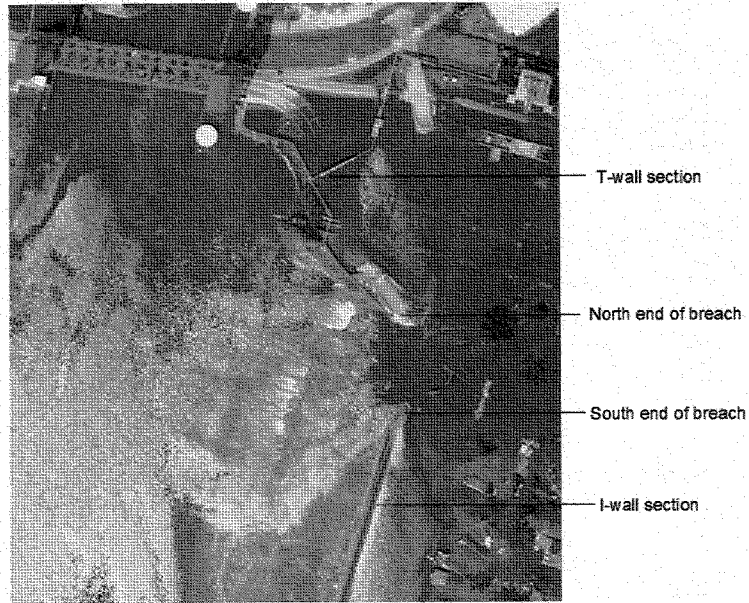
Figure 4.7: Airborne digital imagery of the north breach at the Lower Ninth Ward. Water is shown flowing back into the IHNC (courtesy NOAA, August 31, 2005).
