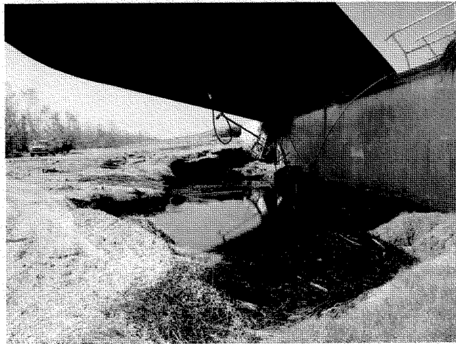
Figure 4.14: Scour near barge damage at the Bayou Bienvenue Gate site (J. Wartman, October 5, 2005).
