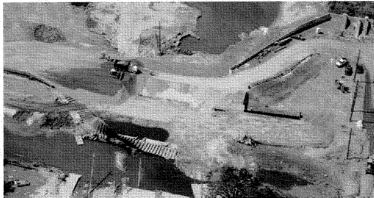
Figure 4.9: Aerial view of the north breach of the Lower Ninth Ward (L. Harder, October 14, 2005).
