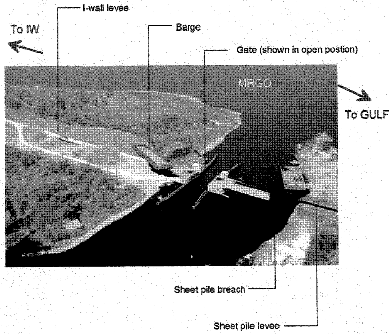
Figure 4.12: Northwest facing aerial view of the Bayou Bienvenue Gate structure (L. Harder, October 14, 2005).
