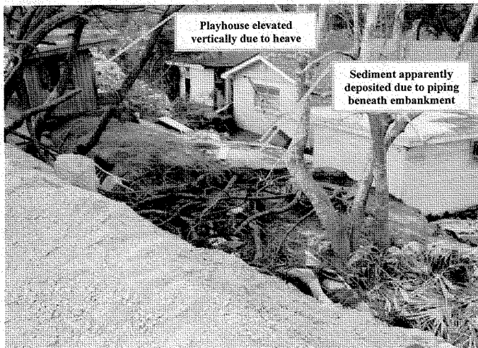
Figure 2.16: Conditions at the inboard toe of the London Avenue Canal (North) breach section.
