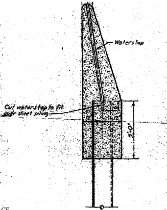
Figure 2.2(a): Typical I-wall section in the New Orleans region.
