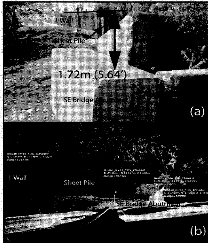
Figure 7.15: Photograph of the southeast abutment of the London Avenue Canal bridge at Robert E. Lee Blvd (a), and LIDAR scan of the same location (b). New soil and rock apparently fills scour and sink hole erosion beneath the abutment. The relative height gap between the bridge abutment and the flood wall is 1.72 meters (5.6 feet).
