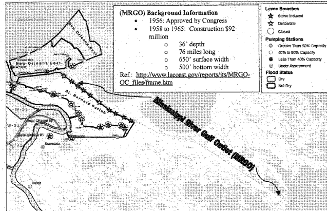
Figure 4.19: Mississippi River Gulf Outlet [MRGO] (USACE). The two yellow stars (i.e., deliberate breaches) along MRGO seem to correspond to locations of gate structures where storm-induced breaches occurred. These yellow star markers are likely errors in the original map that should have been designated using blue star markers.
