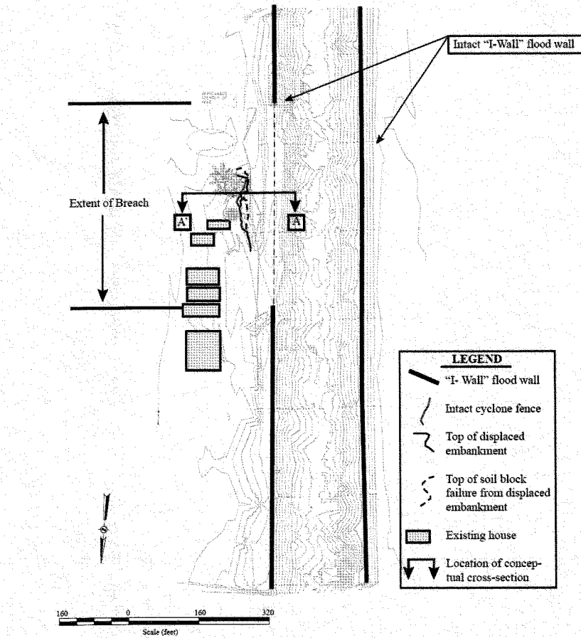
Figure 2.6: Schematic plan view of the 17 th Street Canal breach site. Results of LIDAR scan superimposed on base survey.
