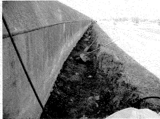
Figure 4.4: North view from the end of the south breach of Lower Ninth Ward. Note how the scour trench becomes progressively wider as it approaches the breach (J. Wartman, October 4, 2005).
