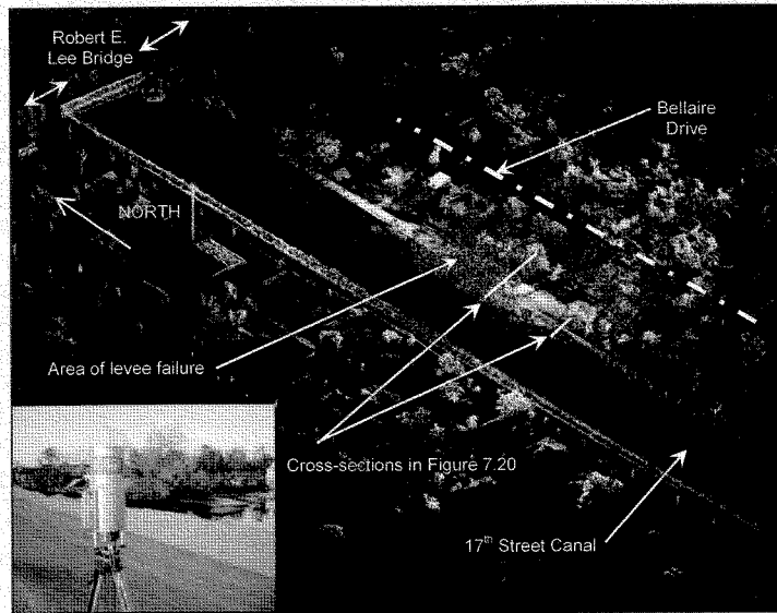
Figure 7.18: Overview oblique image of the 17 th Street Canal area in the vicinity of the breach. The Robert E. Lee Blvd. Bridge is to the north (upper left) and the breach area is to the upper right (east). Houses within the neighborhood breach area and the scour pond were imaged from the new levee and Bellaire Drive.
