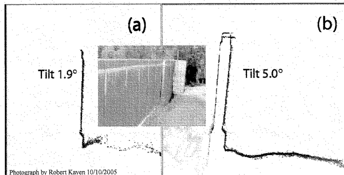
Figure 7.14: Cross sections through two segments of distressed I-wall at London Avenue Canal. Segment (a) is toward the south (left) of Figure 7.13 and has a modest 1.9 degree rotational deformation toward the landside of the levee. Near a position of maximum distress, the I-wall has 5.0 degrees of rotational deformation.
