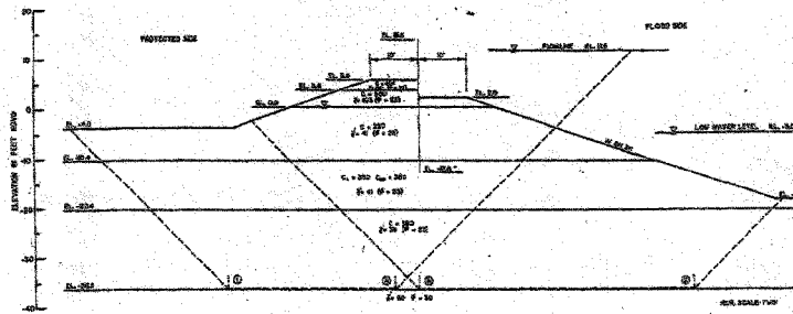
Source: Eustis Engineering, "Geotechnical Analyses, Metairie Relief Canal (17th Street Canal), OLB Project No. 2043-0222, New Orleans, Louisiana, 31 August, 1988.
