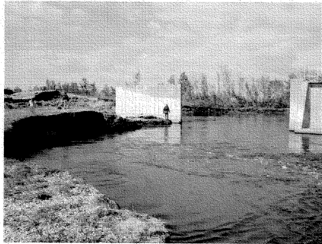
Figure 4.23: Ground perspective of Bayou Dupree gate abutment failure (L. Wooten, October 6, 2005).
