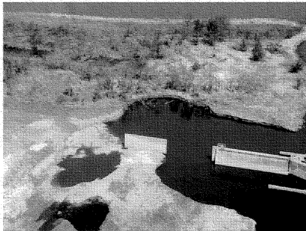
Figure 4.22: Levee failure on southwestern bank of MRGO at Bayou Dupree. Note concrete sheetpile and levee transition washouts (L. Harder, October 14, 2005).
