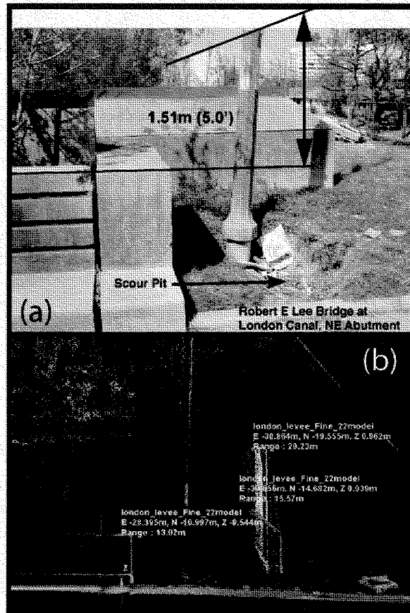
Figure 7.17: Photograph taken directly south and adjacent to the northeast abutment of the Robert E. Lee Bridge (a), and corresponding LIDAR scan of the same location (b). A scour trench is clearly visible beneath the abutment. The wall gap here is 1.51 meters (5.0 feet).
