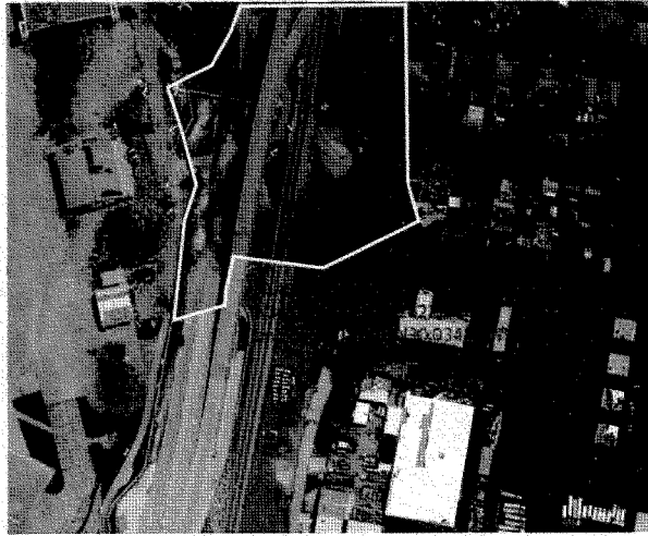
Figure 7.9: Sites 6 & 7, Lakefront Airport Levee Transition Breach: (N30.03367° W90.02622°) and airport Levee I-Wall: (N30.03436°
