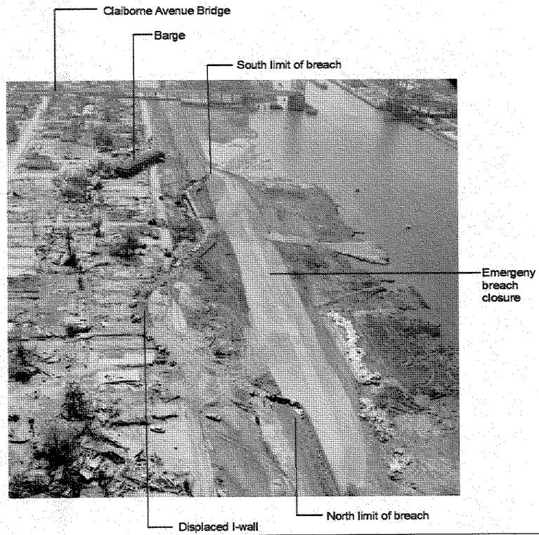
Figure 4.2: Aerial view of the south breach at the Lower Ninth Ward (L. Harder, October 14, 2005).
