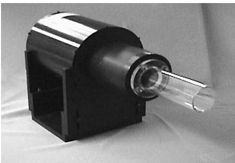
Three versions of this standard are used for pulsed-laser calibrations. The Q-Series, developed in the 1980s is used for 1.06 \mu m lasers. The QUV and QDUV calorimeters, developed in the 1990s are in current use for calibrations at 248 nm and 193 nm, respectively.
