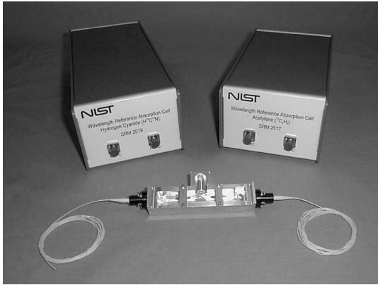
Wavelength calibration Standard Reference Materials.
