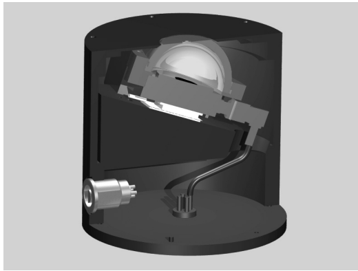
A three-dimensional representation of a new pyroelectric-based radiometer head for infrared optical measurements as part of a collaboration with the NIST Optical Technology Division. The critical detector element and gold-black coating are being developed in the Optoelectronics Division.
