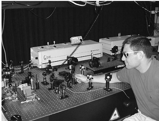
Ultrafast measurement system with tunable wavelength for pump-probe characterization of compound semiconductor structures.
