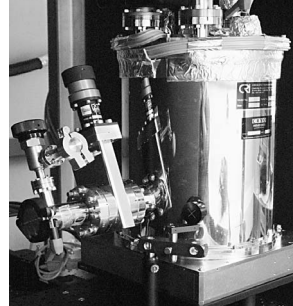
The Laser-Optimized Cryogenic Radiometer, developed in the late 1990s, and used for the highest accuracy measurements with low-level cw lasers, 100 \mu W to 1 mW at wavelengths from 0.4 \mu m to 2 \mu m.
