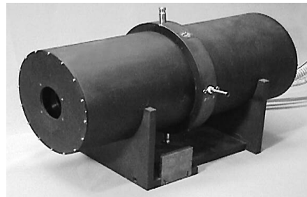
The K-Series Calorimeter, developed in the 1970s, for high power cw lasers in the range from 1 W to 1000 W and wavelengths from 0.4 \mu m to 20 \mu m. In current use for calibrations.
