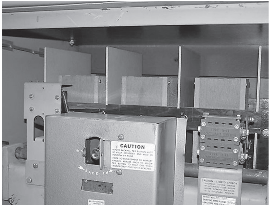
Figure 5: Obsolete Electrical Systems at the National Air and Space Museum
