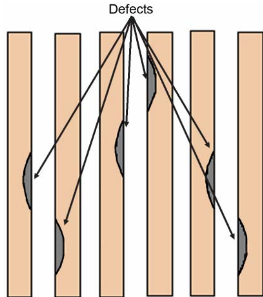
Figure 5—Defects of each group of six low- or no-value 2 by 4s were randomly distributed. Lumber was resawn into web sections to fabricate a value-added laminated I-beam. (Courtesy of Chris Wallace, Structural Research Engineer, Wyoming Sawmill, Inc.)
