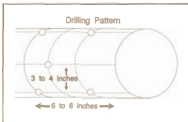
Figure 3. Pattern for drilling holes in logs.
