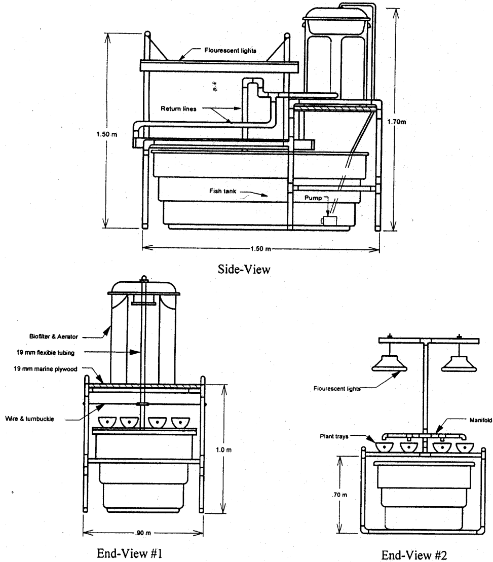
Fig. 1. Classroom scale aquaponics unit. Note: All structural components are 2.5-cm (1-inch) PVC pipe, unless otherwise noted.
