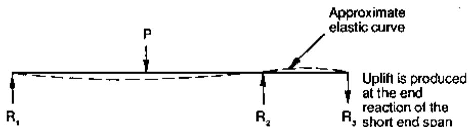
Figure 6-21. - Uplift force on a continuous-span superstructure.
