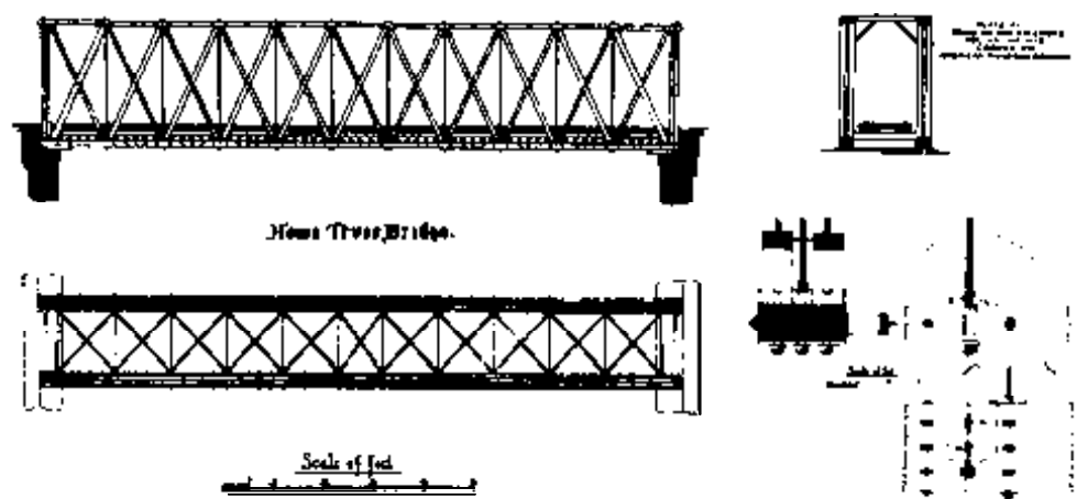
Figure 1-15.- Howe truss bridge patented in 1840 (photo courtesy of the American Society of Civil Engineers; © 1976. Used by permission).
