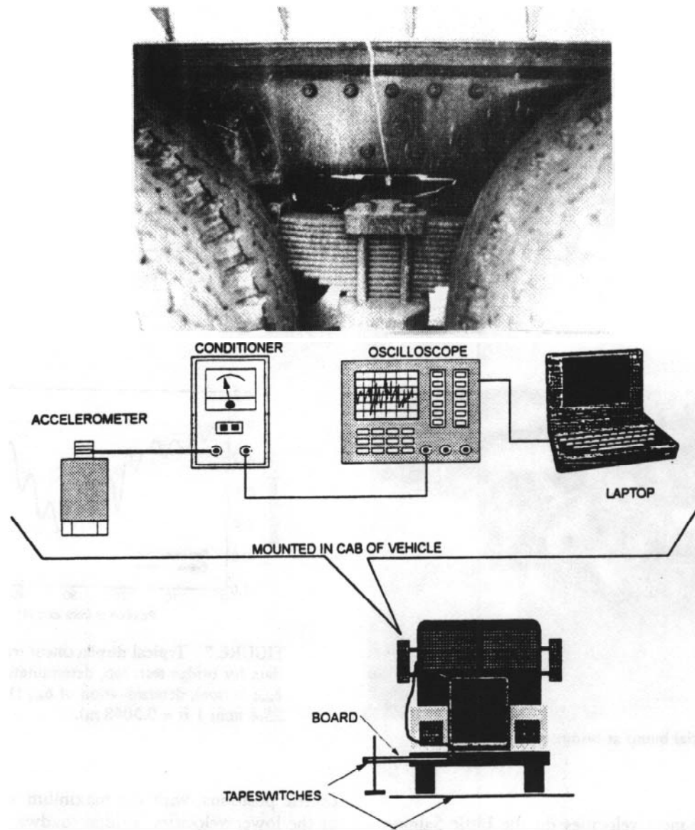
FIGURE 5 Vehicle data acquisition system: top , accelerometer mounted on frame; bottom , schematic of layout.
