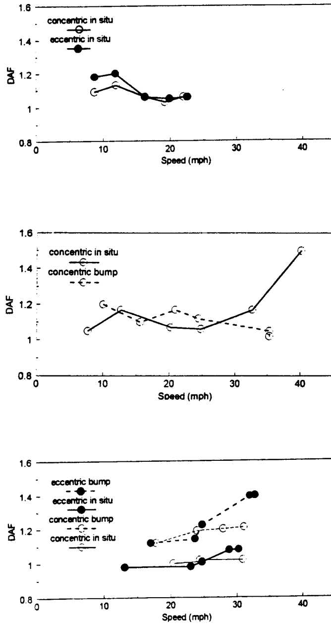
FIGURE 11 DAFs for field-tested bridges: top , Trout Road; middle , Little Salmon; bottom , Lampeter (1 mph = 1.61 km/hr).
