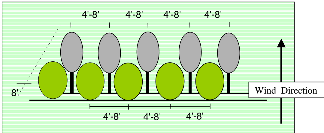
Figure 6. Wedge shape planting suggested to generate higher air-flow over the shelterbelt.
