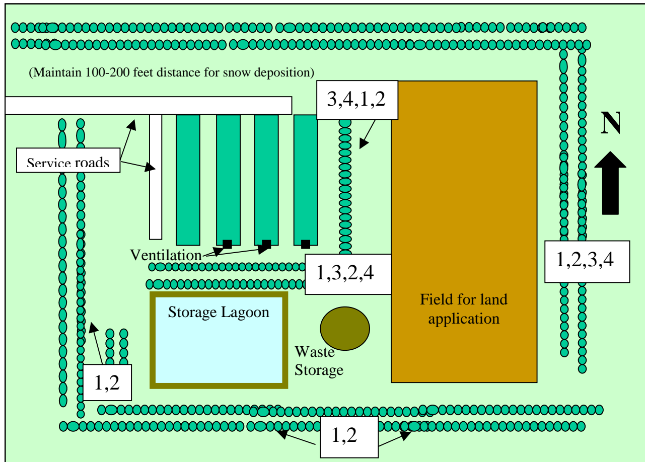
Figure 7. A hypothetical shelterbelt system design for a typical swine production facility. The numbers refer to the functional interaction and means by which the shelterbelt will mitigate livestock odor. The number 1 refers to creation of air mixing turbulence, the number 2 refers to dust deposition, the number 3 refers to particulate interception, and the number 4 refers to sites of air pollution sinks. Other important design considerations include: livestock type, odor sources, air/wind patterns, the species of trees/shrubs used. Another concern is the location of access openings and roadways. Openings should, as much as possible, be located so as not to breach the shelterbelts interception of prevailing winds. Another very important factor to be understood is typical snow deposition patterns. It is undesirable to place any vegetation in a way that cause snow deposition to become troublesome, in fact vegetative placement can help to ameliorate snow problems and cut down on snow removal labor and costs (For more information see Wray et al, 1997 and Quam et al, 1996.)
