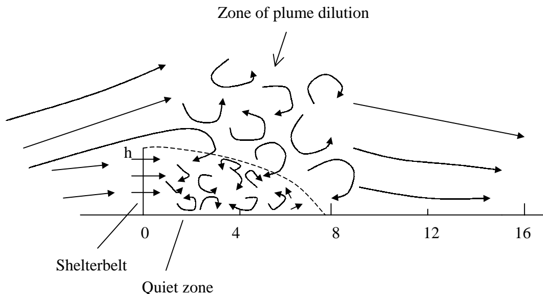
Figure 3. Schematic representation of turbulence and zone of potential odor dilution. Adapted from Raine (1974) as used in McNaughton (1988).
