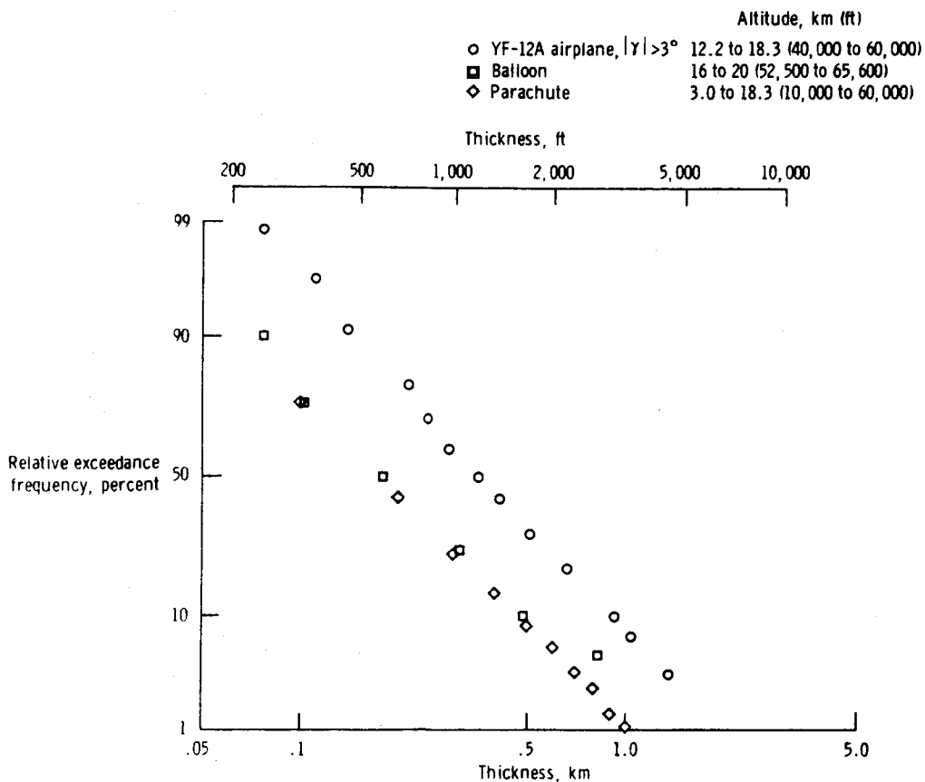
Fig. 4 Turbulence Patch Thickness Distributions From Three Sources
