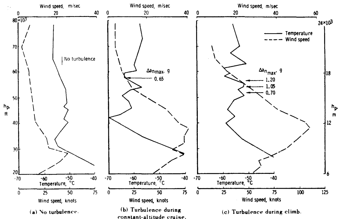
Fig. 5 Example Wind and Temperature Profiles for Various Turbulence Conditions (observed gust accelerations are noted at their respective flight altitudes)
