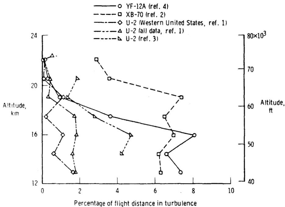
Fig. 1 Amount of Turbulence Versus Altitude
