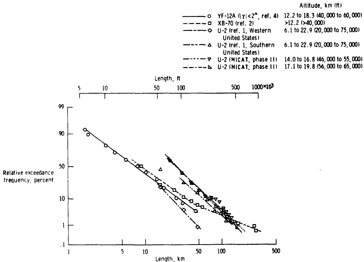
Fig. 3 Comparison of Turbulence Patch Length Distributions From Various Sources
