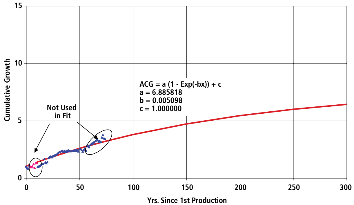
Figure A7-9. Paradox/San Juan Basins Exponential Curve Fit of Tight Formation Liquids Cumulative Growth Factor
