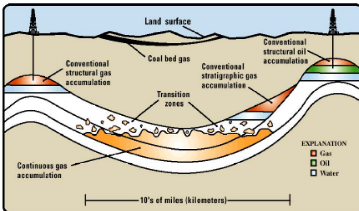
Figure A6-1. Conventional vs. Continuous Accumulations
