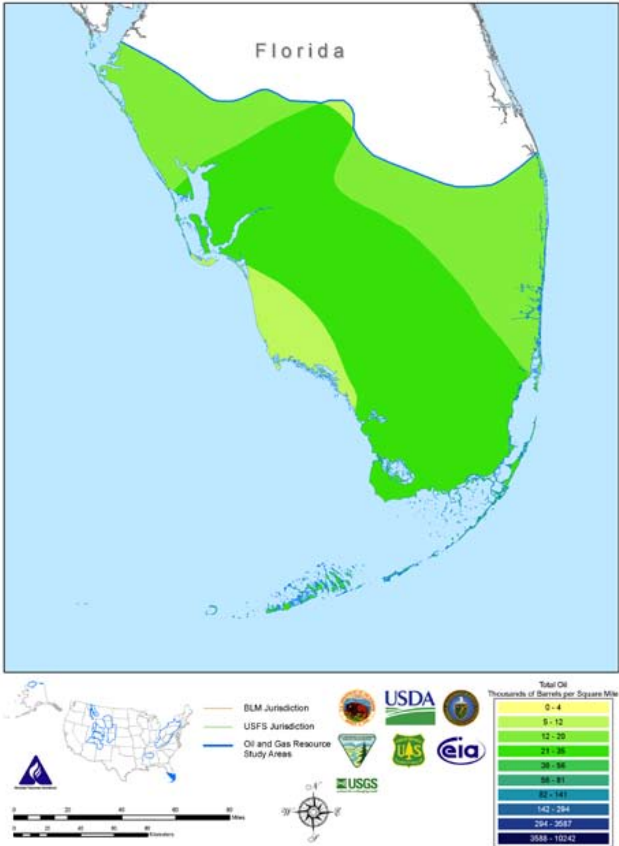
Figure 2-22. Total Oil Map, Florida Peninsula Study Area
