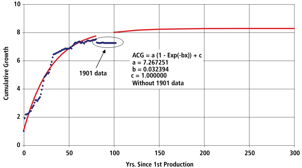
Figure A7-21. Denver Basin Exponential Curve Fit of Equivalent Oil Cumulative Growth Factor
