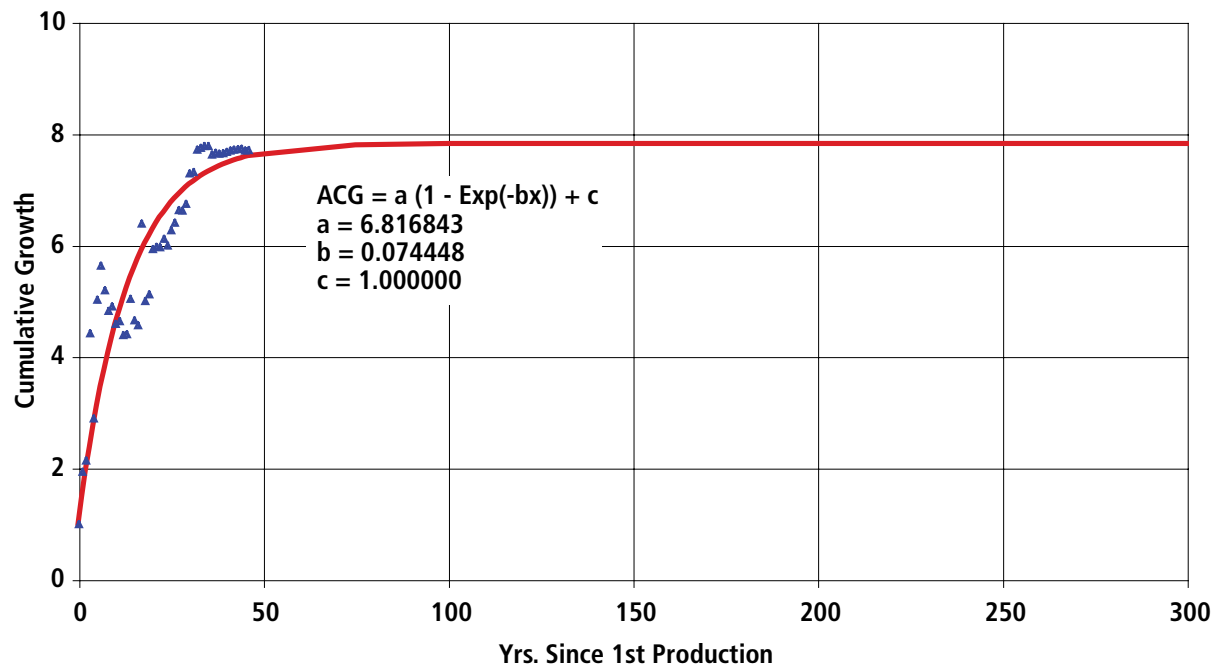
Figure A7-2. Uinta-Piceance Basin Exponential Curve Fit of Tight Formation Equivalent Oil Cumulative Growth Factor
