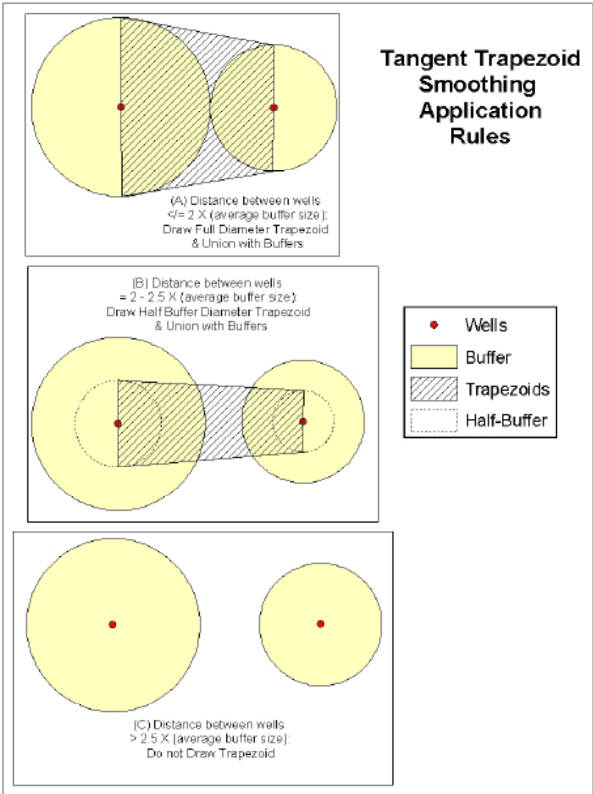
Figure A8-6. Tangent Trapezoid Smoothing Rules
