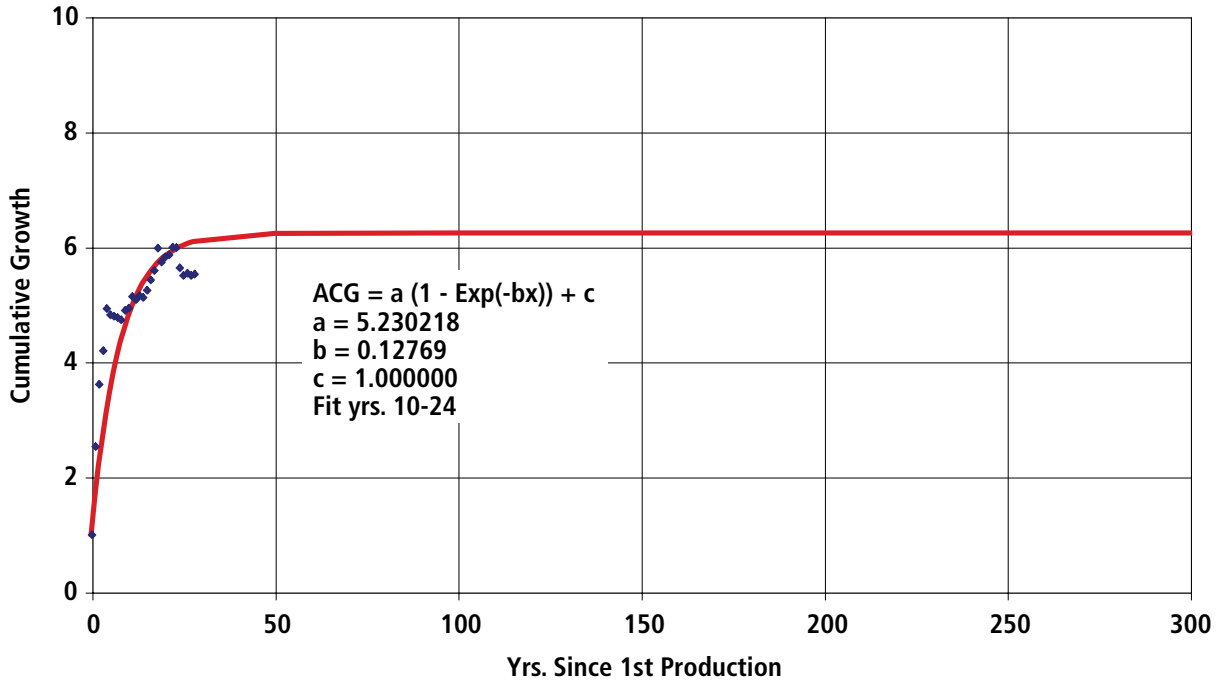
Figure A7-15. Wyoming Thrust Belt Exponential Curve Fit of Oil Equivalent Cumulative Growth Factor
