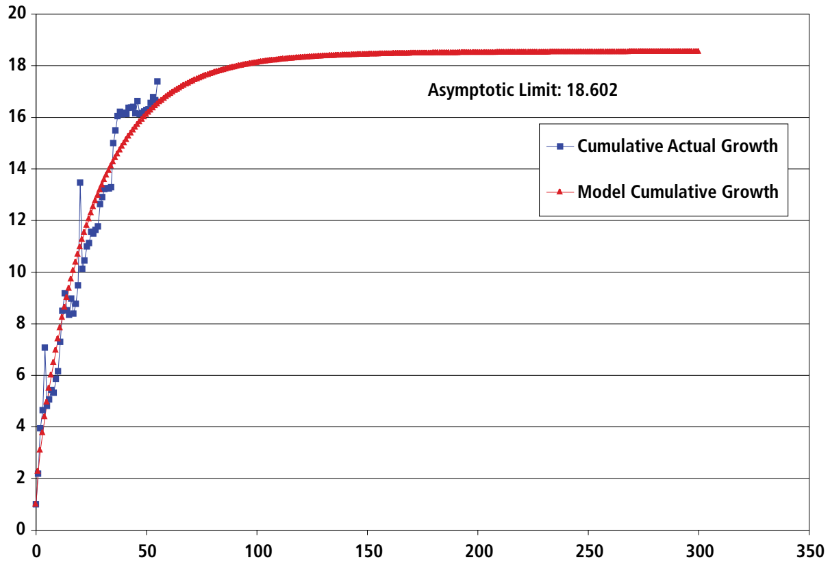
Figure A7-27. Uinta/Piceance Basin Liquids Fields Model Fit
