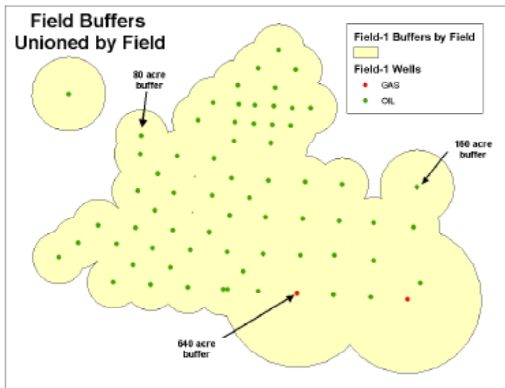
Figure A8-4. Field Buffers by Field
