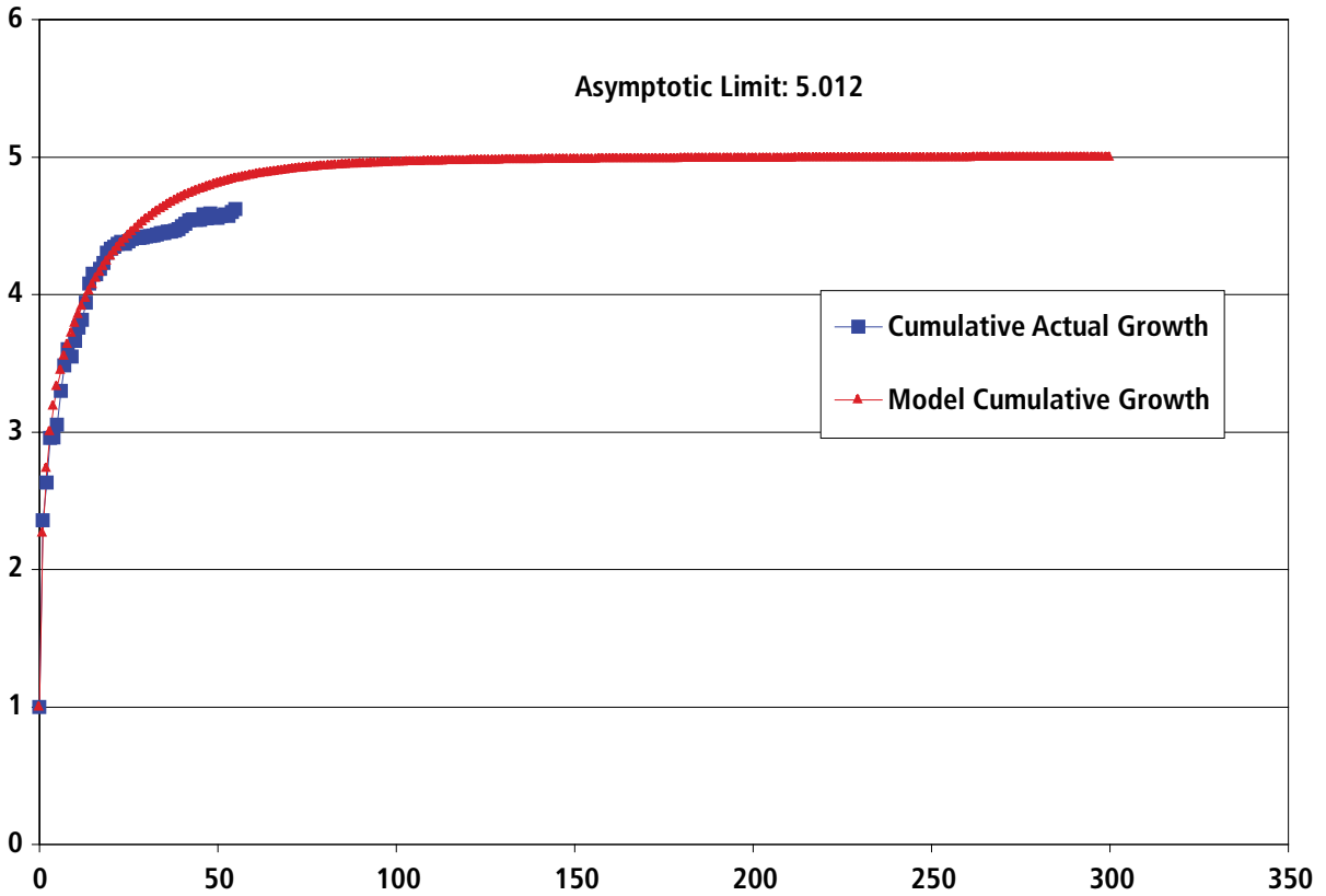
Figure A7-37. Denver Basin Liquids Fields Model Fit
