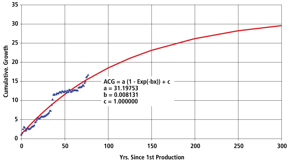
Figure A7-1. Uinta-Piceance Basin Exponential Curve Fit of Equivalent Oil Cumulative Growth Factor
