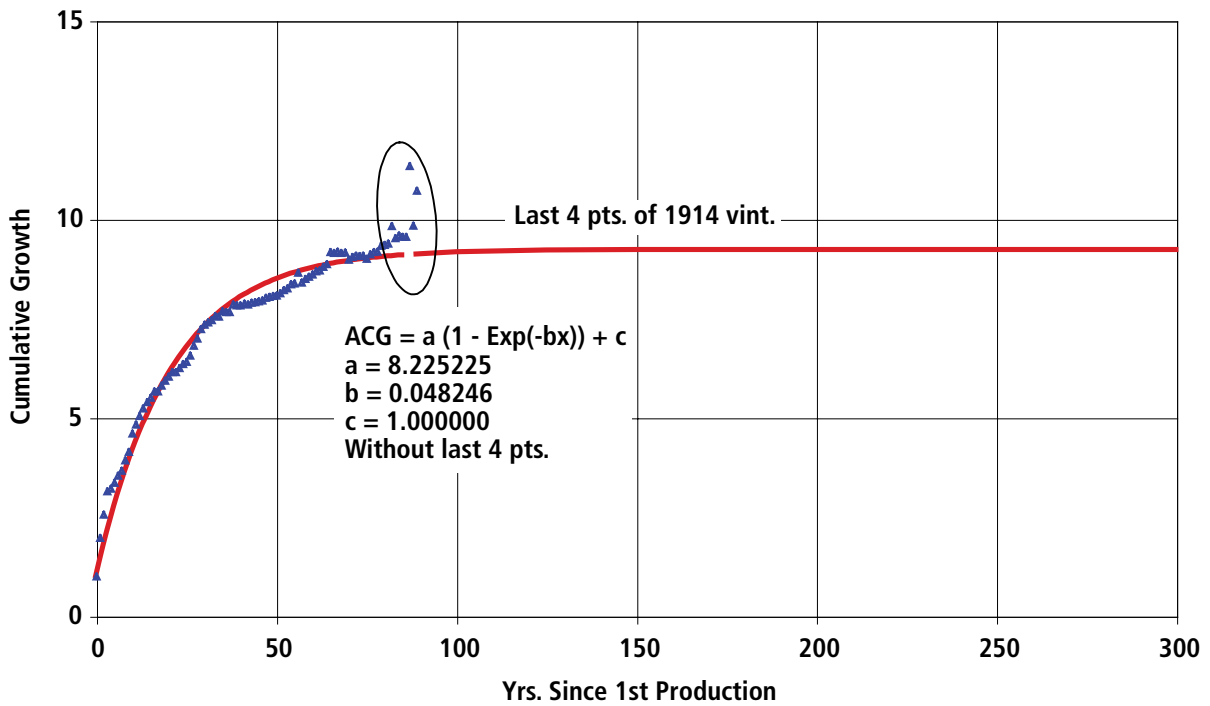
Figure A7-12. Powder River Basin Exponential Curve Fit of Equivalent Oil Cumulative Growth Factor
