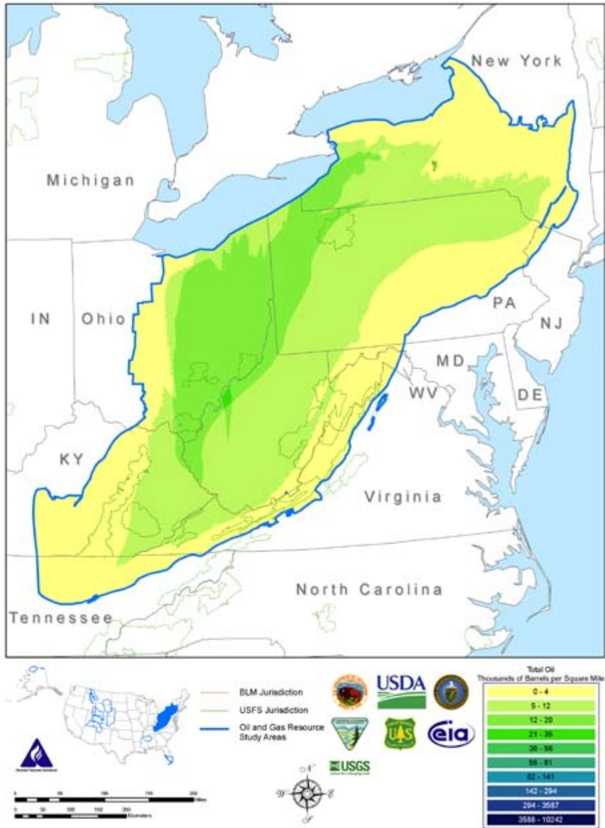
Figure 2-24. Total Oil Map, Appalachian Basin Study Area
