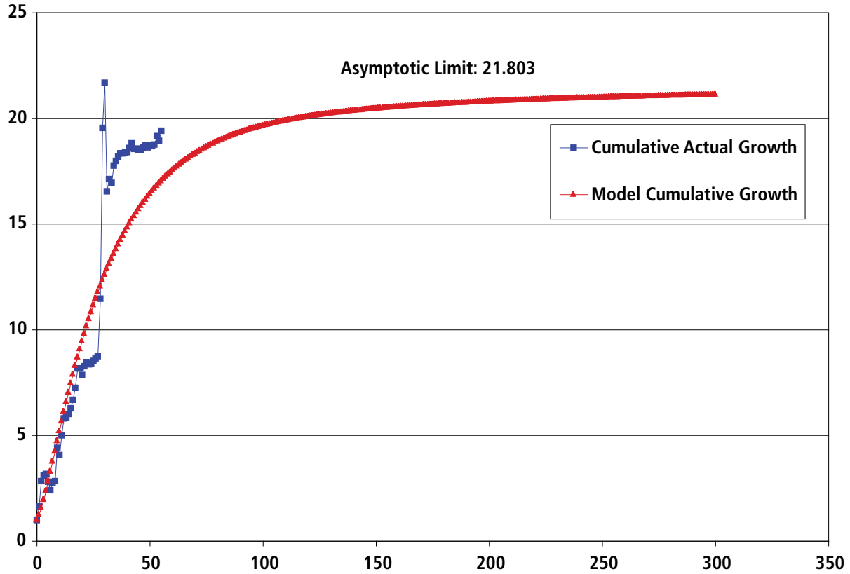
Figure A7-28. Uinta/Piceance Basin Gas Fields Model Fit
