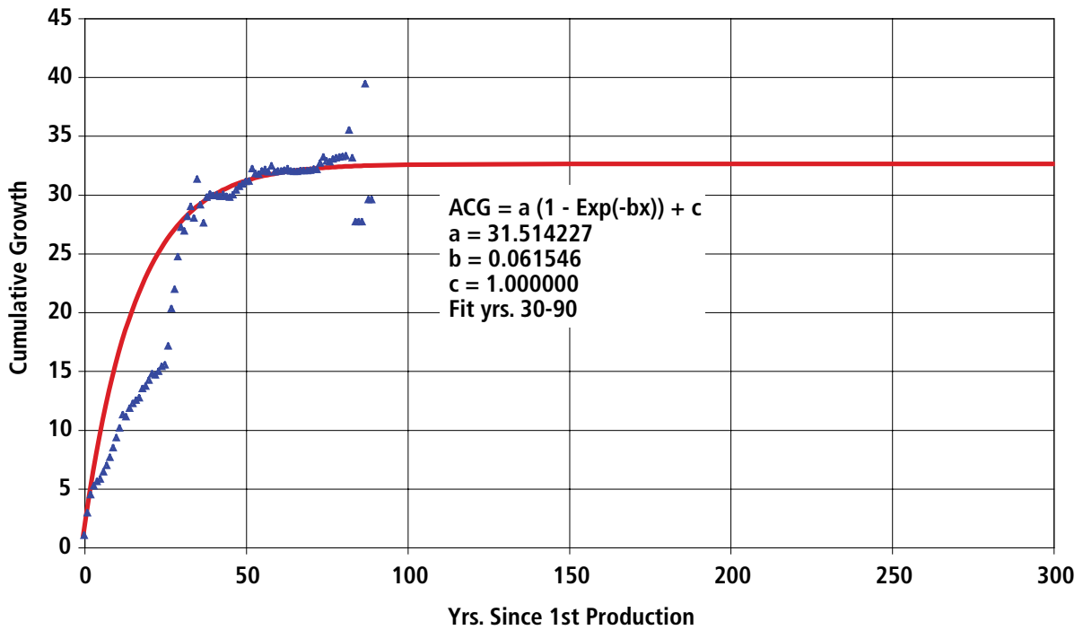
Figure A7-14. Powder River Basin Exponential Curve Fit of Gas Cumulative Growth Factor
