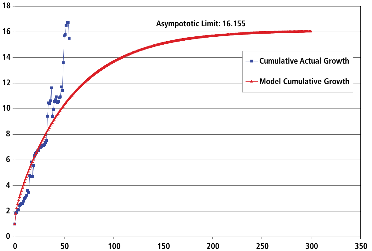
Figure A7-29. Paradox/San Juan Basins Liquids Fields Model Fit
