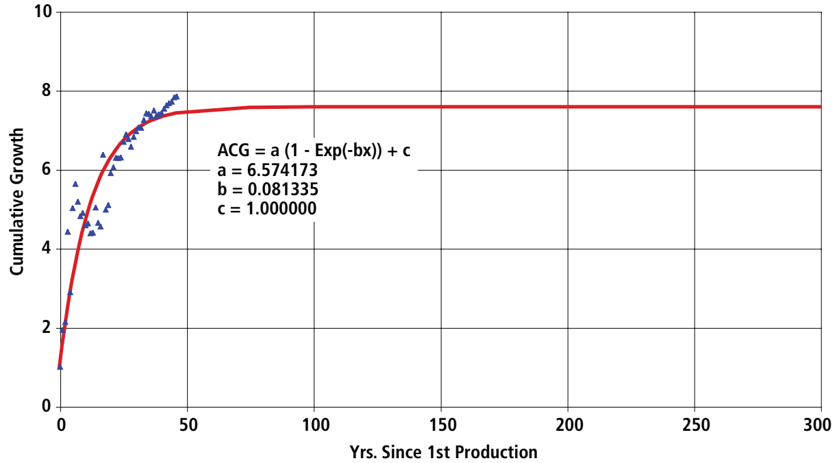
Figure A7-5. Uinta-Piceance Basin Exponential Curve Fit of Tight Formation Gas Cumulative Growth Factor
