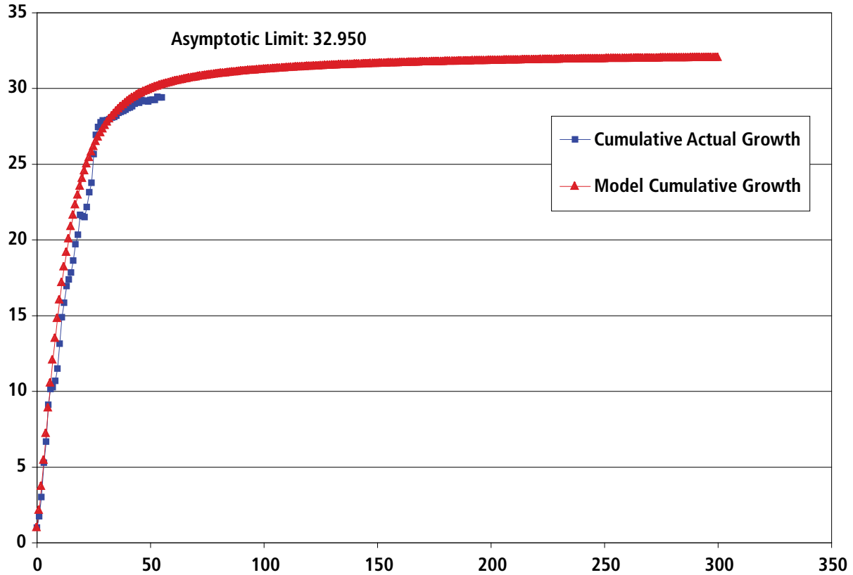
Figure A7-35. Greater Green River Basin Liquids Fields Model Fit
