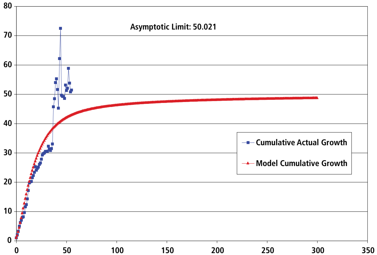
Figure A7-36. Greater Green River Basin Gas Fields Model Fit
