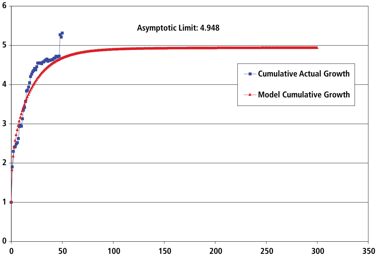
Figure A7-38. Denver Basin Gas Fields Model Fit
