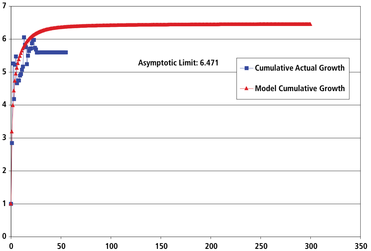
Figure A7-33. Wyoming Thrust Belt Liquids Fields Model Fit
