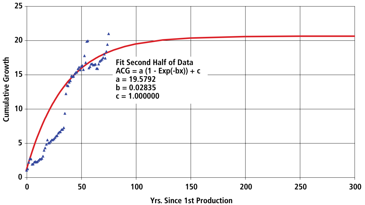
Figure A7-4. Uinta-Piceance Basin Exponential Curve Fit of Gas Cumulative Growth Factor
