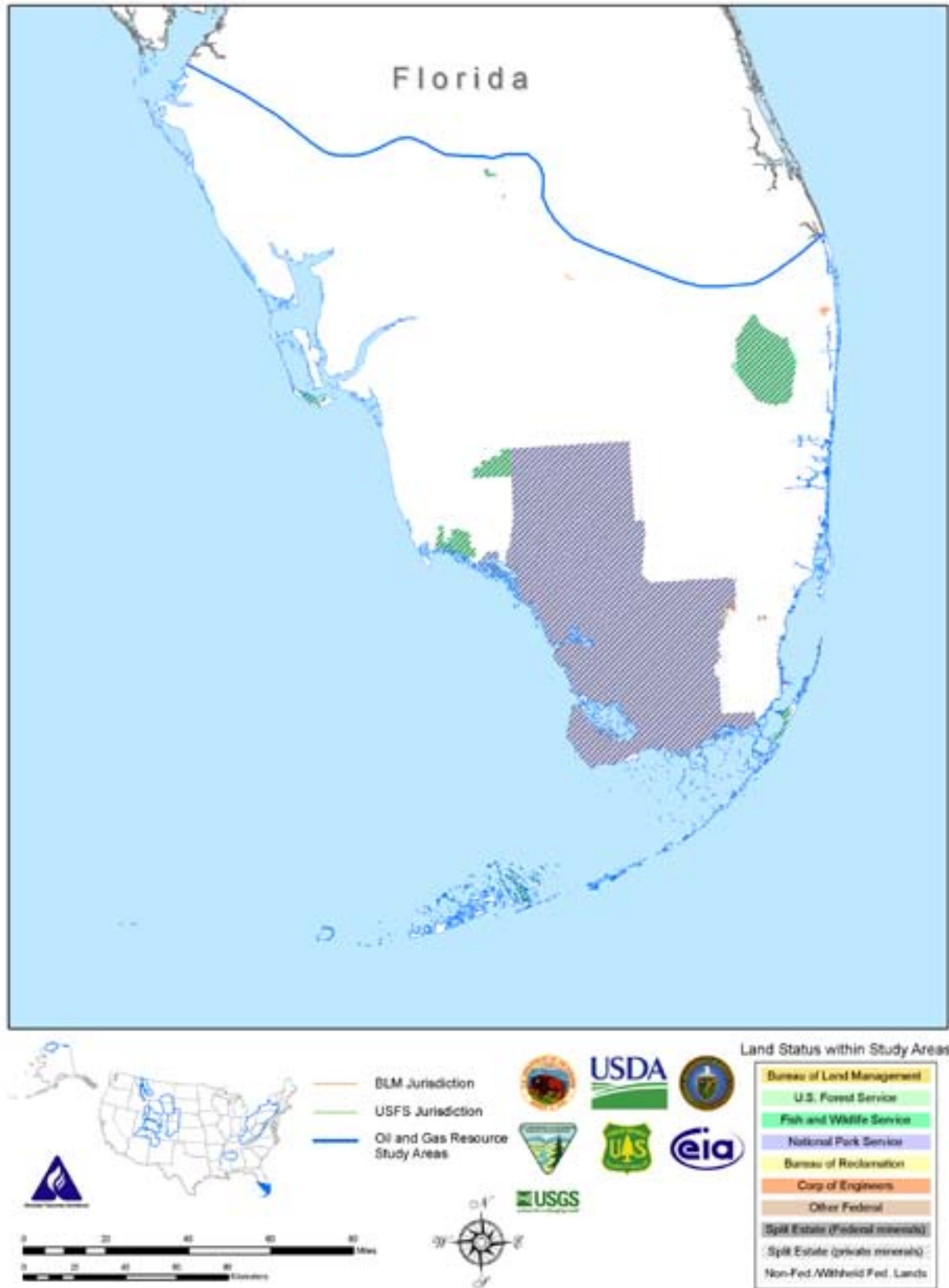
Figure 2-9. Federal Land Status Map, Florida Peninsula Study Area
