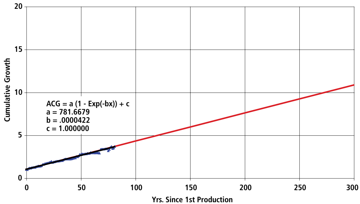
Figure A7-6. Paradox/San Juan Basins Exponential Curve Fit of Equivalent Oil Cumulative Growth Factor
