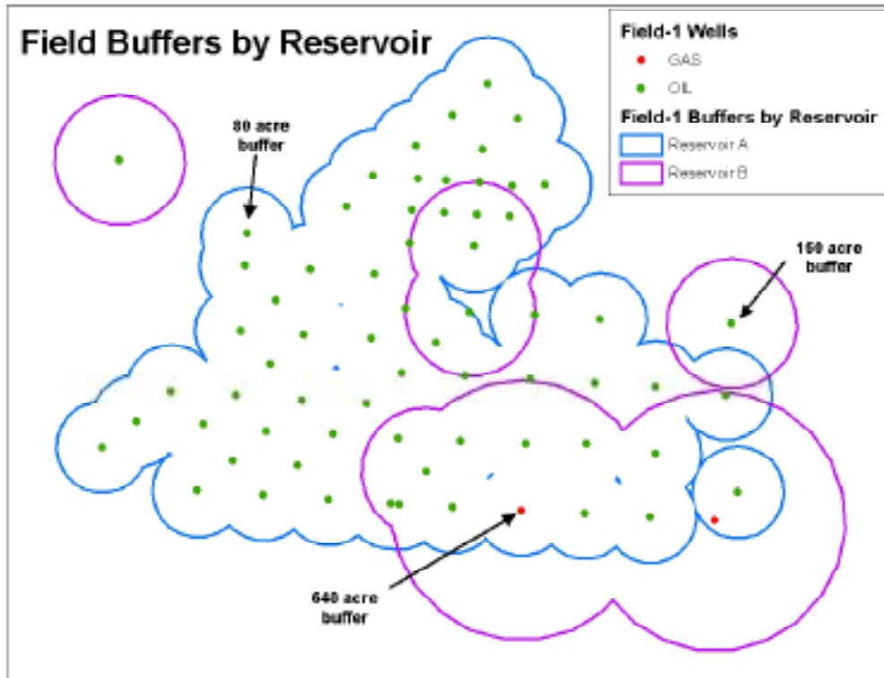
Figure A8-3. Field Buffers by Reservoir
