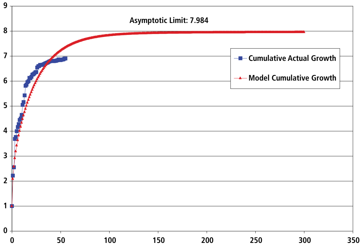
Figure A7-31. Powder River Basin Liquids Fields Model Fit
