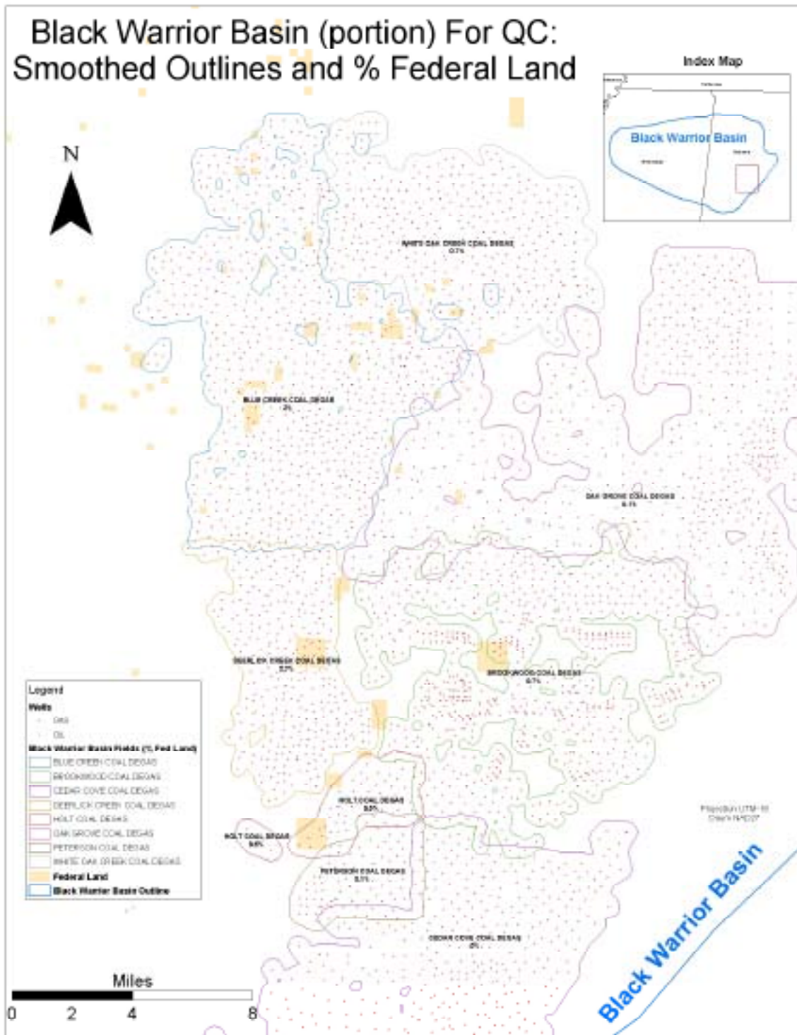
Figure A8-8. Black Warrior Basin Quality Check Map Showing Smoothed Field Outlines and Percent Federal Land
