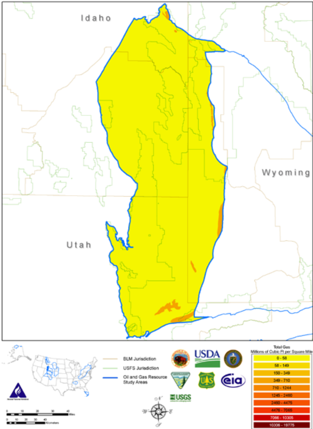
Figure 2-30. Total Natural Gas Map, Wyoming Thrust Belt Study Area
