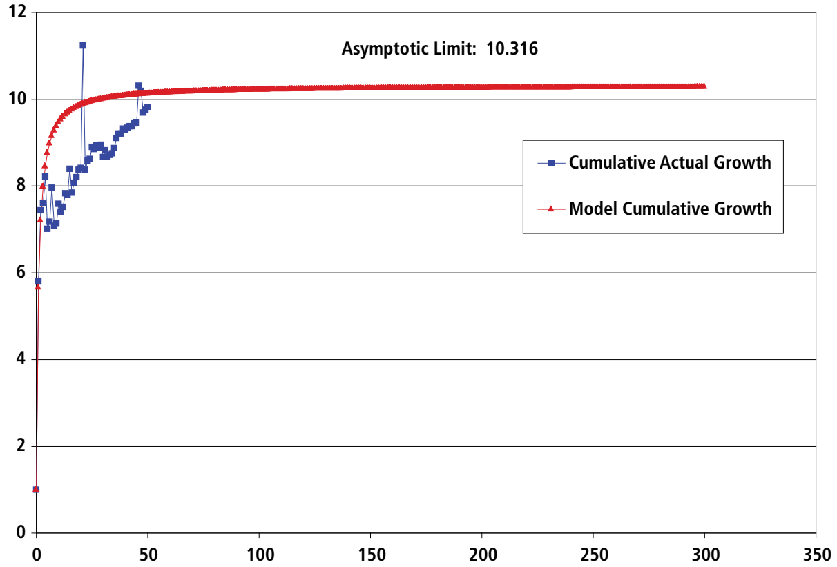
Figure A7-39. Black Warrior Basin Liquids Fields Model Fit
