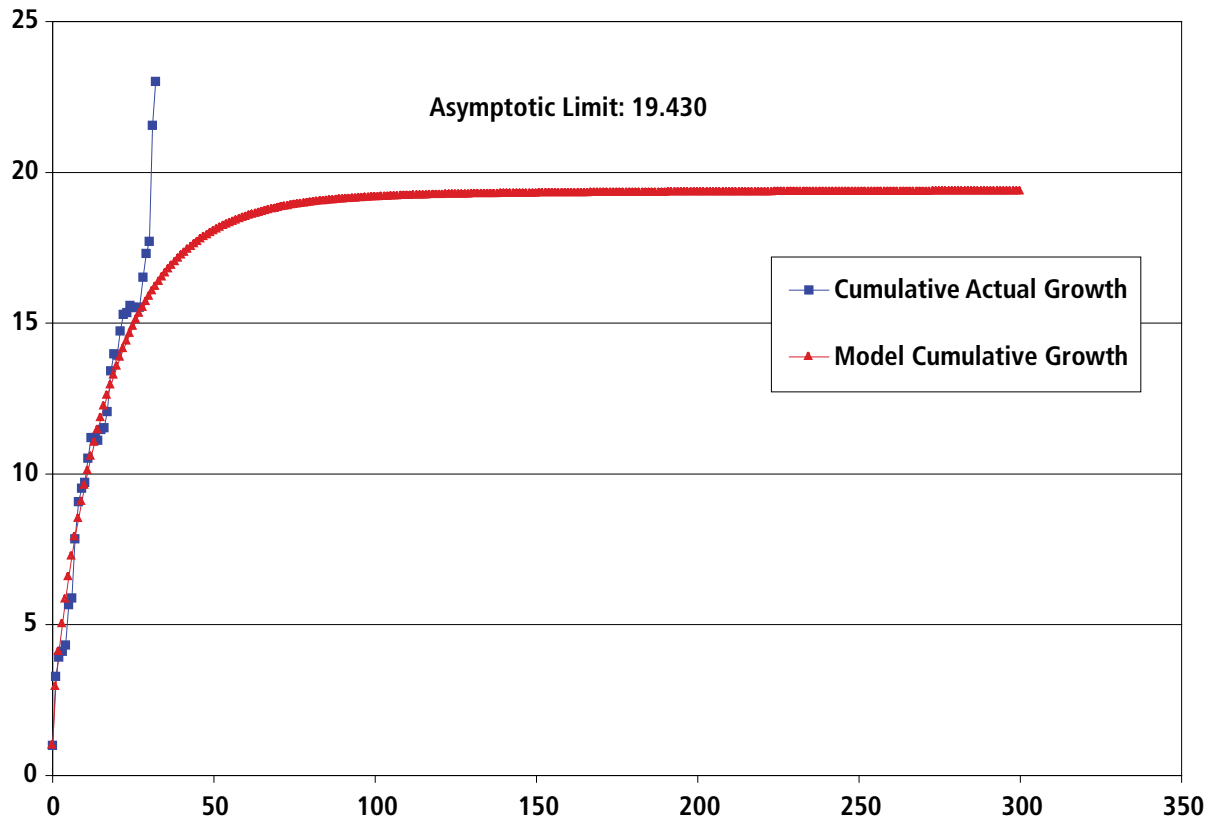
Figure A7-40. Black Warrior Basin Gas Fields Model Fit
