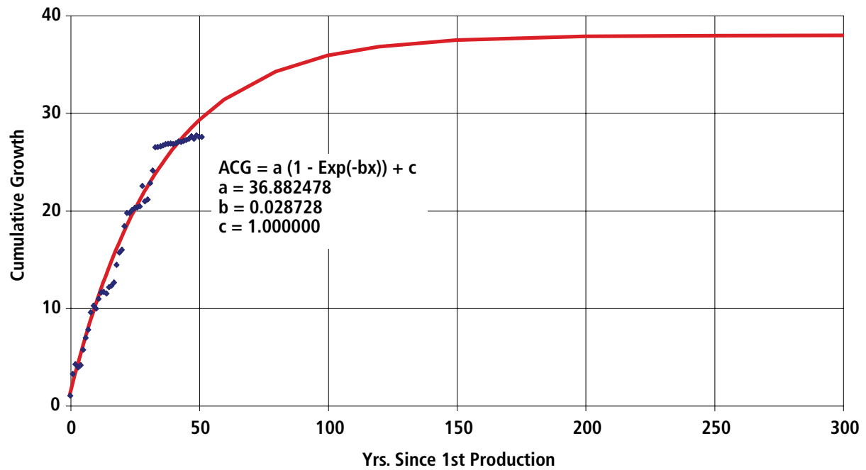
Figure A7-26. Black Warrior Basin Exponential Curve Fit of Gas Cumulative Growth Factor
