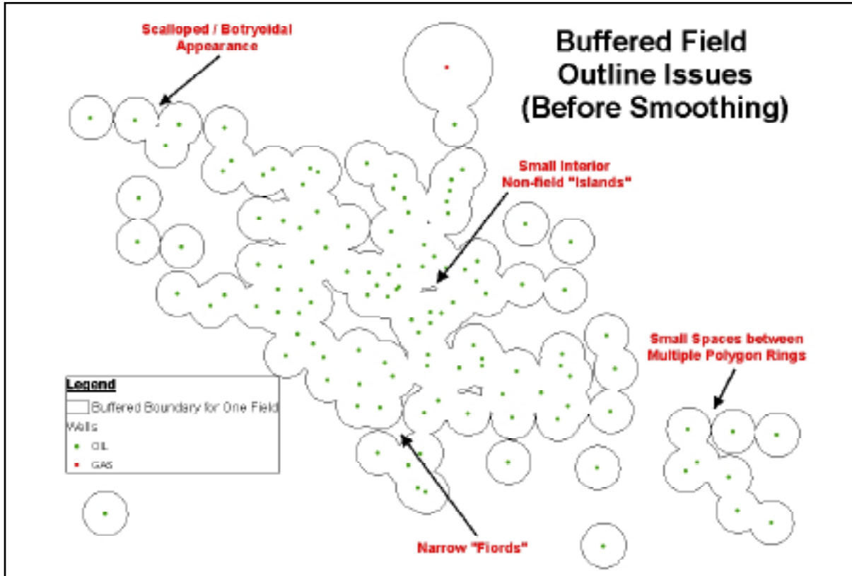
Figure A8-5. Buffered Field Outline Issues
