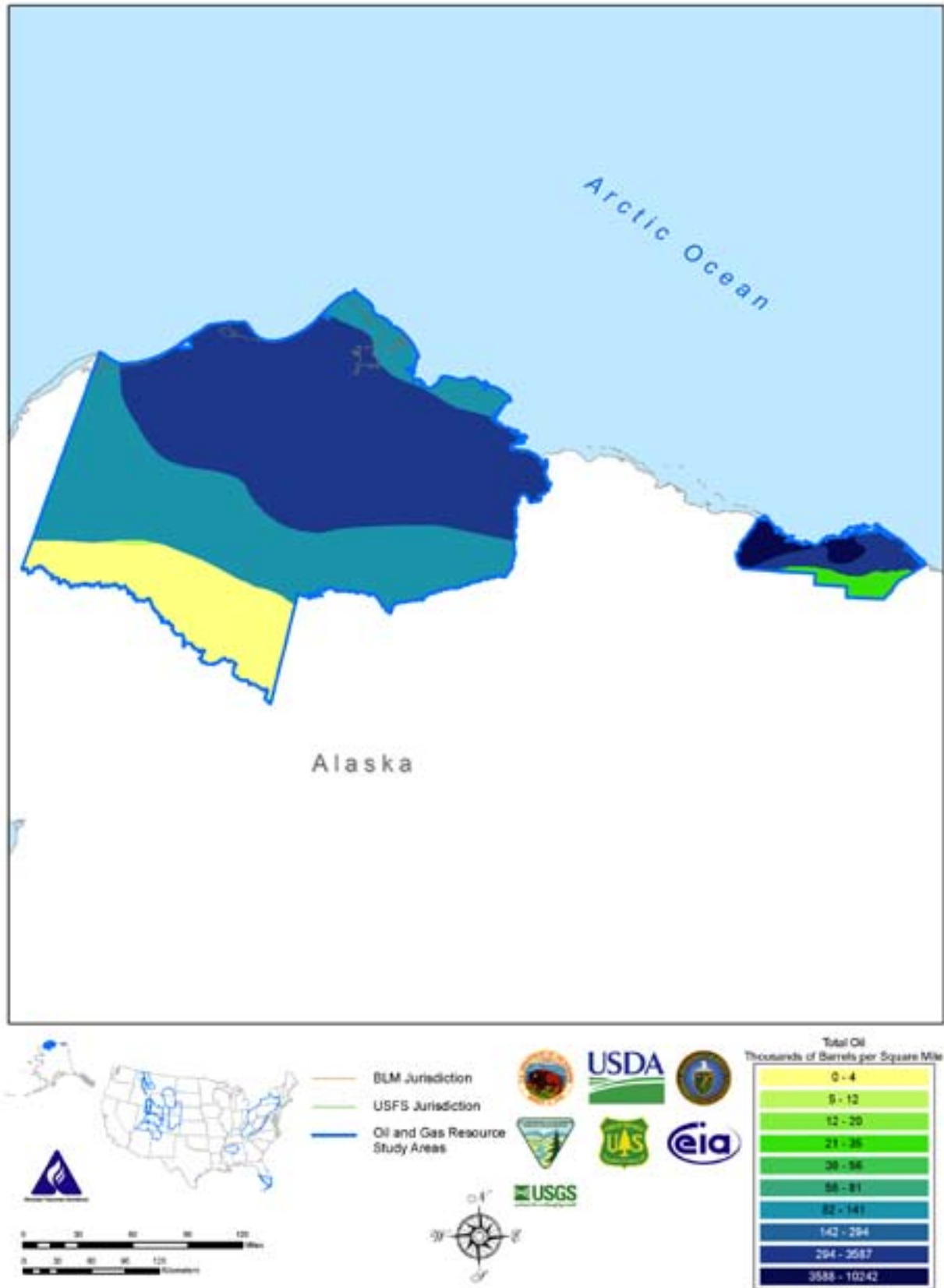
Figure 2-14. Total Oil Map, Northern Alaska Study Area
