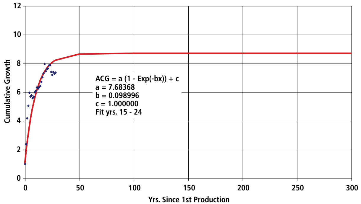
Figure A7-17. Wyoming Thrust Belt Exponential Curve Fit of Gas Cumulative Growth Factor
