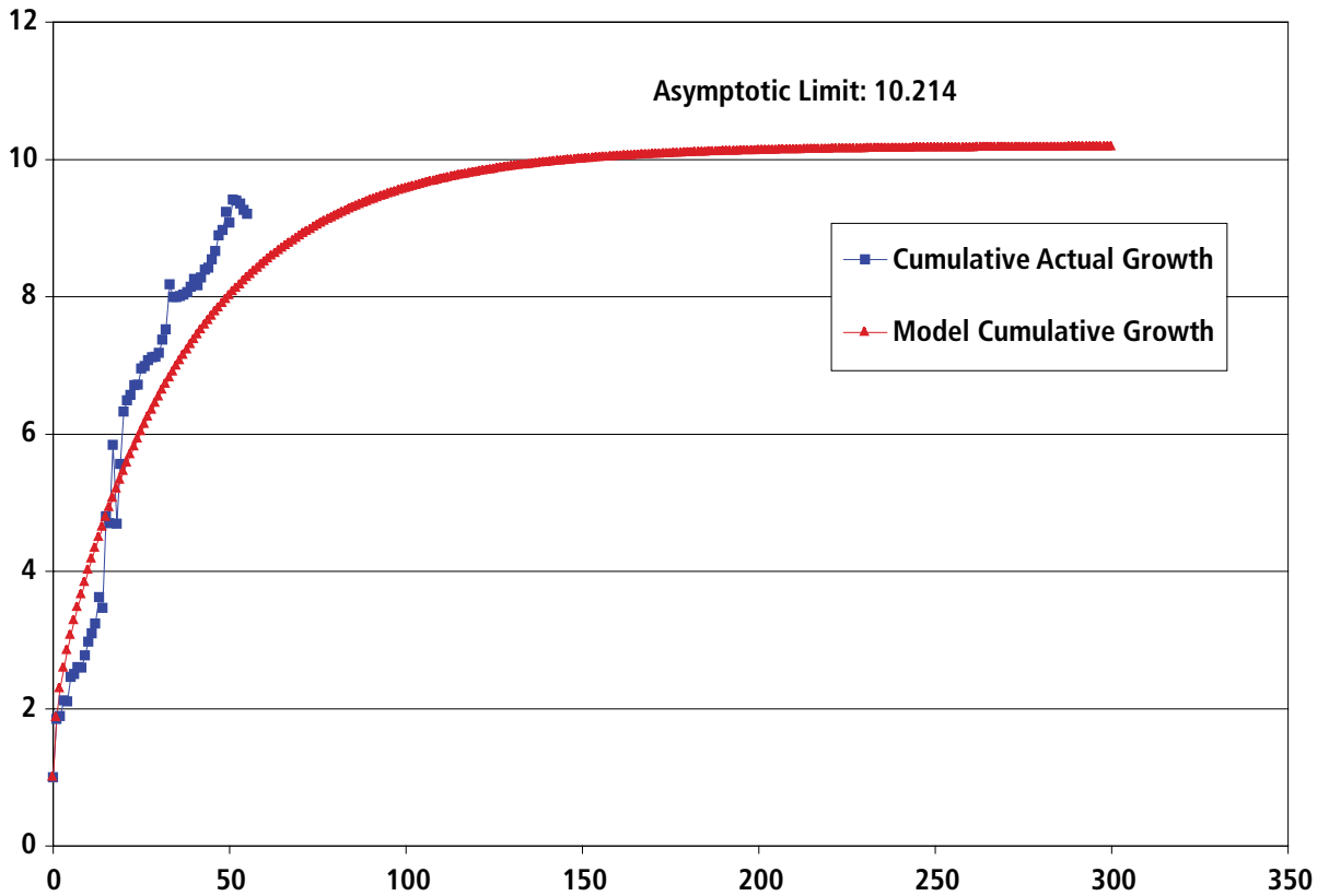
Figure A7-30. Paradox/San Juan Basins Gas Fields Model Fit (Coalbed Natural Gas Not Included)
