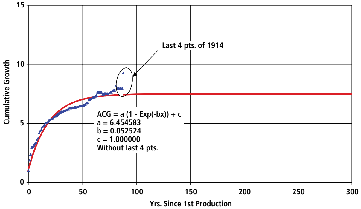
Figure A7-13. Powder River Basin Exponential Curve Fit of Liquids Cumulative Growth Factor
