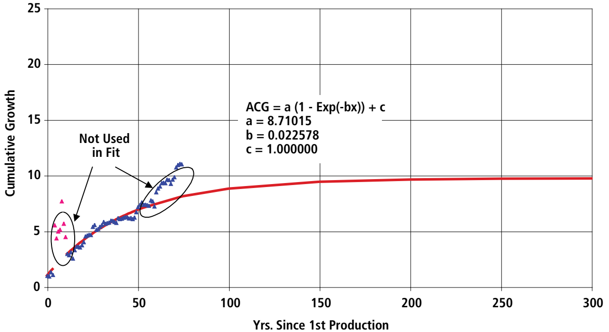
Figure A7-11. Paradox/San Juan Basins Exponential Curve Fit of Tight Formation Gas Cumulative
