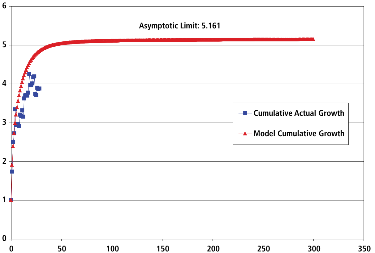
Figure A7-34. Wyoming Thrust Belt Gas Fields Model Fit
