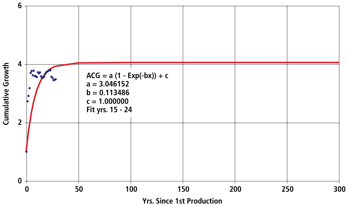
Figure A7-16. Wyoming Thrust Belt Exponential Curve Fit of Liquids Cumulative Growth Factor
