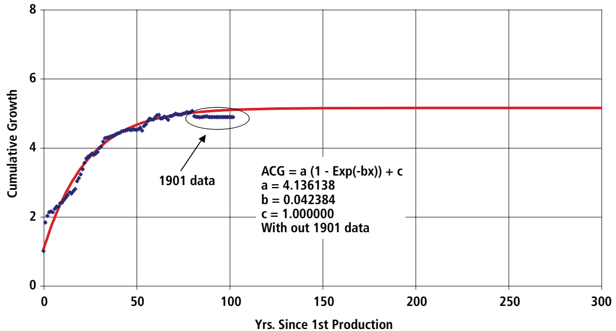
Figure A7-22. Denver Basin Exponential Curve Fit of Liquids Cumulative Growth Factor
