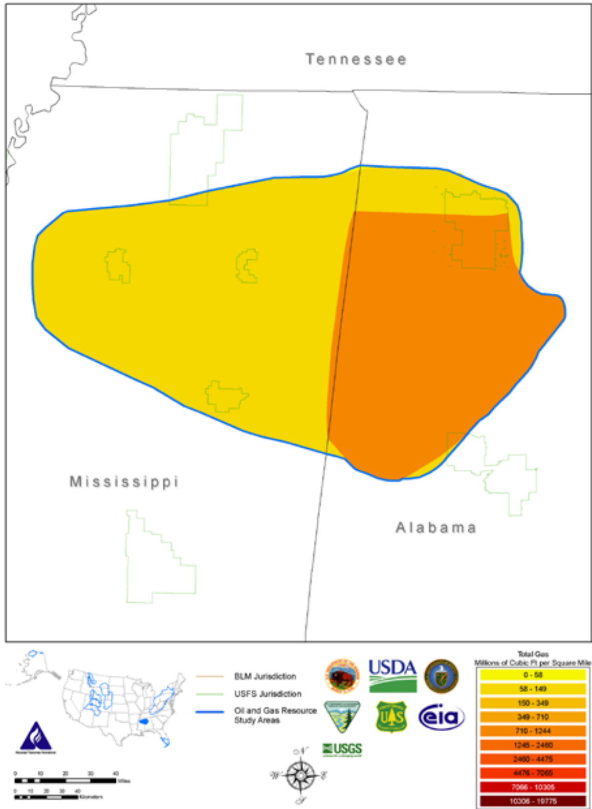
Figure 2-34. Total Natural Gas Map, Black Warrior Basin Study Area
