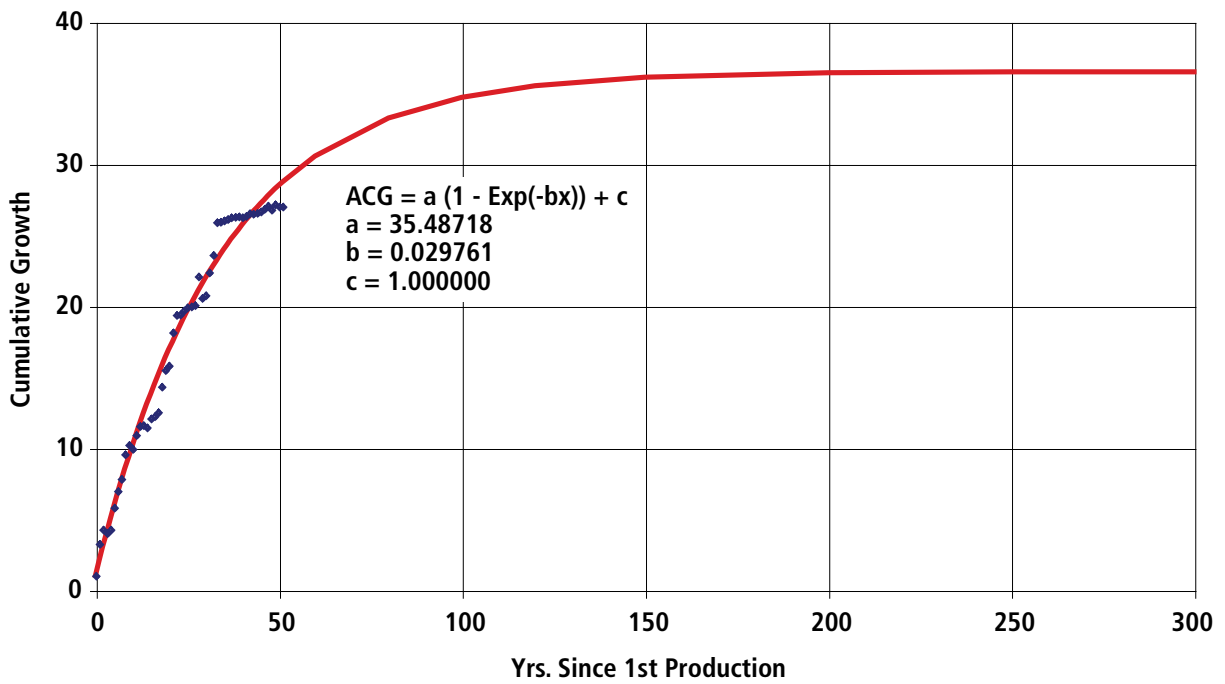
Figure A7-24. Black Warrior Basin Exponential Curve Fit of Oil Equivalent Cumulative Growth
