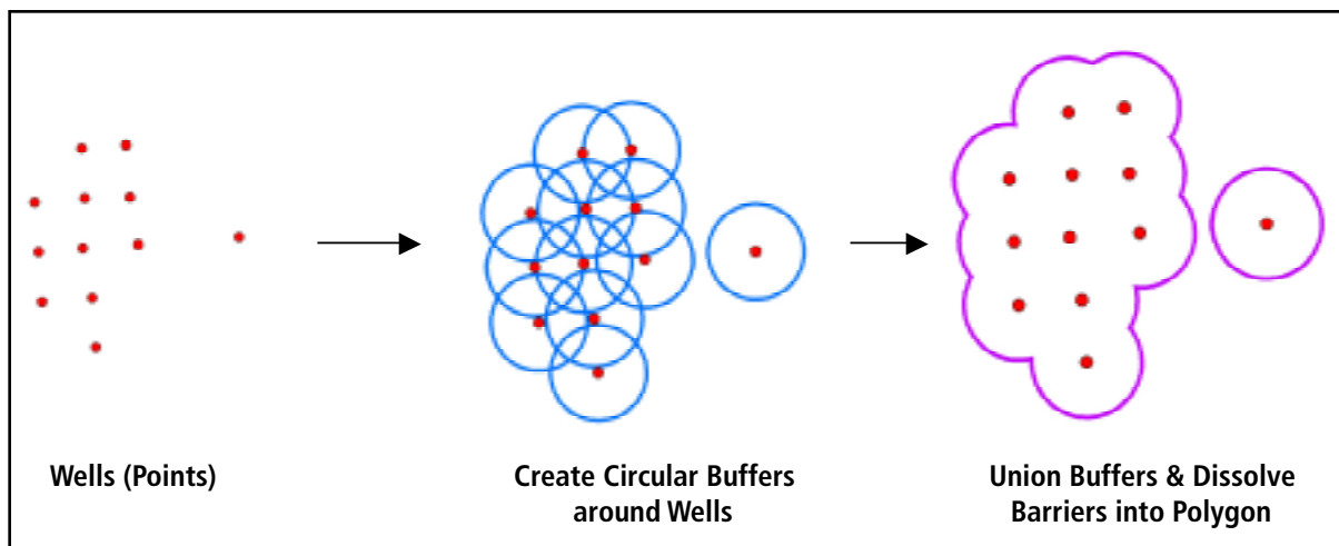
Figure A8-2. Buffering Process
