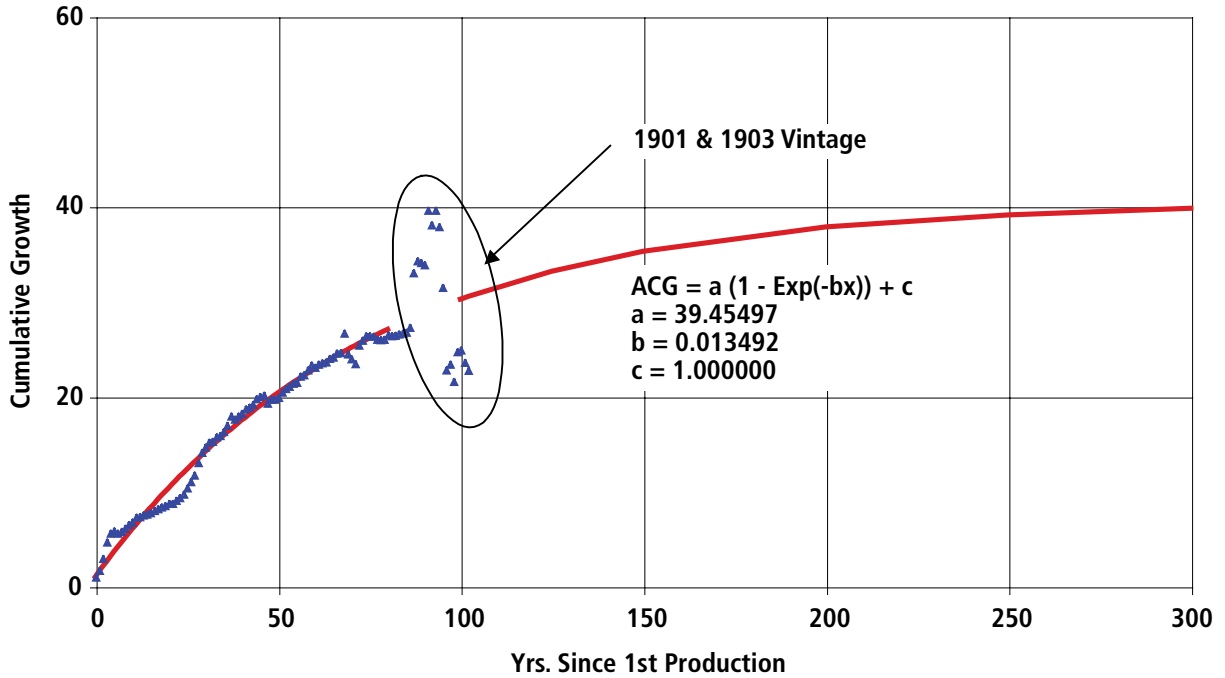
Figure A7-19. Greater Green River Basin Exponential Curve Fit of Liquids Cumulative Growth Factor
