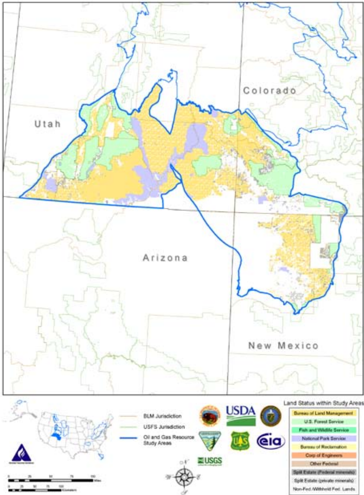
Figure 2-3. Federal Land Status Map, Paradox/San Juan Basins Study Area
