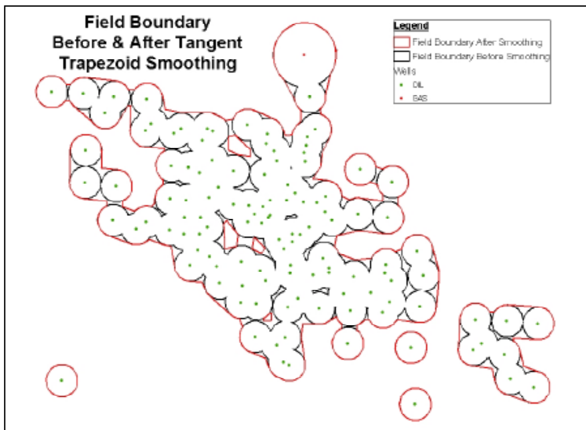
Figure A8-7. Field Boundary Before and after Smoothing with Tangent Trapezoid Technique
