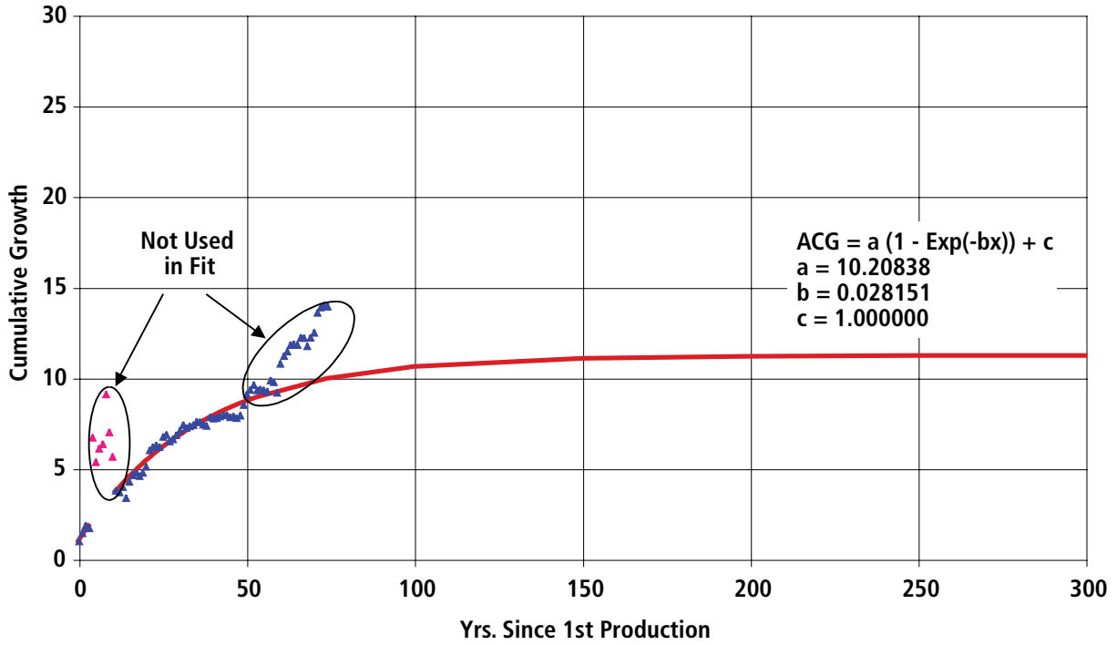
Figure A7-7. Paradox/San Juan Basins Exponential Curve Fit of Tight Formation Equivalent Oil Cumulative Growth Factor
