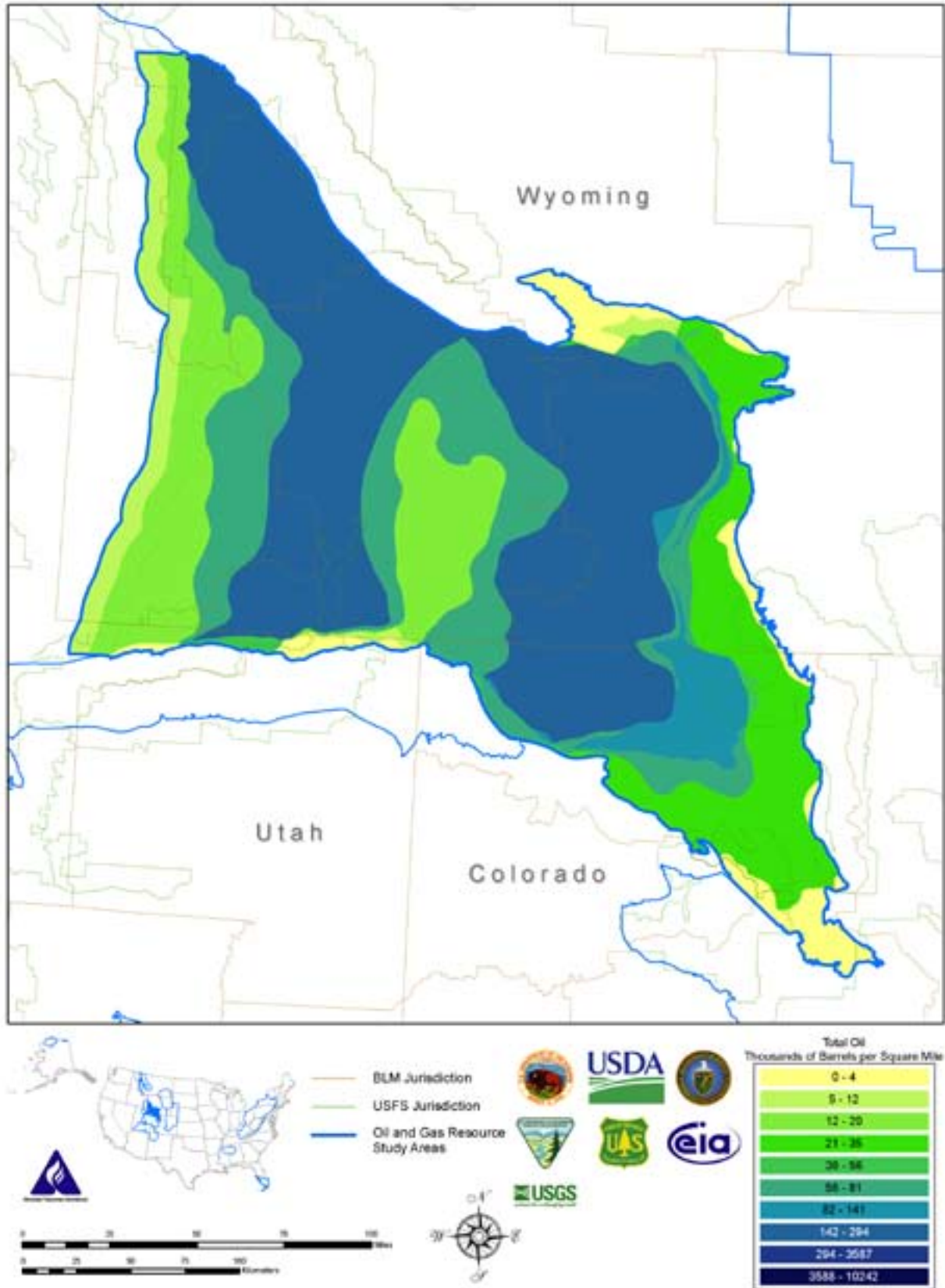
Figure 2-20. Total Oil Map, Greater Green River Basin Study Area
