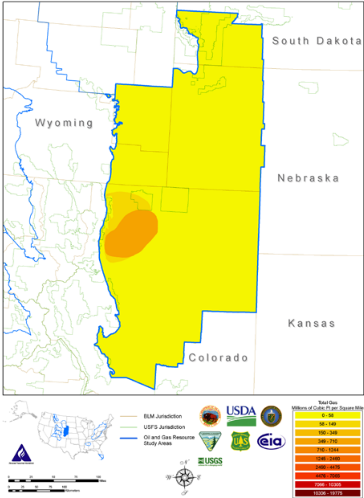
Figure 2-32. Total Natural Gas Map, Denver Basin Study Area
