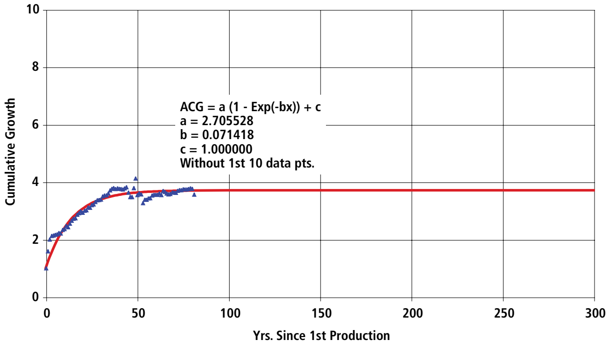
Figure A7-8. Paradox/San Juan Basins Exponential Curve Fit of Liquids Cumulative Growth Factor
