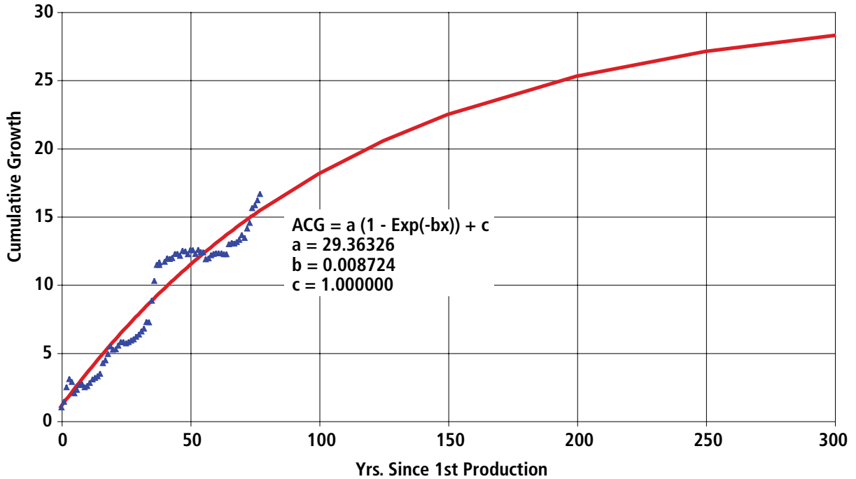
Figure A7-3. Uinta-Piceance Basin Exponential Curve Fit of Liquids Cumulative Growth Factor
