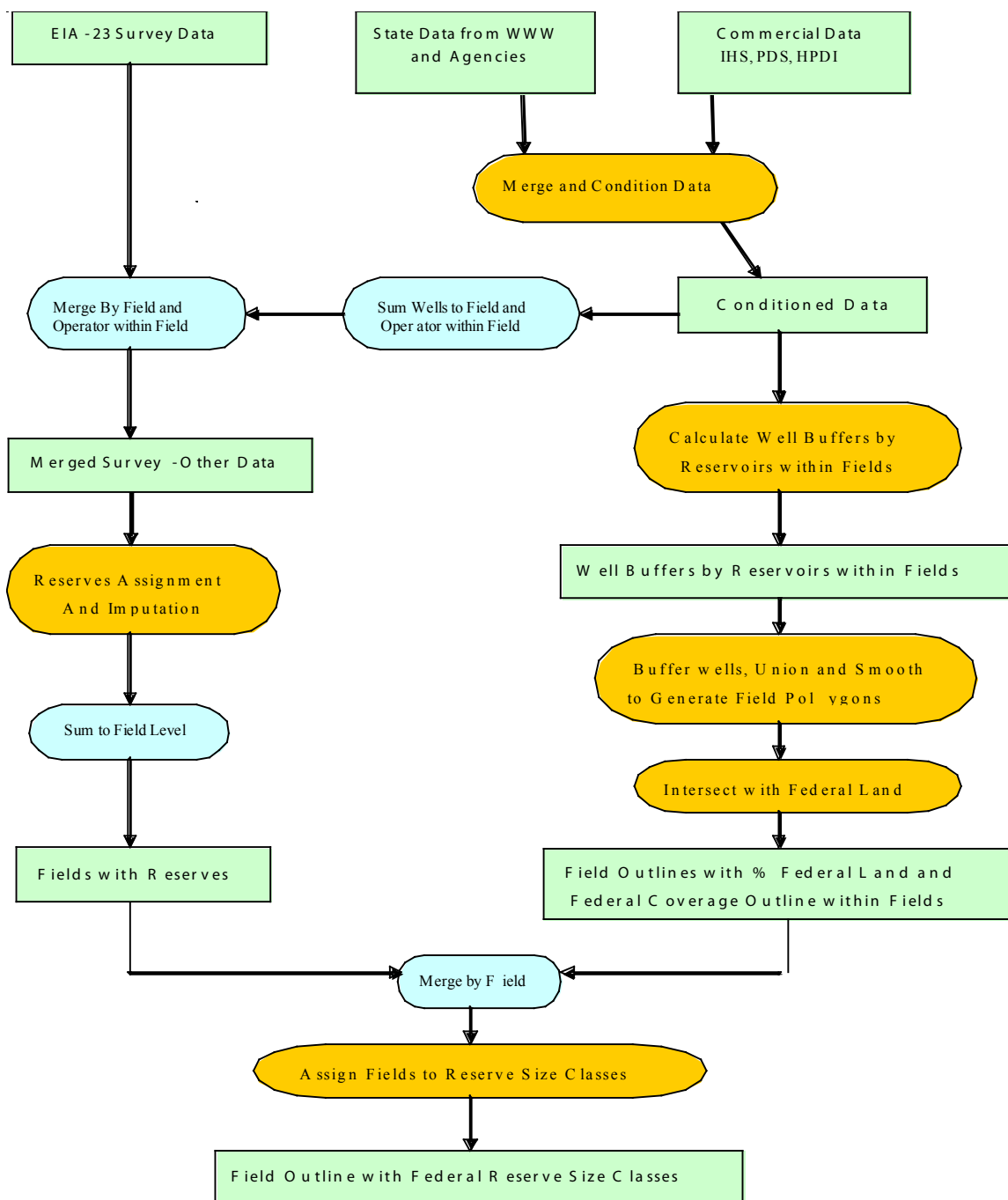
Figure A8-1. Phase II Process Flows
