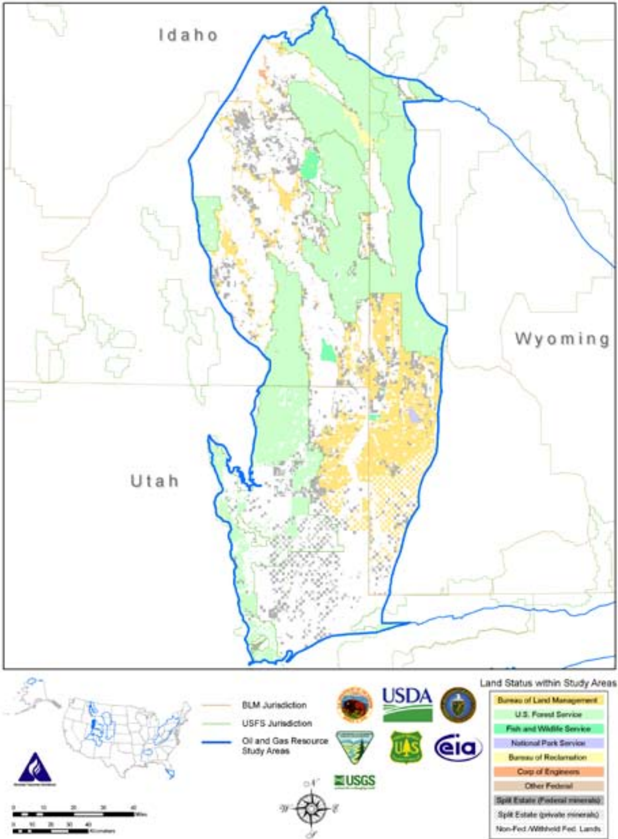
Figure 2-6. Federal Land Status Map, Wyoming Thrust Belt Study Area
