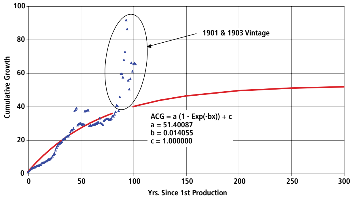
Figure A7-18. Greater Green River Basin Exponential Curve Fit of Equivalent Oil Cumulative Growth Factor
