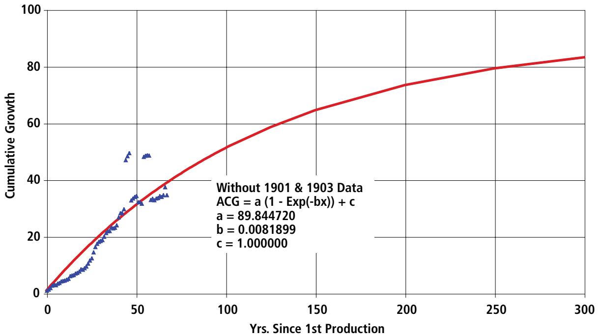
Figure A7-20. Greater Green River Basin Exponential Curve Fit of Gas Cumulative Growth Factor
