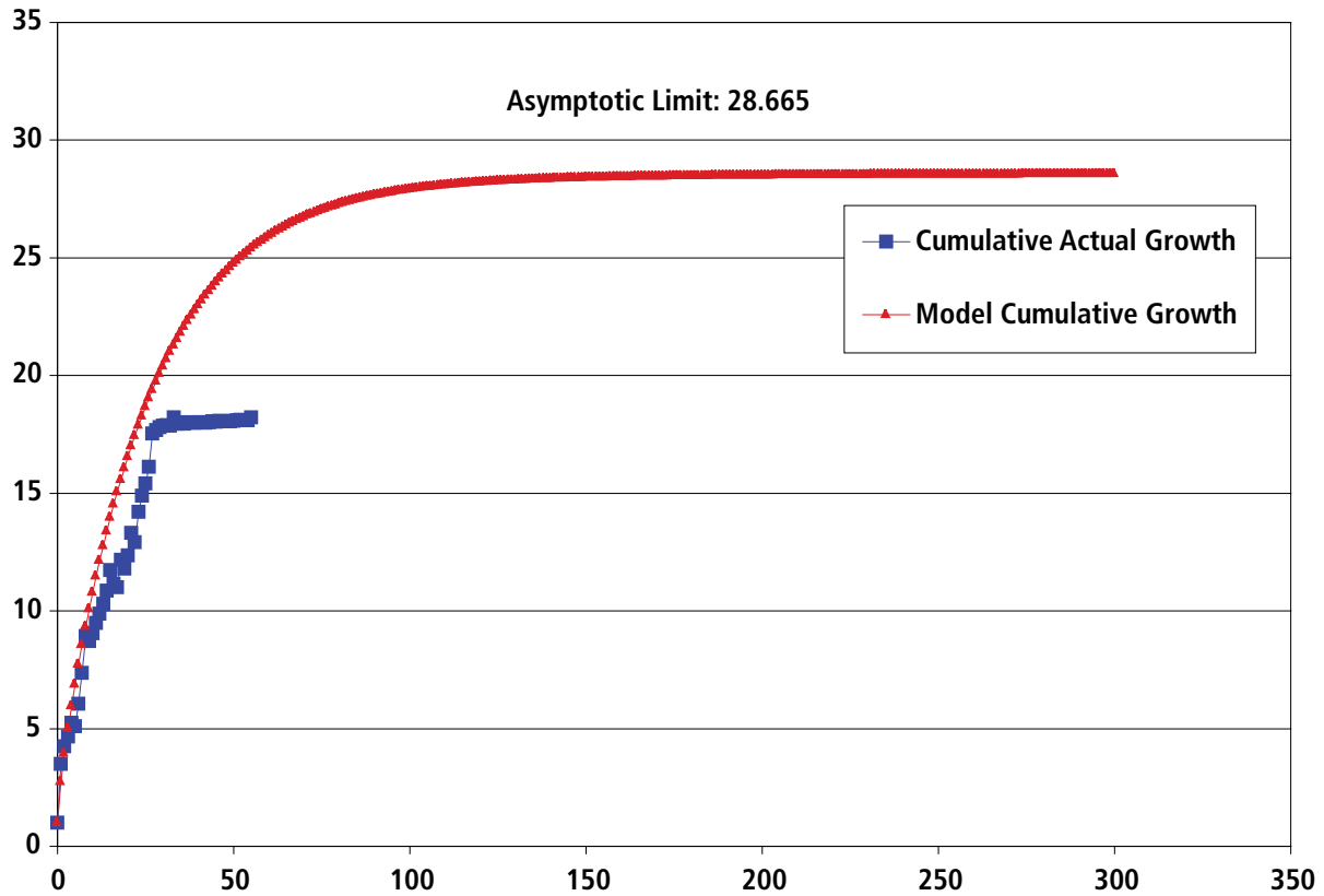
Figure A7-32. Powder River Basin Gas Fields Model Fit
