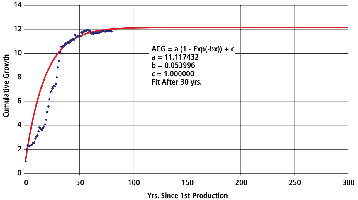
Figure A7-23. Denver Basin Exponential Curve Fit of Gas Cumulative Growth Factor
