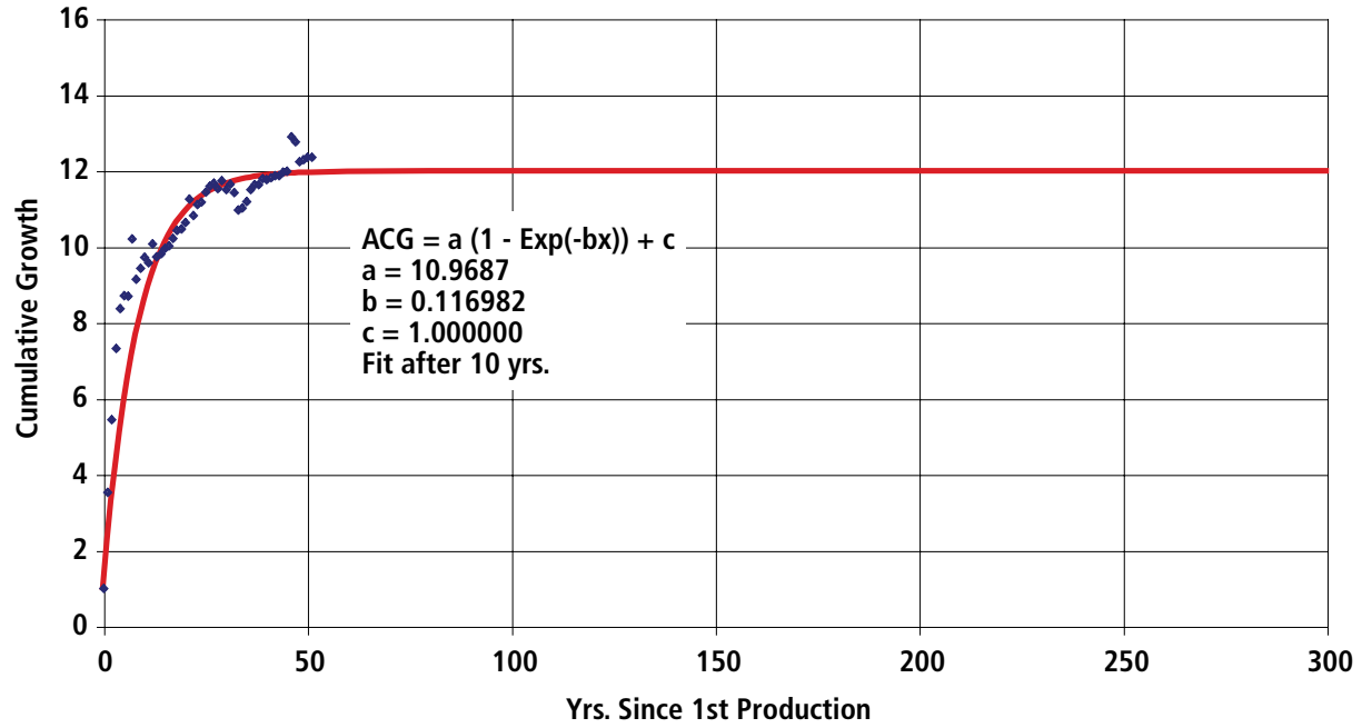
Figure A7-25. Black Warrior Basin Exponential Curve Fit of Liquids Cumulative Growth Factor
