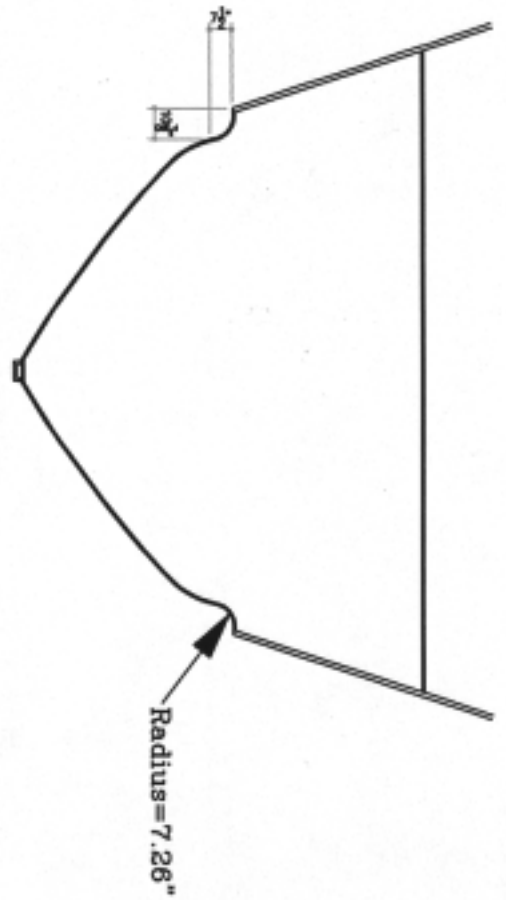
OUTER REEF 73 QUIETROLL SPRAY RAIL DIMENSIONS AND DETAILS
