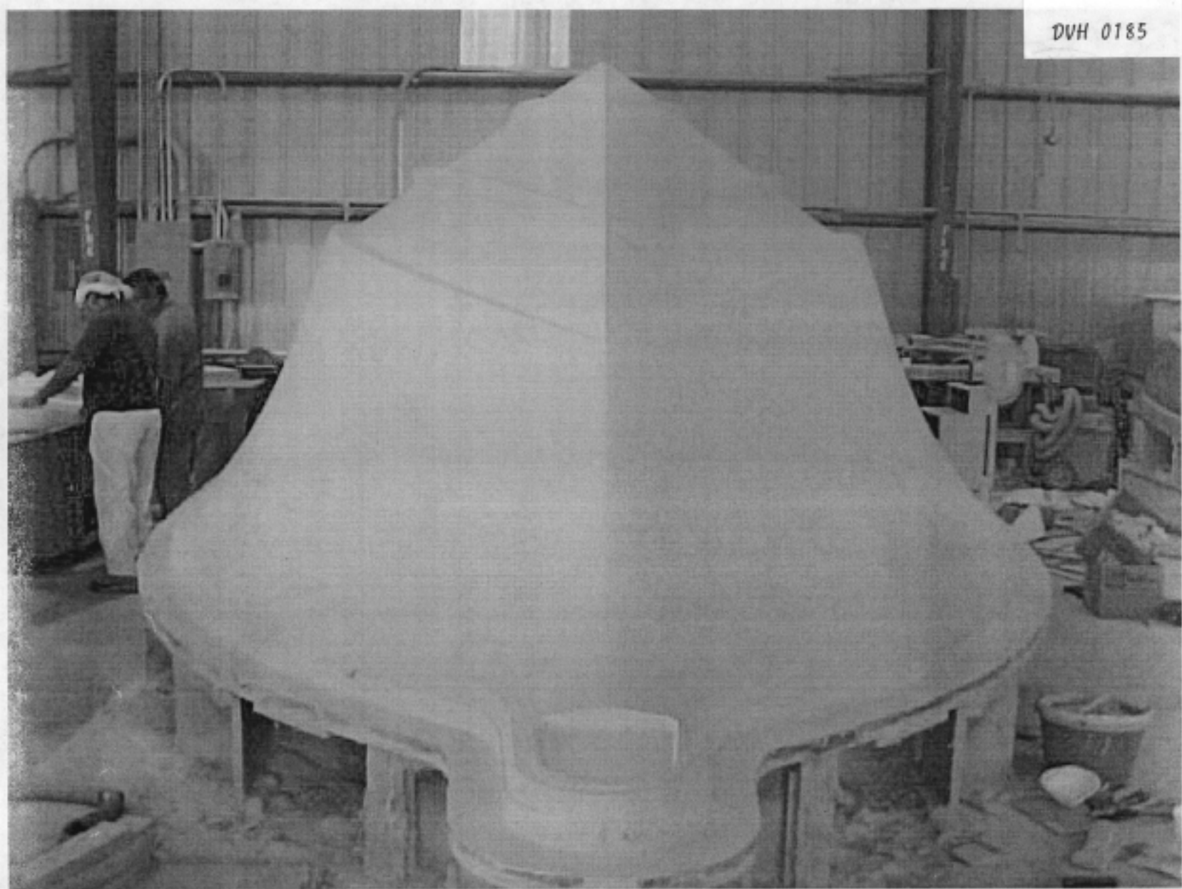
PLAN 27. CENTER CONSOLE HULL PLUG
