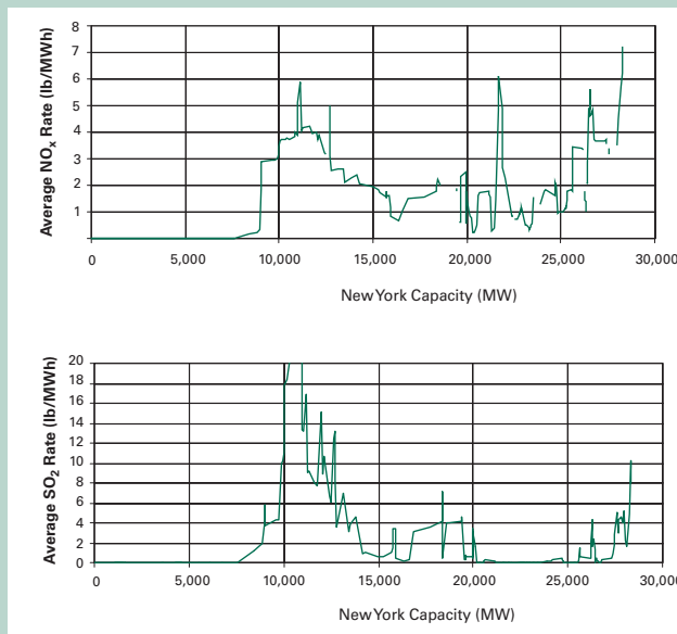
Figure 3.3.2: NO x and SO 2 Emissions by Capacity
