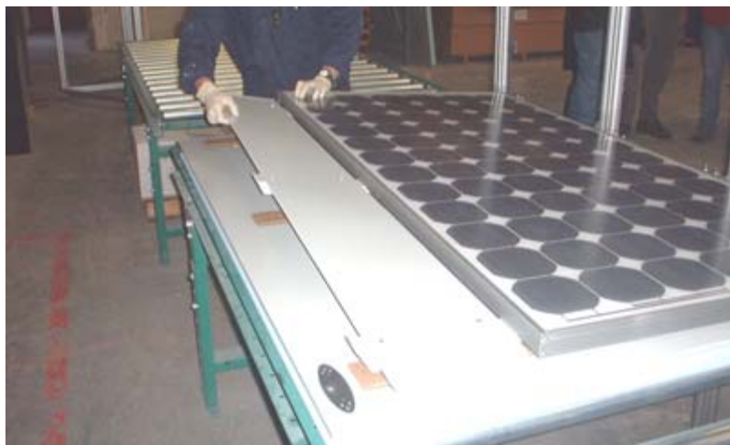
Figure 11: Completed Tile Assembly on the PL Factory Line
