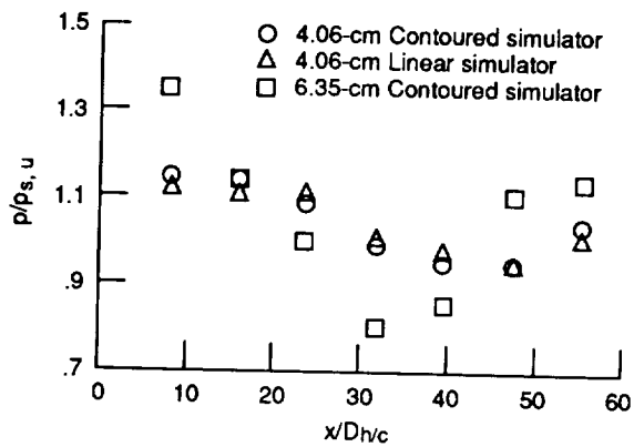
Figure 12.—Centerline static pressure distribution of isolated boundary layer simulator model at Mach 4.0.
