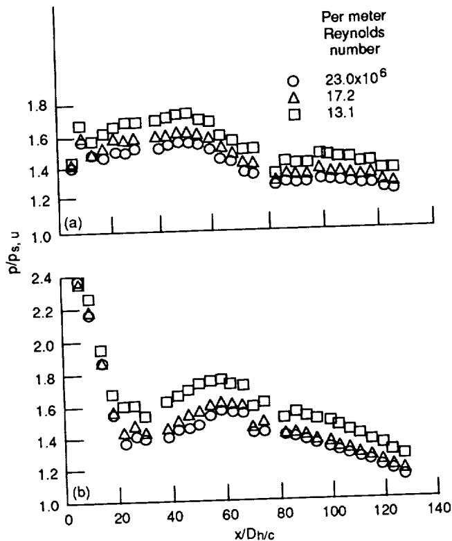
(a) 43-Percent channel height boundary layer simulator. (b) 57-Percent channel height boundary layer simulator.
