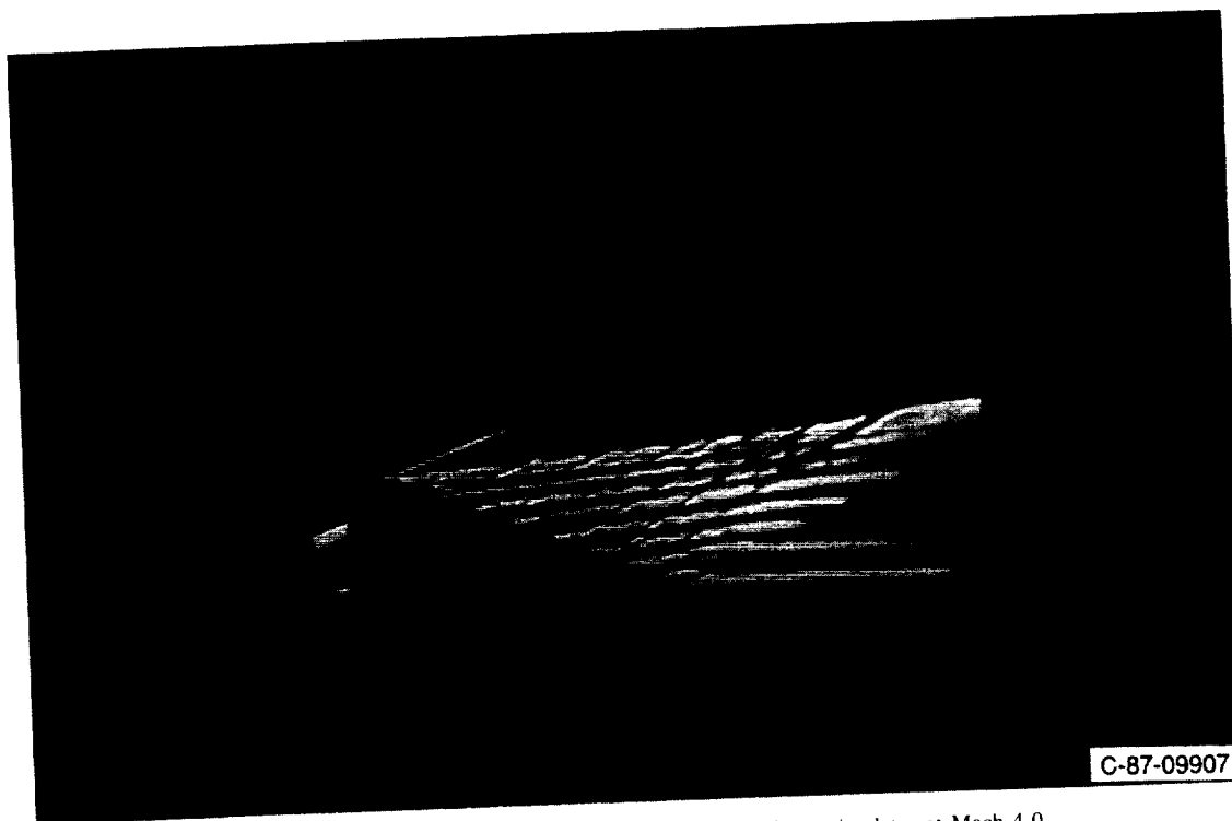
Figure 7.—Schlieren photograph of isolated boundary layer simulator at Mach 4.0.
