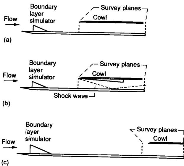
(a) Lewis channel flow model with cowl angle of 0°. (b) Lewis channel flow model with cowl angle of 4°. (c) Lewis/Langley channel flow model.
