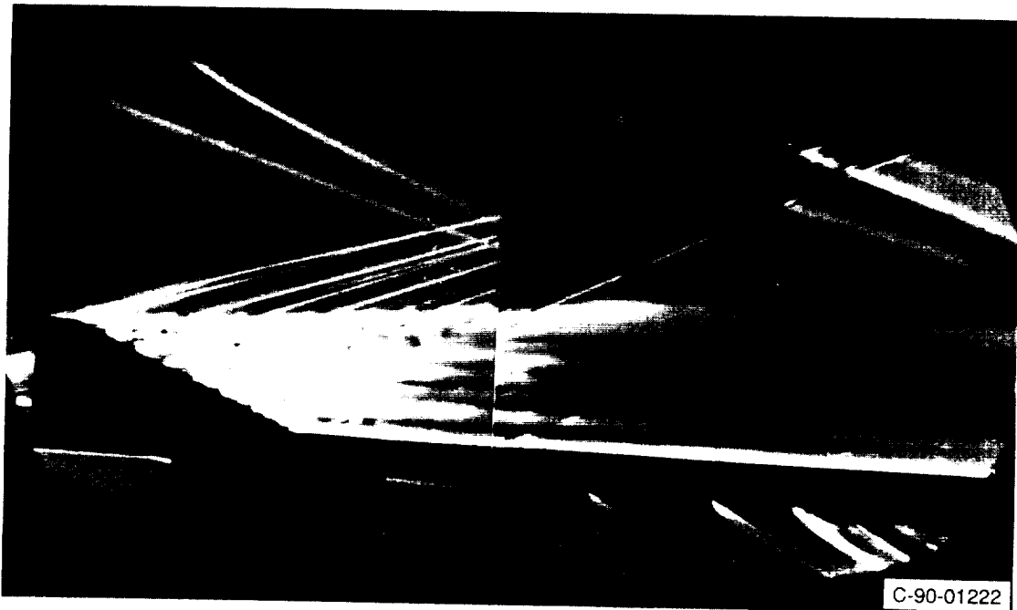
Figure 8.—Composite schlieren photograph of isolated honeycomb boundary layer simulator in two positions at Mach 4.0.
