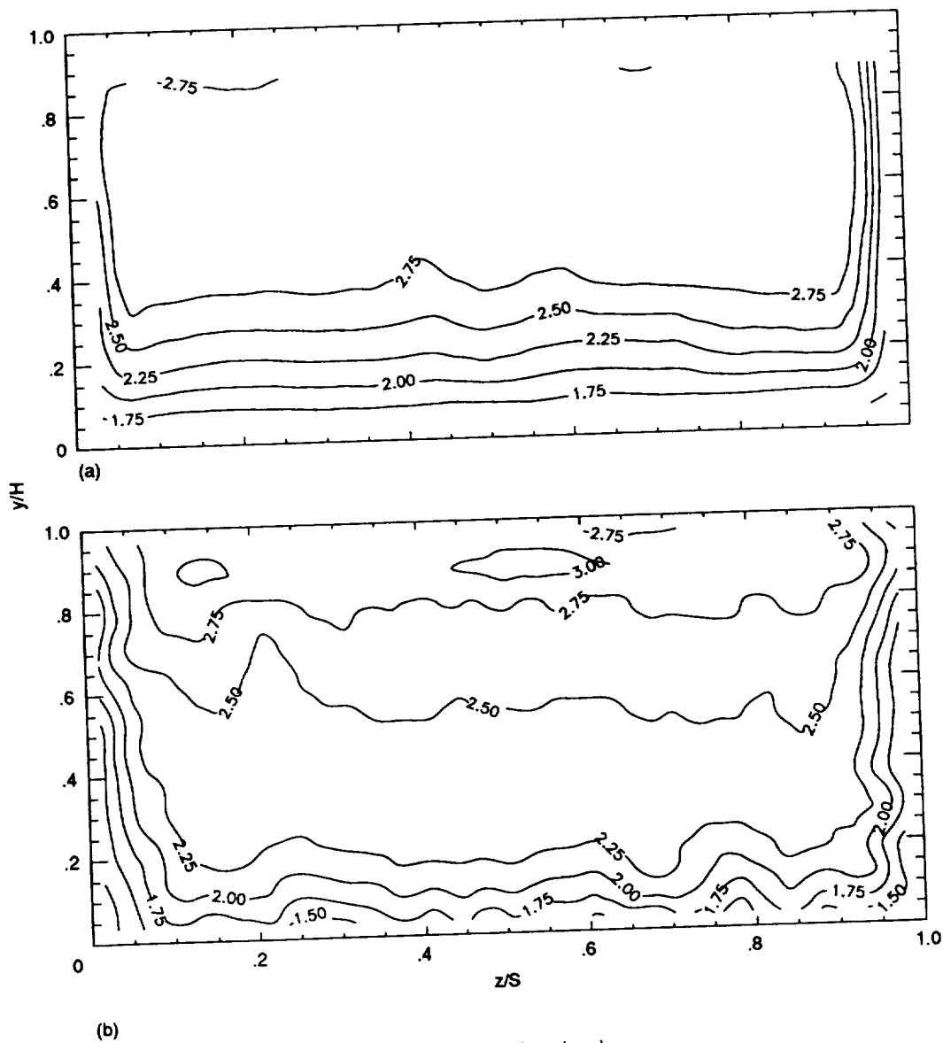
Figure 22.—Cross-plane Mach number contours for Lewis channel flow model at Mach 3.0 with cowl angle of 0^\circ (cowl exit survey).
