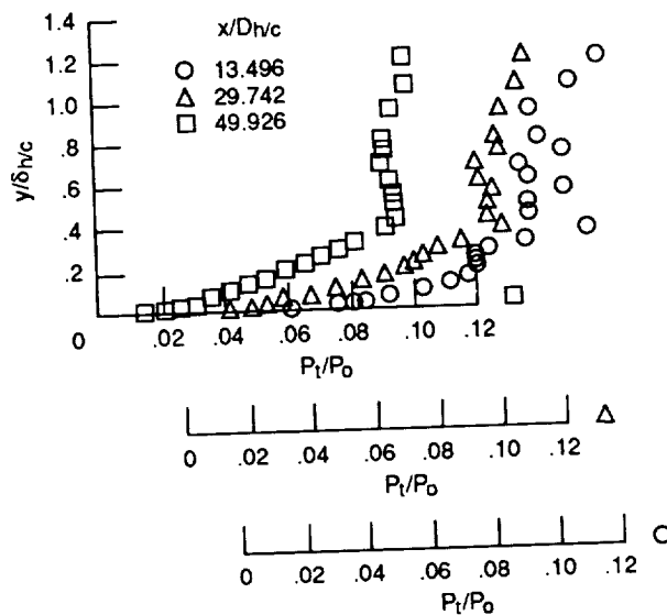
Figure 15.—Centerline streamwise pitot pressure profiles of isolated boundary layer simulator model at Mach 4.0 ( \delta_{h/c} = 4.06 cm).
