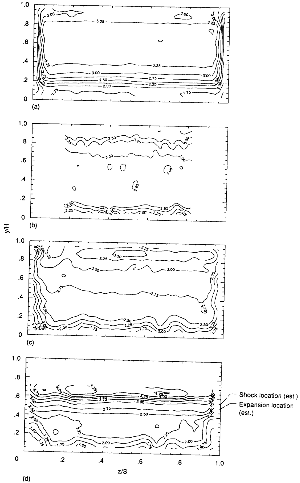
(a) 0° Cowl angle, naturally occurring boundary layer (cowl exit survey). (b) 0° Cowl angle, simulated boundary layer (cowl entrance survey).
