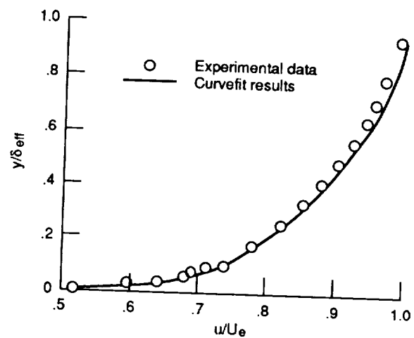
Figure 18.—Simulated boundary layer wall-wake curvefit results at Mach 4.0 ( x/D_{h/c} = 50 ).
