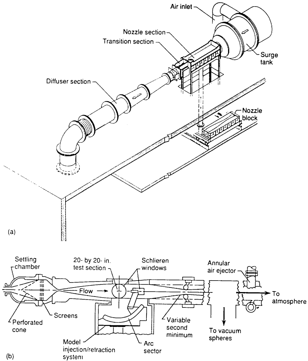
(a) NASA Lewis 1- by 1-Foot Supersonic Wind Tunnel. (b) NASA Langley 20 Inch-Mach 6 Hypersonic Wind Tunnel.
