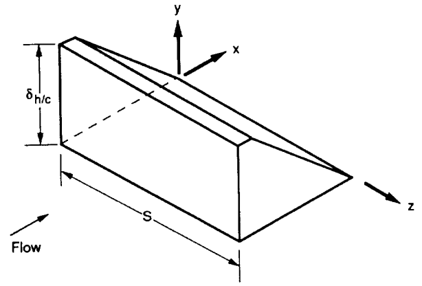
Figure 2.—Model coordinate system.
