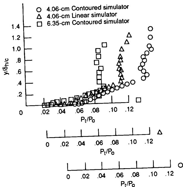
Figure 16.—Centerline pitot profiles of isolated boundary layer simulator model at Mach 4.0 ( x/D_{h/c} = 46 ).
