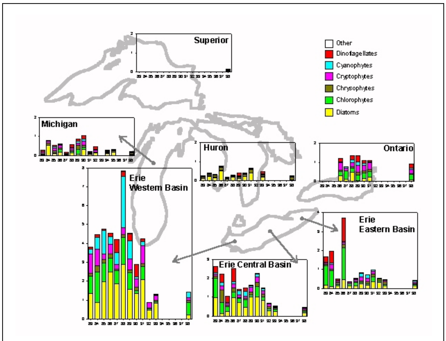
Figure 1. Trends in phytoplankton biovolume ( \text{gm}/\text{m}^3 ) and community composition in the Great Lakes 1983-1998 (Summer, Open Lake, Epilimnion) (Blank indicates no data).
