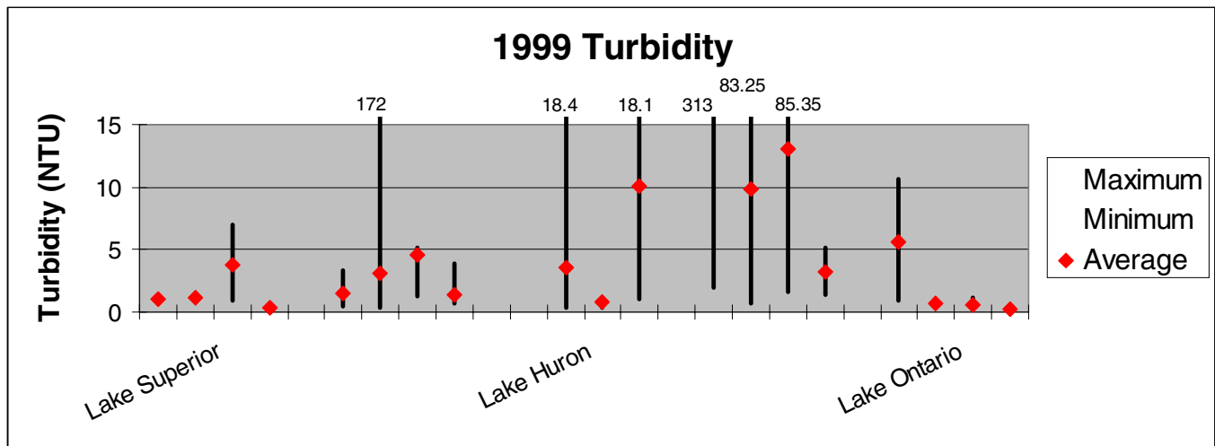
Figure 3. This graph represents the fluctuations that occur in raw water turbidity in the course of a single year. Values are based on monthly averages. Due to this, the graph is representative of possible fluctuation ranges but not conclusive of the exact turbidity for 1999.
