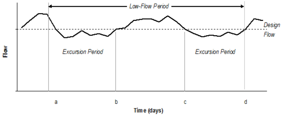
Figure 3-1: Illustration of biologically-based design flow
