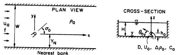
Figure 8-6. Schematics of single port discharge geometry in ambient channel with rectangular cross-section (width W may be finite or unlimited).
