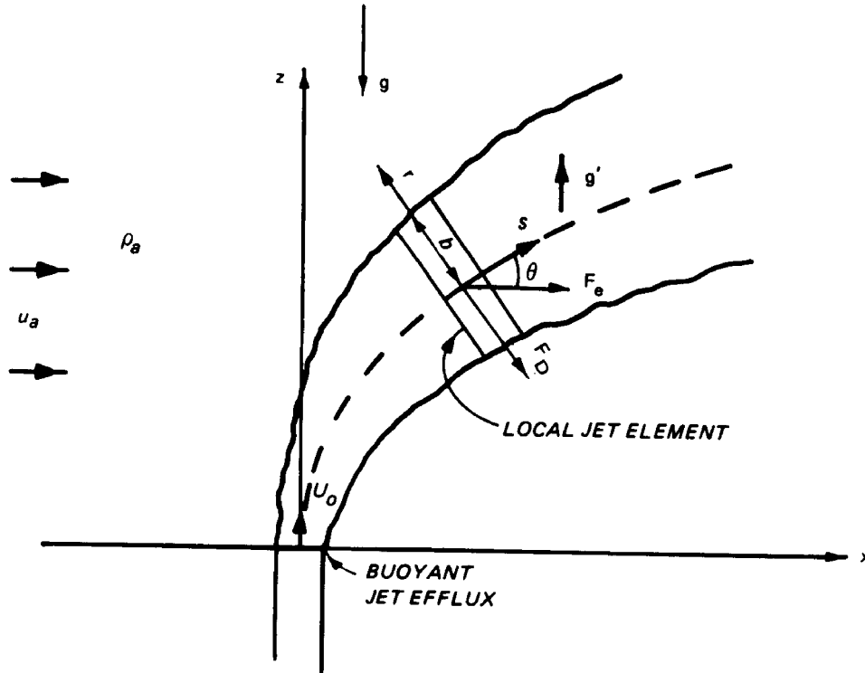
Figure 8-9. Round buoyant jet in ambient crossflow with drag and entrainment forces (Example: vertical discharge).
