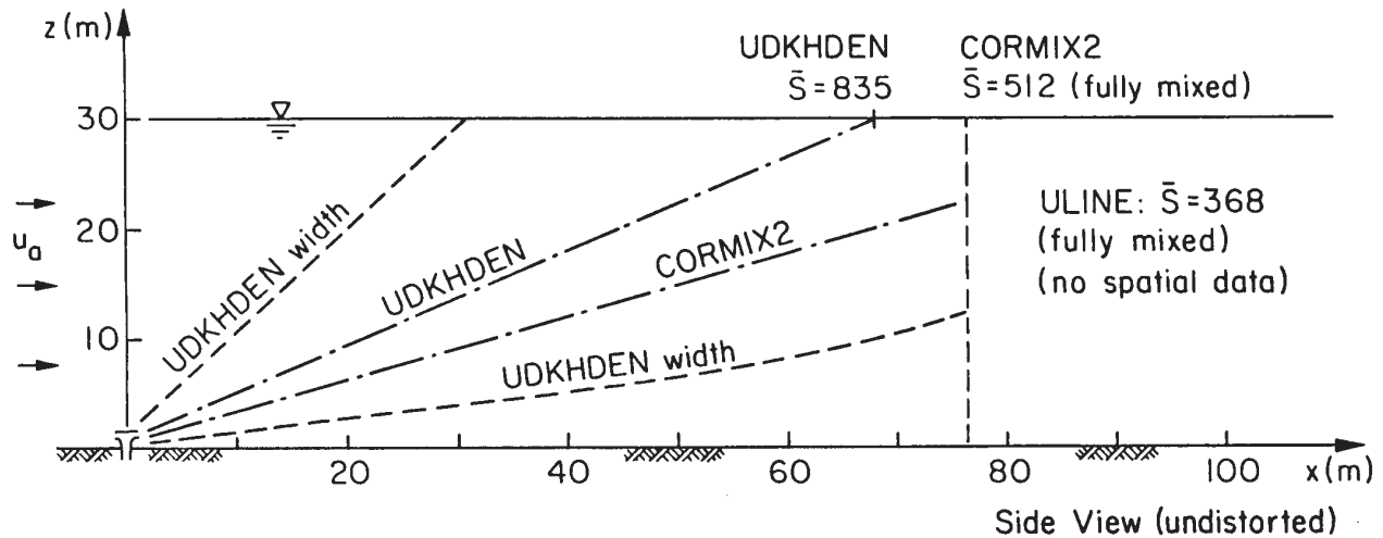
Figure 9-10. Case BB2: multipoint diffuser discharge in uniform ambient; comparison of jet integral models and CORMIX2.
