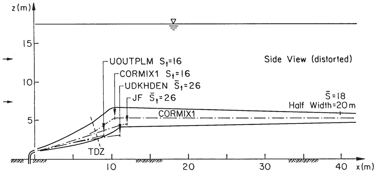
Figure 9-6. Case AA3: single port discharge (modified design) in stratified summer conditions; comparison of jet integral models and CORMIX1.
