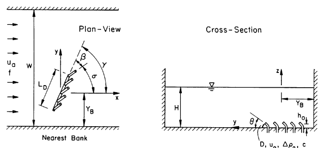
Figure 8-7. Schematics of multiport diffuser geometry in ambient channel with rectangular cross-section (width W may be finite or unlimited).
