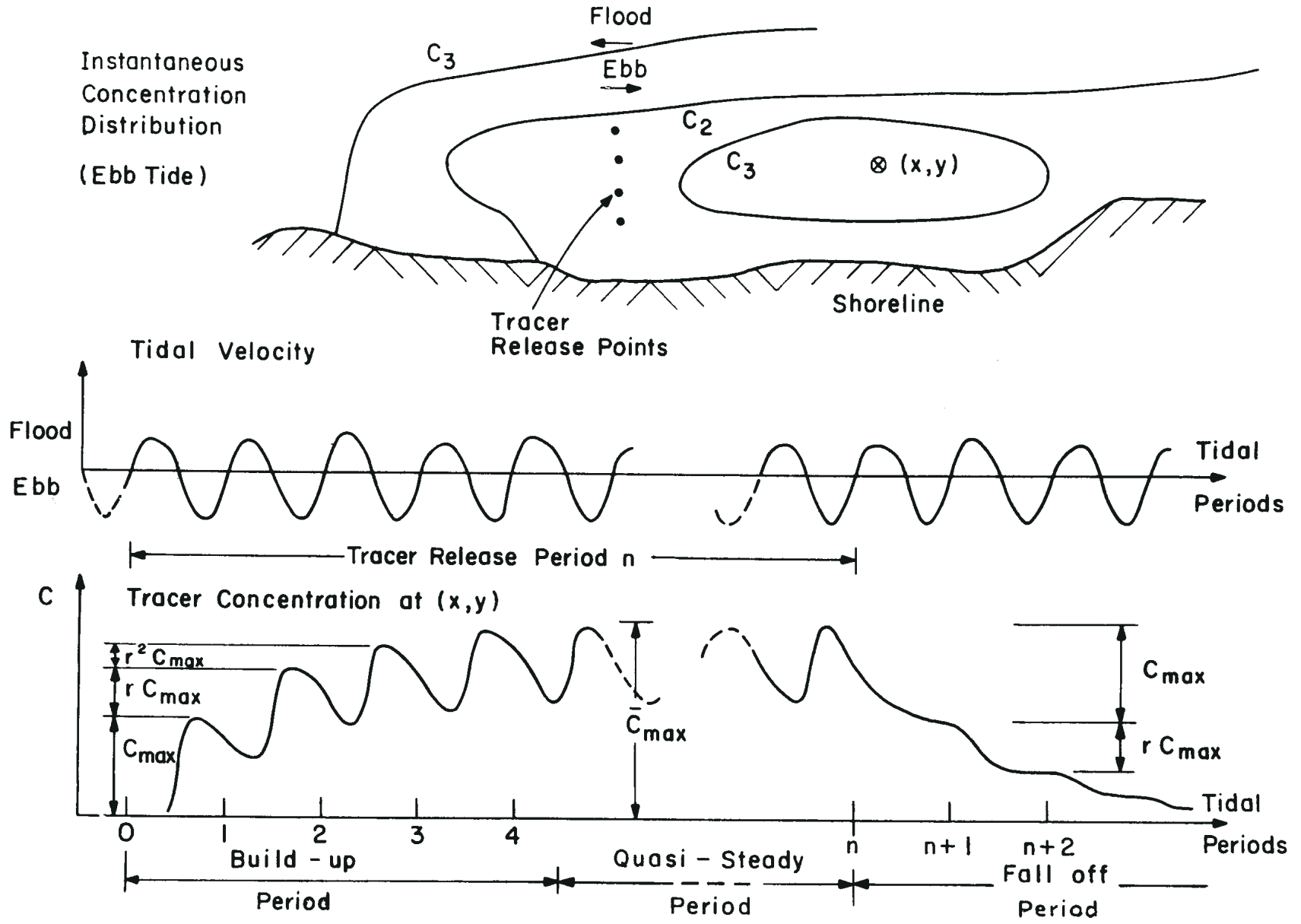
Figure 8-19. Schematics of a field tracer dispersion test in a periodically reversing tidal system.
