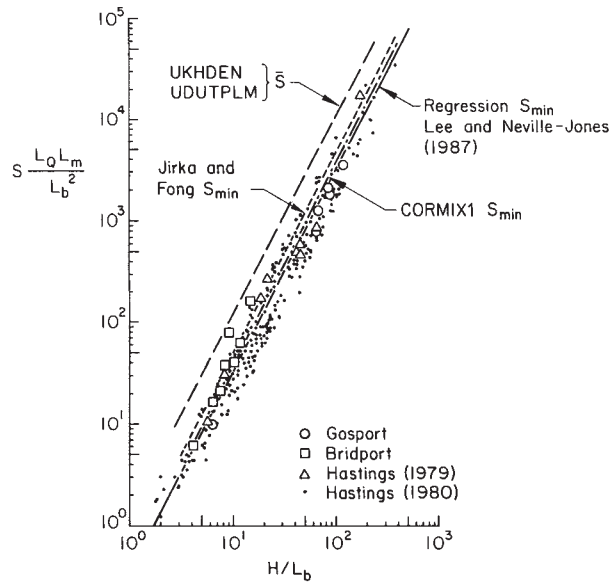
Figure 9-4. Comparison of observed minimum surface dilution for three submerged single port outfalls (Lee and Neville-Jones, 1987) with predictions of jet integral models and CORMIX1.
