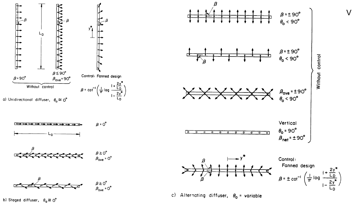
Figure 8-8. Schematic plan views of three major diffuser types: a) Unidirectional diffuser, b) Staged Diffuser, c) Alternating diffuser. Any of those diffusers may have a variable alignment \gamma relative to the ambient current.
