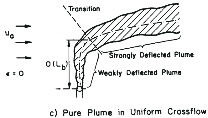
Figure 8-11. Length scales measuring the effects of momentum flux, buoyancy flux, crossflow and stratification of submerged jet behavior.
