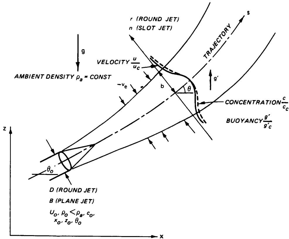
Figure 8-1. Buoyant jet with round or slot geometry in stagnant uniform-density environment.
