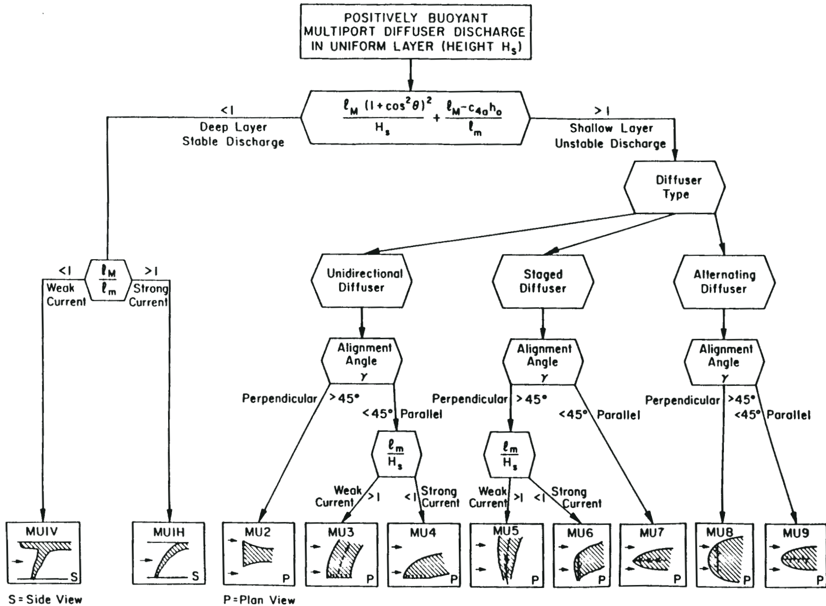
Figure 8-17. CORMIX2 sub-classification: flow classes for positively buoyant multipoint discharges in uniform ambient layer.
