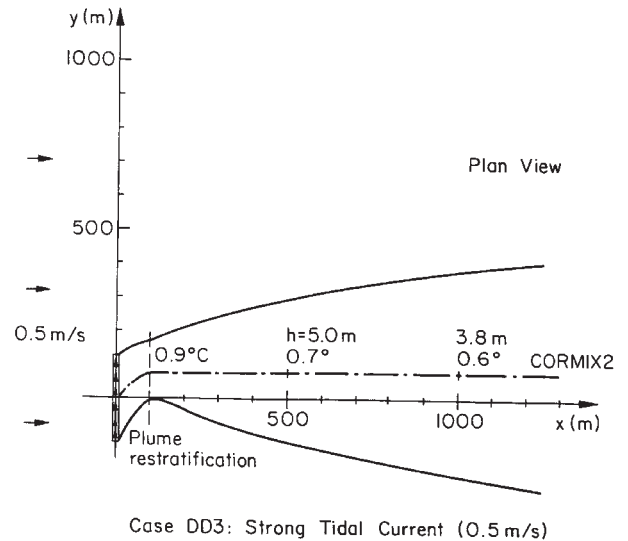
Figure 9-15. Case DD3: staged multiport diffuser for cooling water discharge; CORMIX2 predictions for strong tidal current.
