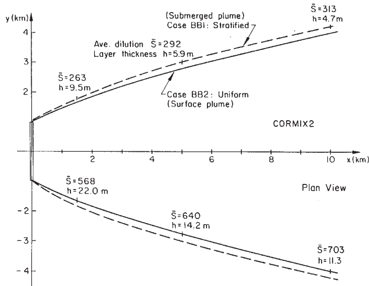
Figure 9-9. Cases BB1 and BB2: predicted (CORMIX2) far-field behavior for multiport diffuser plume in stratified and uniform conditions.
