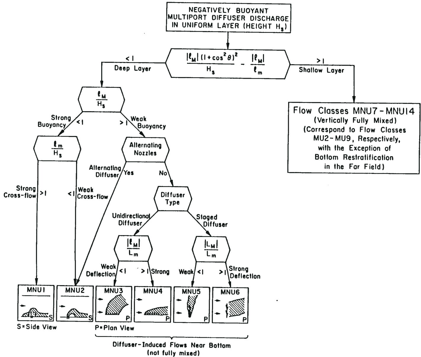
Figure 8-18. CORMIX2 sub-classification: flow classes for negatively buoyant multipoint discharges in uniform ambient layer.
