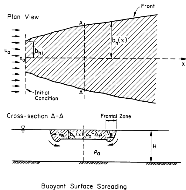
Figure 8-4. Buoyant spreading processes in the far-field (Example: surface spreading).
