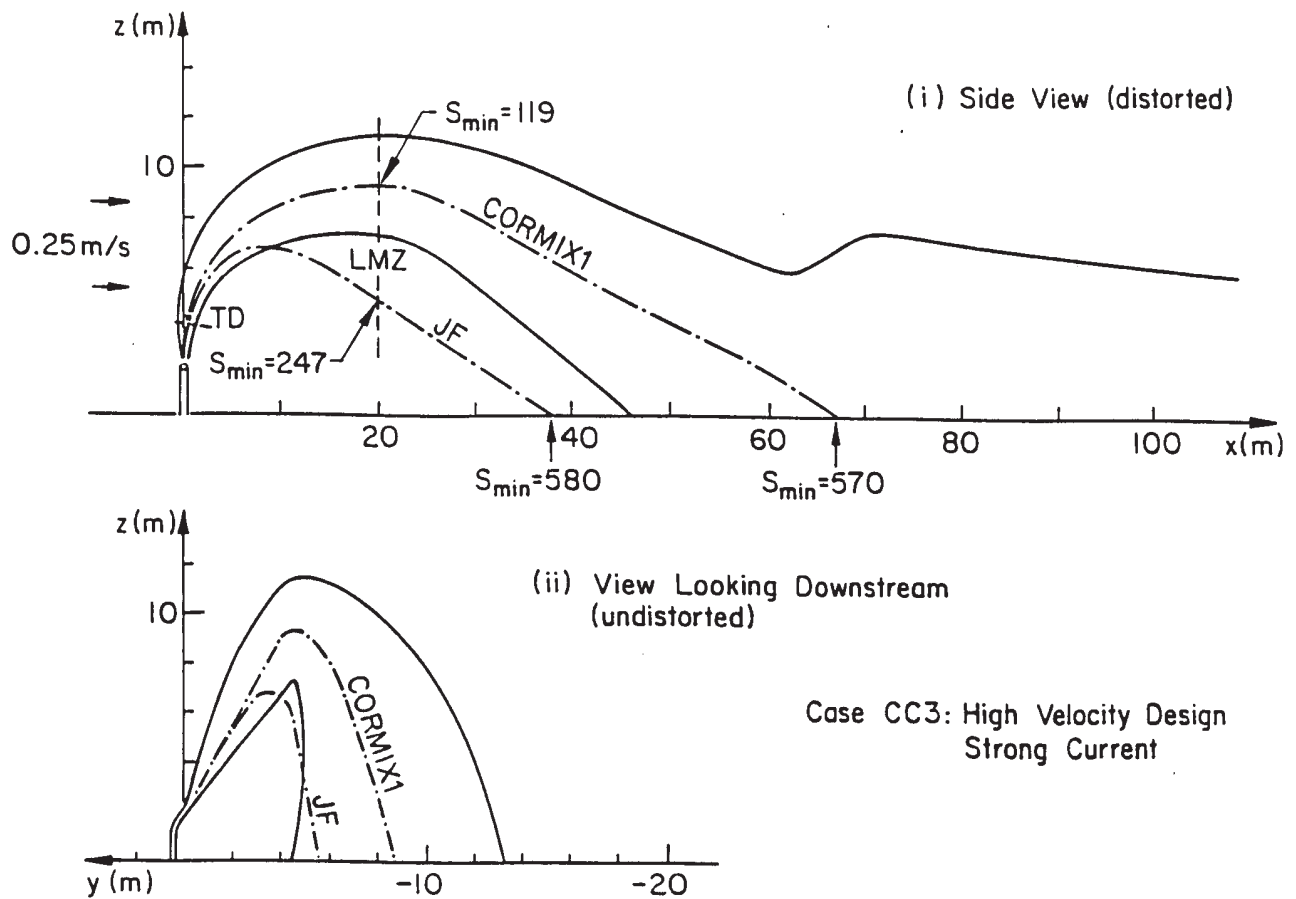
Figure 9-12. Case CC3: negatively buoyant discharge from single port; high exit velocity design with strong ambient current.
