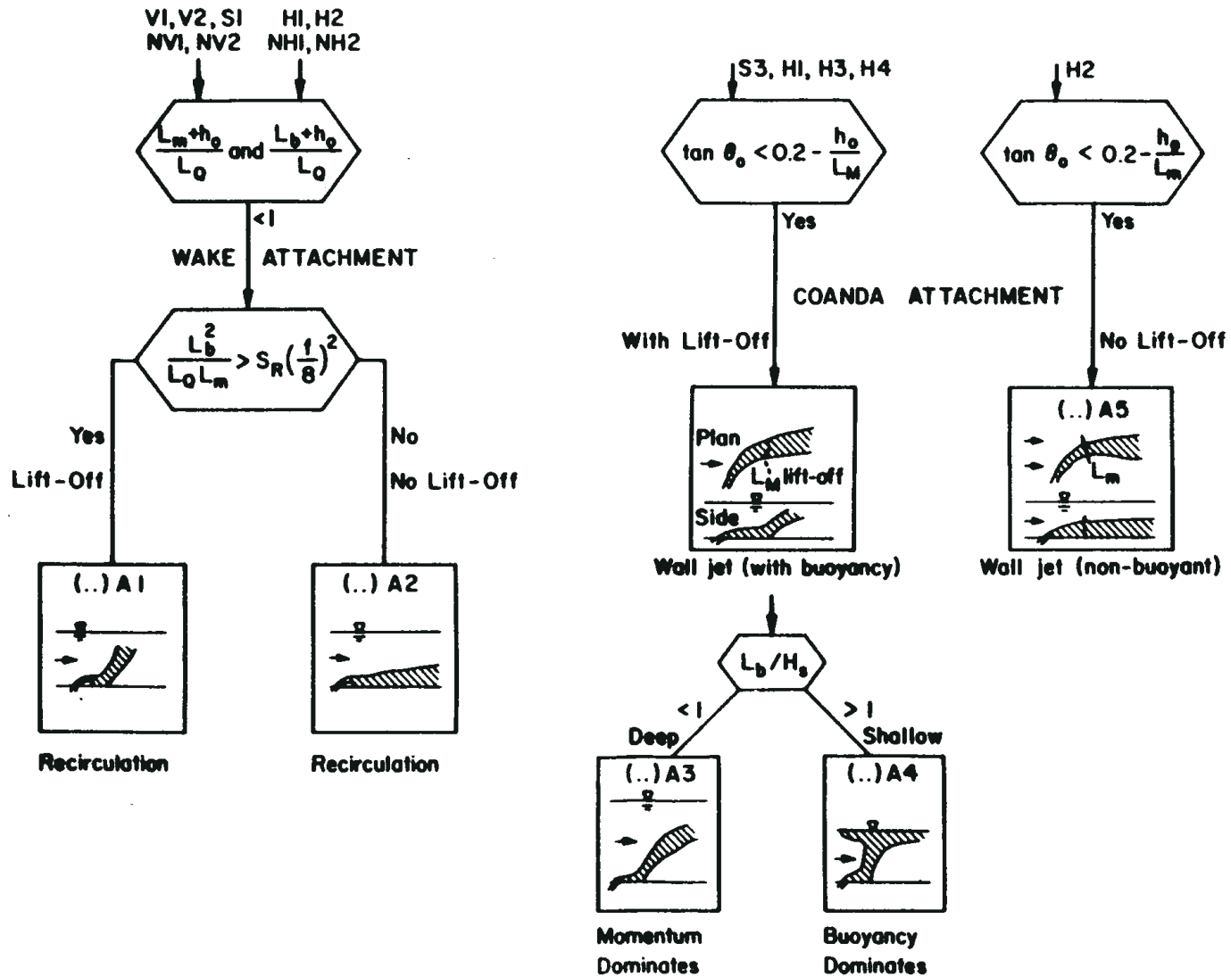
Figure 8-15. CORMIX1 sub-classification: assessment of dynamic bottom attachment processes and flow classes for bottom-attached flows.
