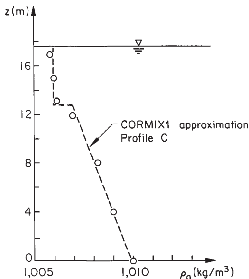
Figure 9-1. Design case AA: vertical ambient density profile in typical summer conditions.
