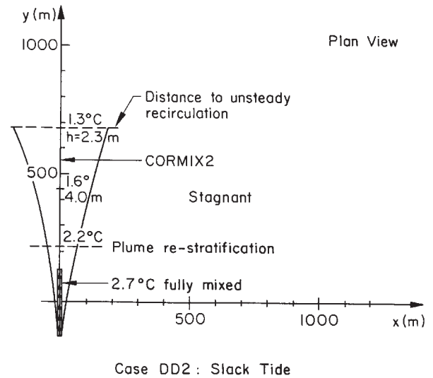
Figure 9-14. Case DD2: staged multiport diffuser for cooling water discharge; CORMIX2 predictions for slack tidal conditions.
