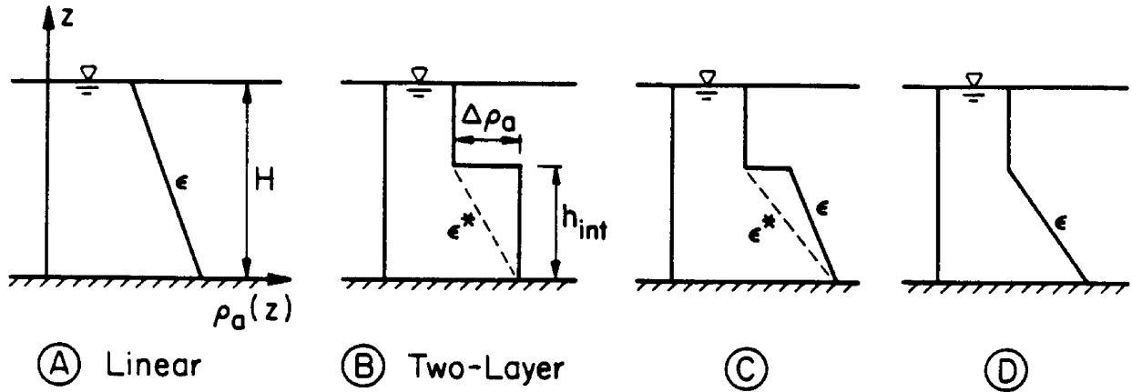
Figure 8-10. Schematic ambient density profiles for use in expert system CORMIX.
