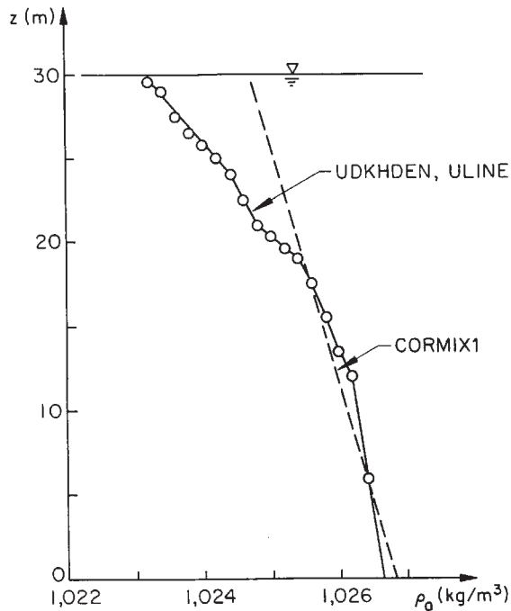
Figure 9-7. Design case BB: vertical ambient density profile for design conditions.
