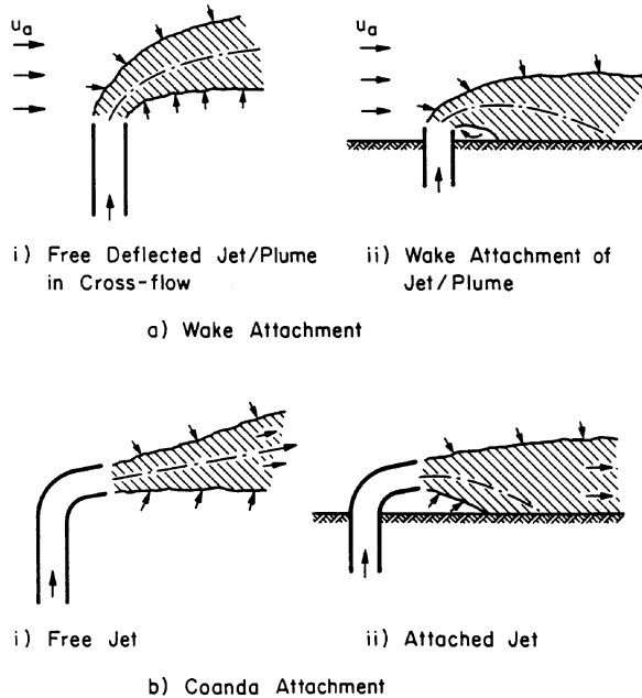
Figure 8-3. Bottom attachment processes for submerged discharges.
