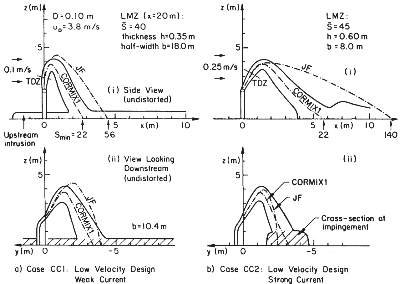
Figure 9-11. Cases CC1 and CC2: negatively buoyant discharge from single port; low exit velocity design under a) weak and b) stronger ambient current.
