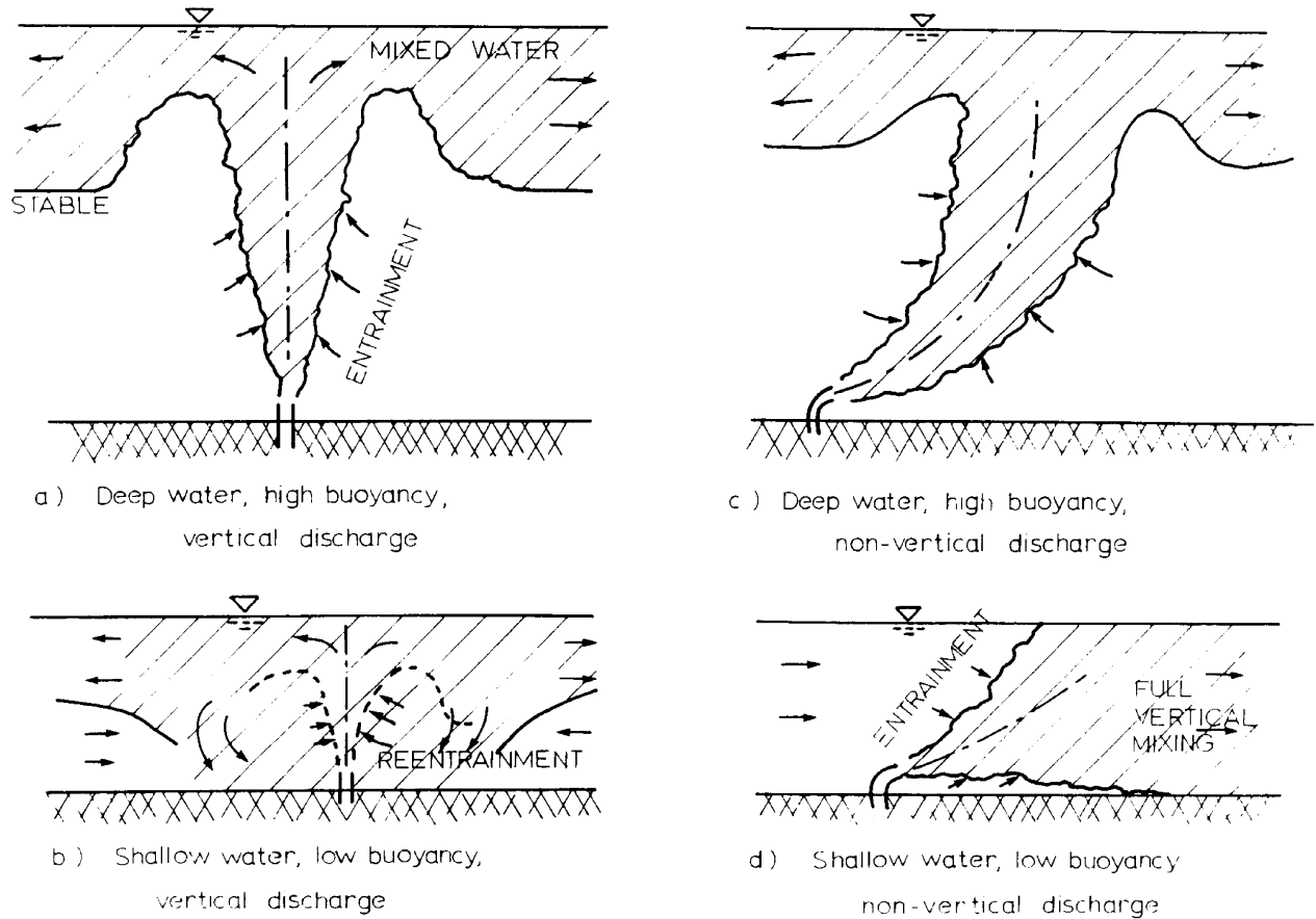
Figure 8-2. Stable or unstable near-field flows produced by submerged buoyant discharges.
