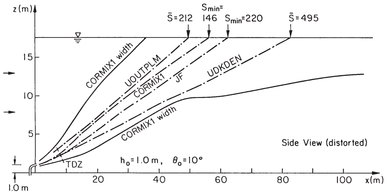
Figure 9-3. Case AA2: single port discharge (modified design) in unstratified winter conditions; comparison of jet integral models and CORMIX1.
