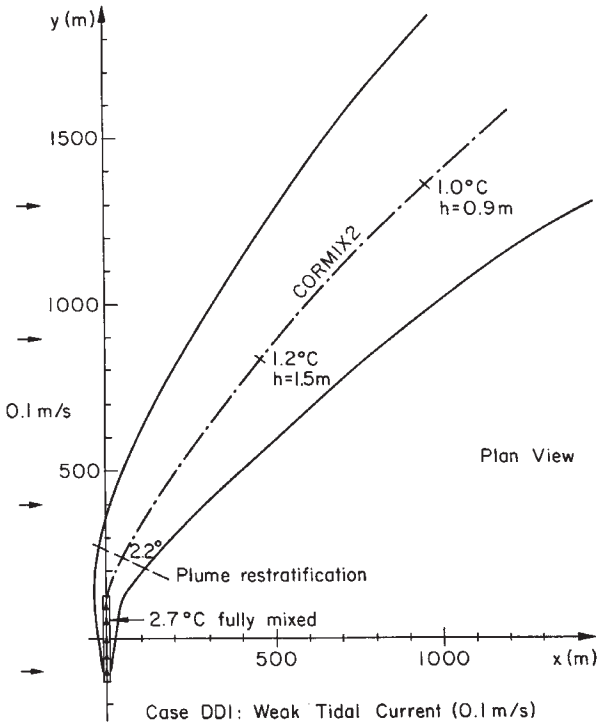
Figure 9-13. Case DD1: staged multiport diffuser for cooling water discharge; CORMIX2 predictions for weak tidal current.
