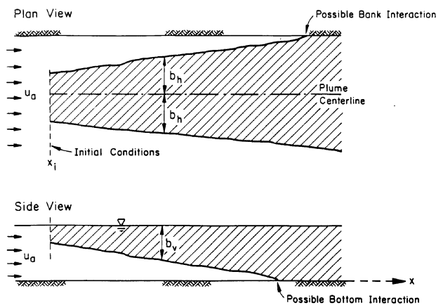
Figure 8-5. Passive ambient diffusion processes.
