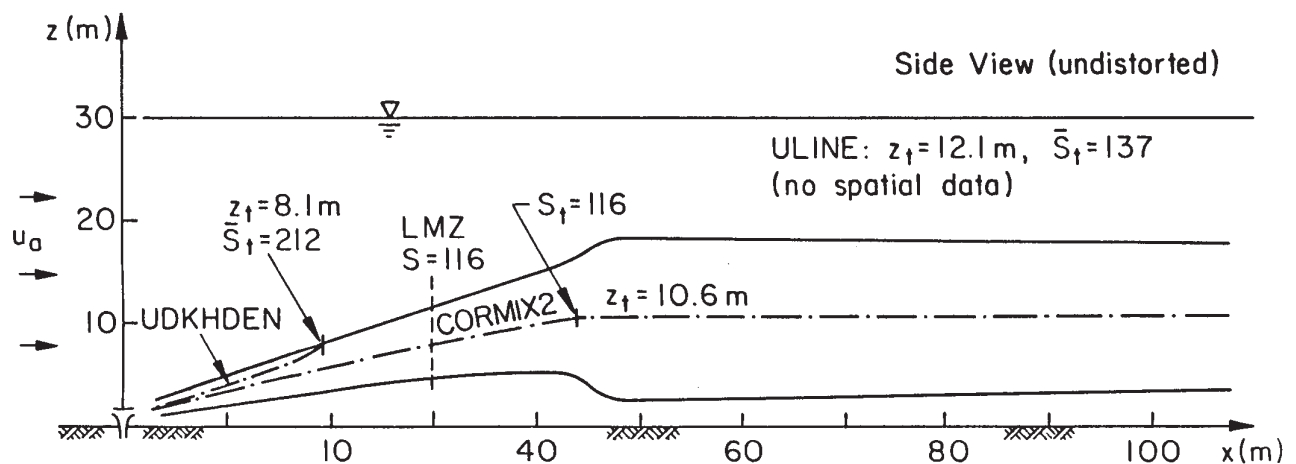
Figure 9-8. Case BB1: multiport diffuser discharge under stratified conditions; comparison of jet integral models and CORMIX2.
