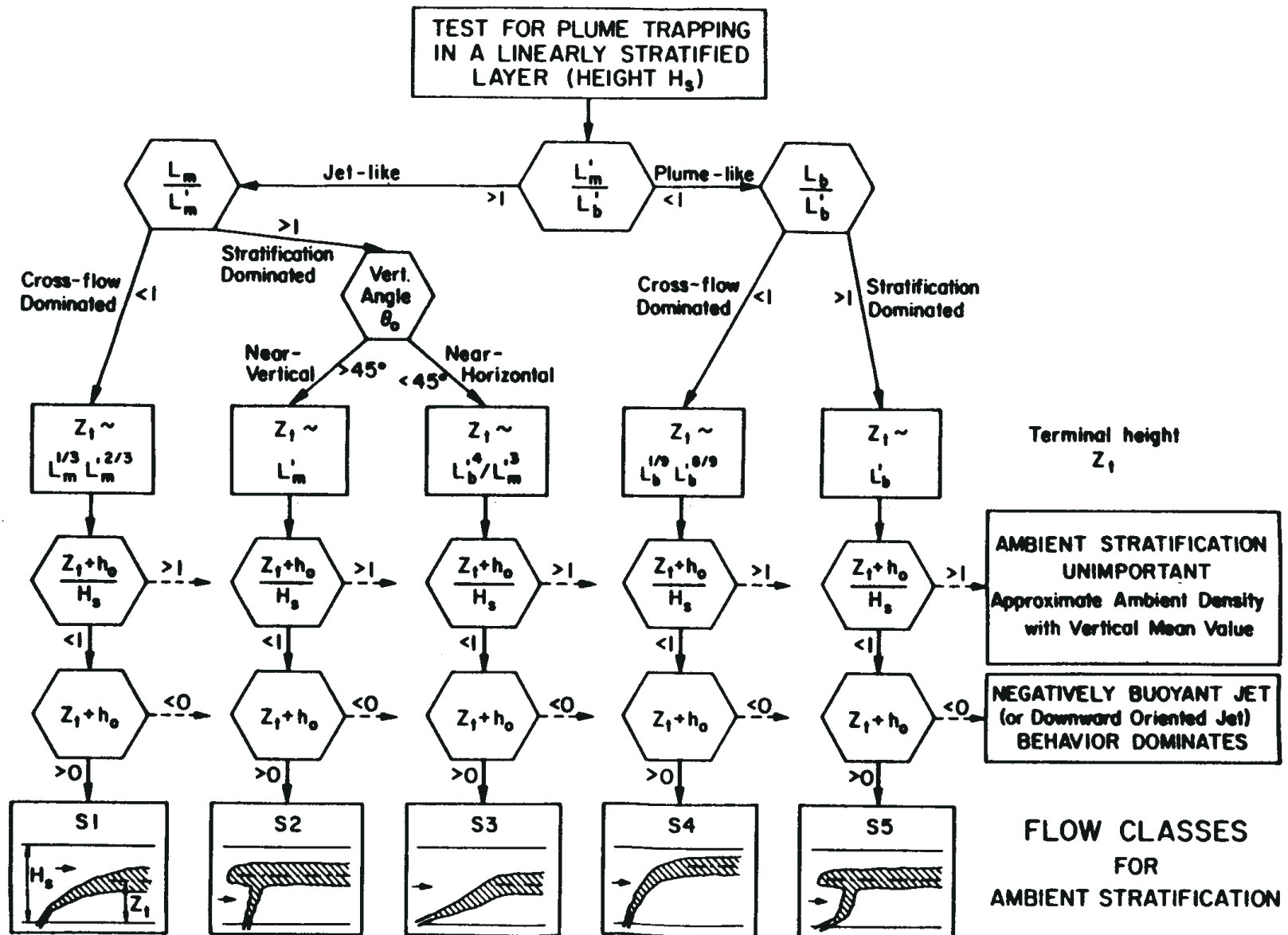
Figure 8-11. Length scales measuring the effects of momentum flux, buoyancy flux, crossflow and stratification of submerged jet behavior.
