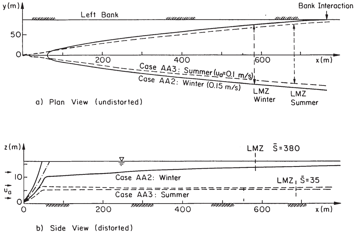
Figure 9-5. Cases AA2 and AA3: predicted (CORMIX1) far-field behavior for single port discharge (modified design) in winter and summer conditions.
