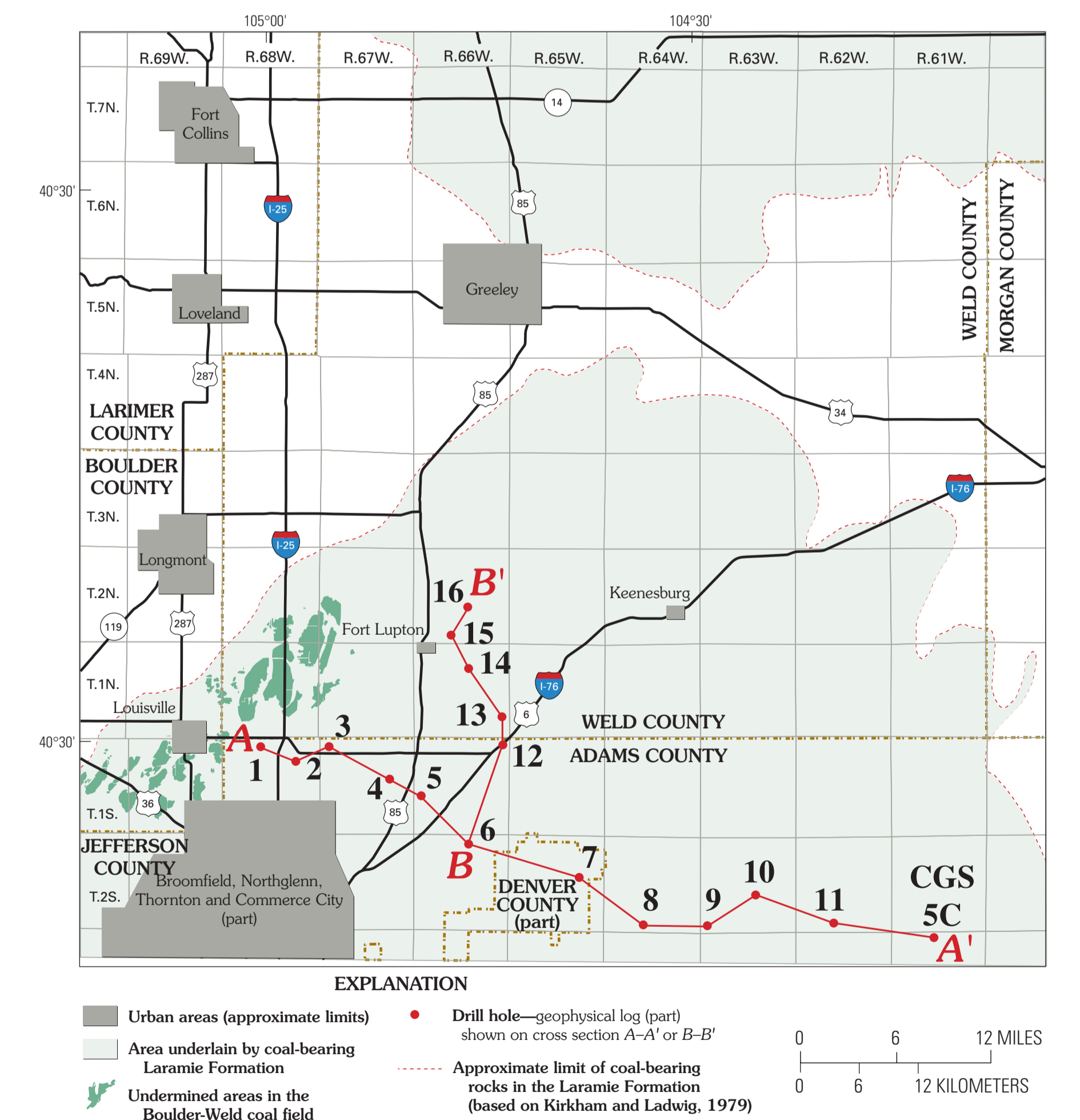
Drill-hole and cross-section locations
