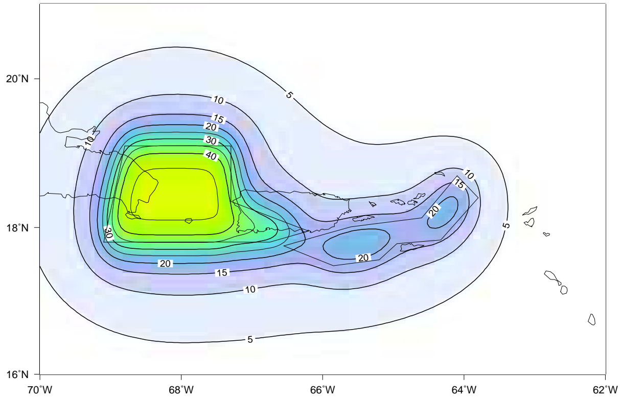
Fig.3e: PGA (%g) with 2% probability of exceedance in 50 years from Anegada and Mona extensional zones.
