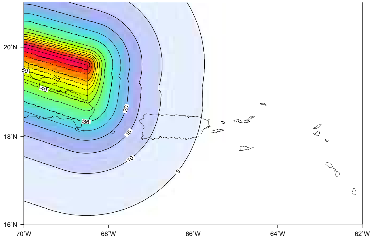
Fig.3d: PGA (%g) with 2% probability of exceedance in 50 years from Hispaniola subduction.
