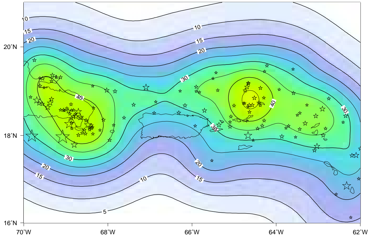
Fig.3b: PGA (%g) with 2% probability of exceedance in 50 years from deep seismicity ( d \geq 50 km).
