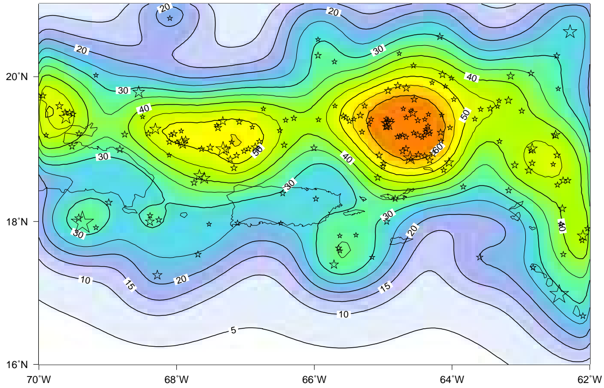
Fig.3a: PGA (%g) with 2% probability of exceedance in 50 years from shallow seismicity ( d < 50 km).
