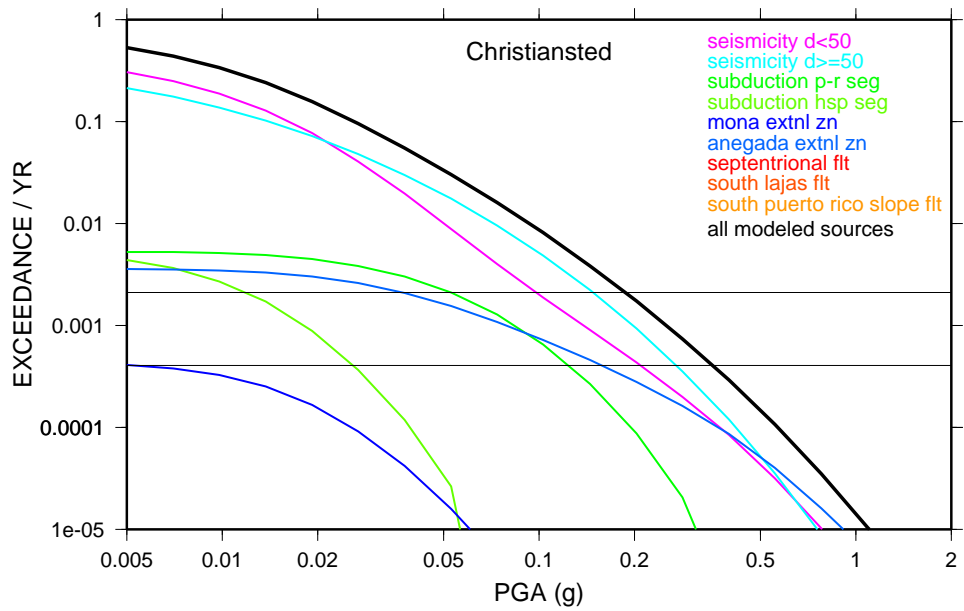
Fig.13e: PGA hazard curves for Christiansted.
