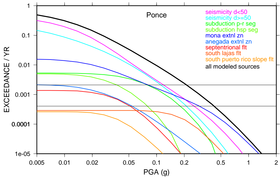
Fig.13c: PGA hazard curves for Ponce.
